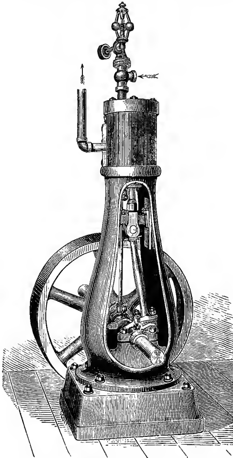
FIG. 93.—Vertical Stationary Steam-Engine.
