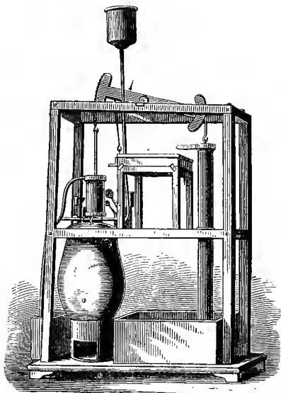
FIG. 24.—The Newcomen Model.
