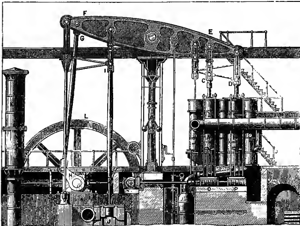
FIG. 105.—Double-Cylinder Pumping-Engine, 1878.
