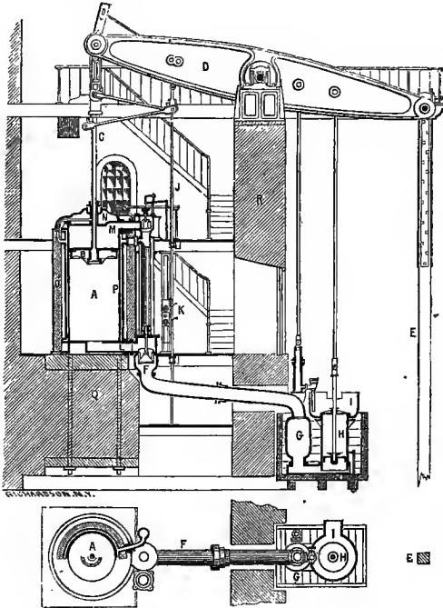
FIG. 101.—Cornish Pumping-Engine, 1878. Section.
