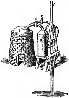
FIG. 11.—Savery's Model, 1698.
