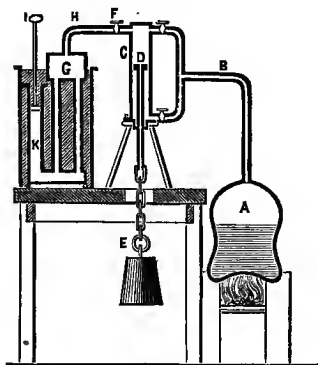
FIG. 25.—Watt's Experiment.
