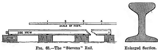
FIG. 68.—The "Stevens" Rail.
