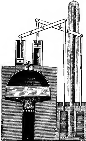
FIG. 41.—Leupold's Engine, 1720.
