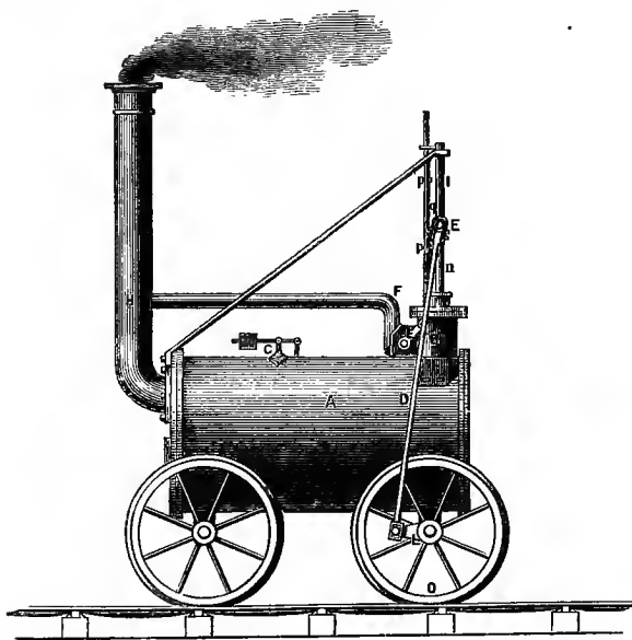
FIG. 50.—Trevithick's Locomotive, 1804.
