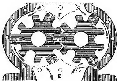
FIG. 124.—Rotary Pump.
