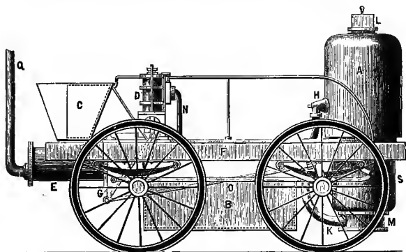
FIG. 54.—The "Novelty," 1829.
