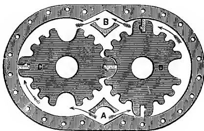
FIG. 123.—Rotary Steam-Engine.
