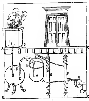
Fig. 1.—Opening Temple-Doors by Steam, B. C. 200.
