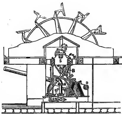
FIG. 181.—Oscillating Engine and Feathering Paddle-Wheel.
