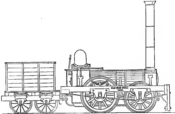
FIG. 64.—"Old Ironsides," 1832.
