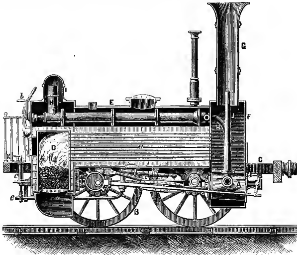
FIG. 57.—Stephenson's Locomotive, 1825.
