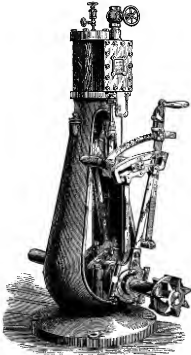
FIG. 135.—Launch-Engine.
