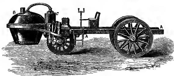
FIG. 44.—Cugnot's Steam-Carriage, 1770.
