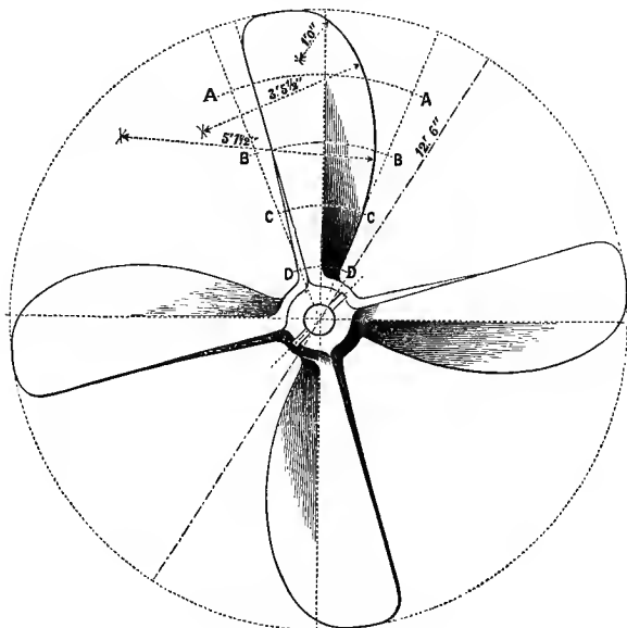
FIG. 139.—Screw-Propeller.
