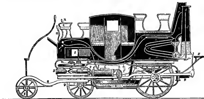
FIG. 48.—Gurney's Steam-Carriage.
