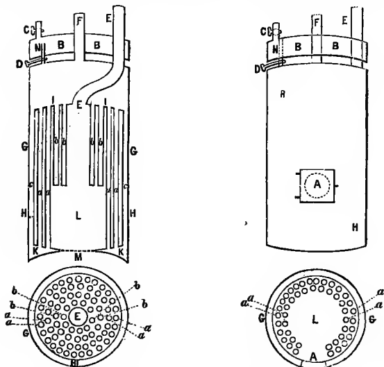
FIG. 73.—Read's Boiler in Section, 1788.
