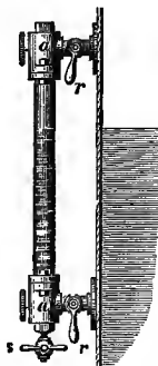
Glass Water-Gauge.
