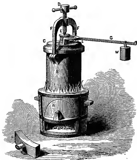
FIG. 16.—Papin's Digester, 1680.
