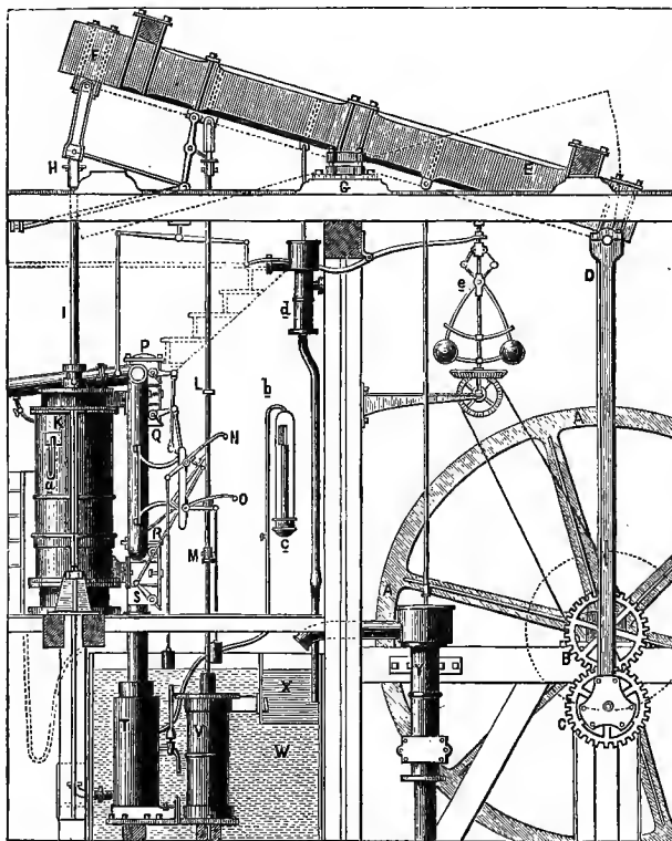
FIG. 27.—Watt's Engine, 1781.
