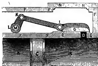
FIG. 100.—The Greene Engine.
