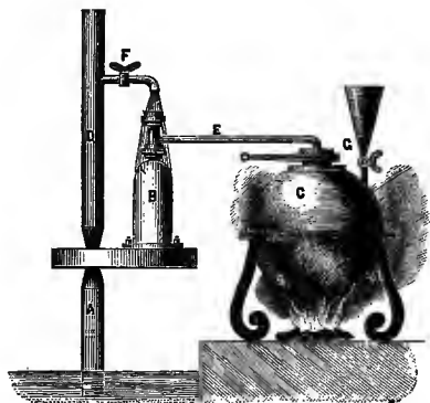
FIG. 12.—Savery's Engine, 1698.
