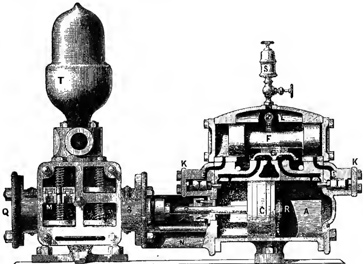
FIG. 102.—Steam-Pump.
