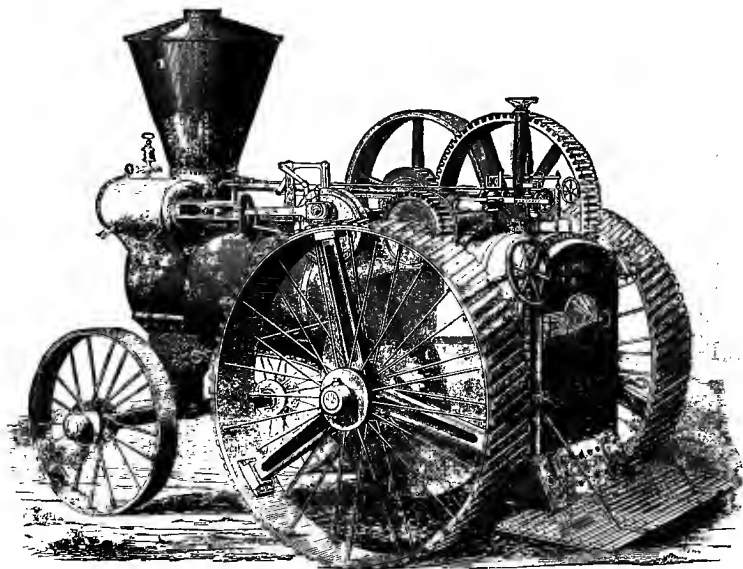
FIG. 117.—The Thrashers' Road-Engine, 1878.
