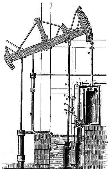
FIG. 26.—Watt's Engine, 1774.
