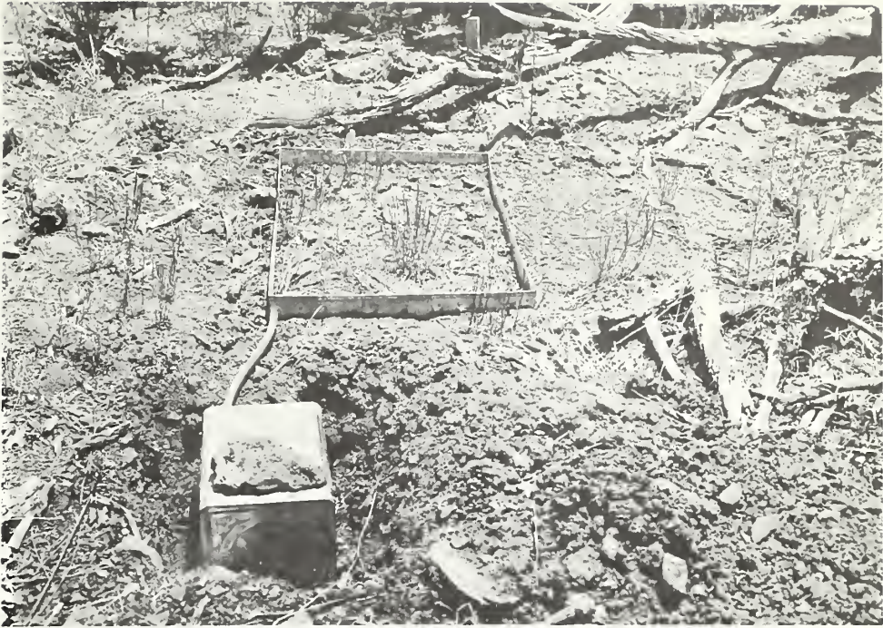
Figure 14. --A plot used for measuring surface runoff in the Utah juniper type. The 2- by 3-foot plot frame is hammered a few inches into the ground. Surface runoff flows into a trough at the lower end of the plot and is carried through a hose into the collection tank where it is weighed. Weight of water is converted to inches of surface runoff.
