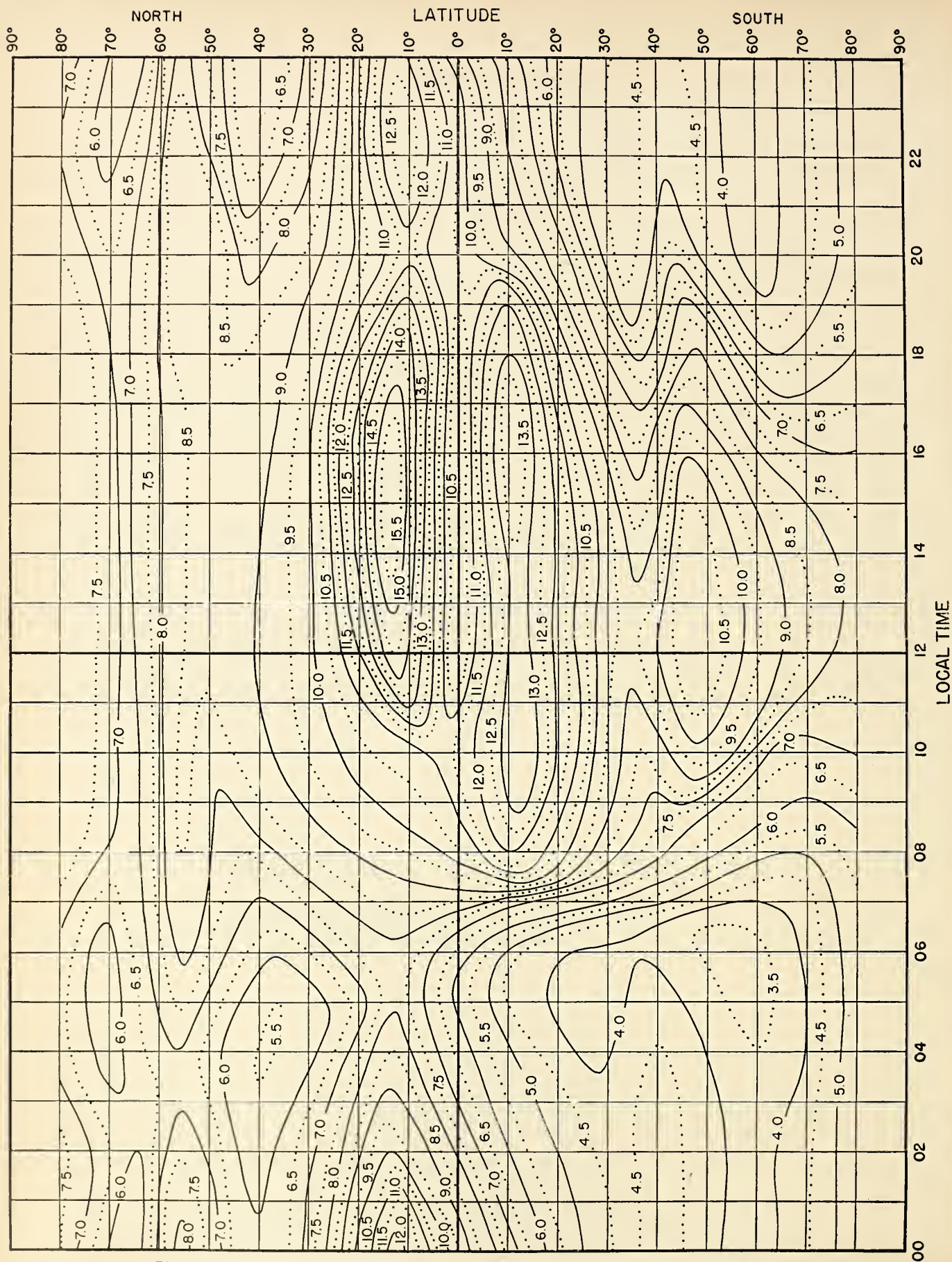
Fig. 7. F 2 ZERO-MUF, IN Mc, I ZONE, PREDICTED FOR JULY 1947
