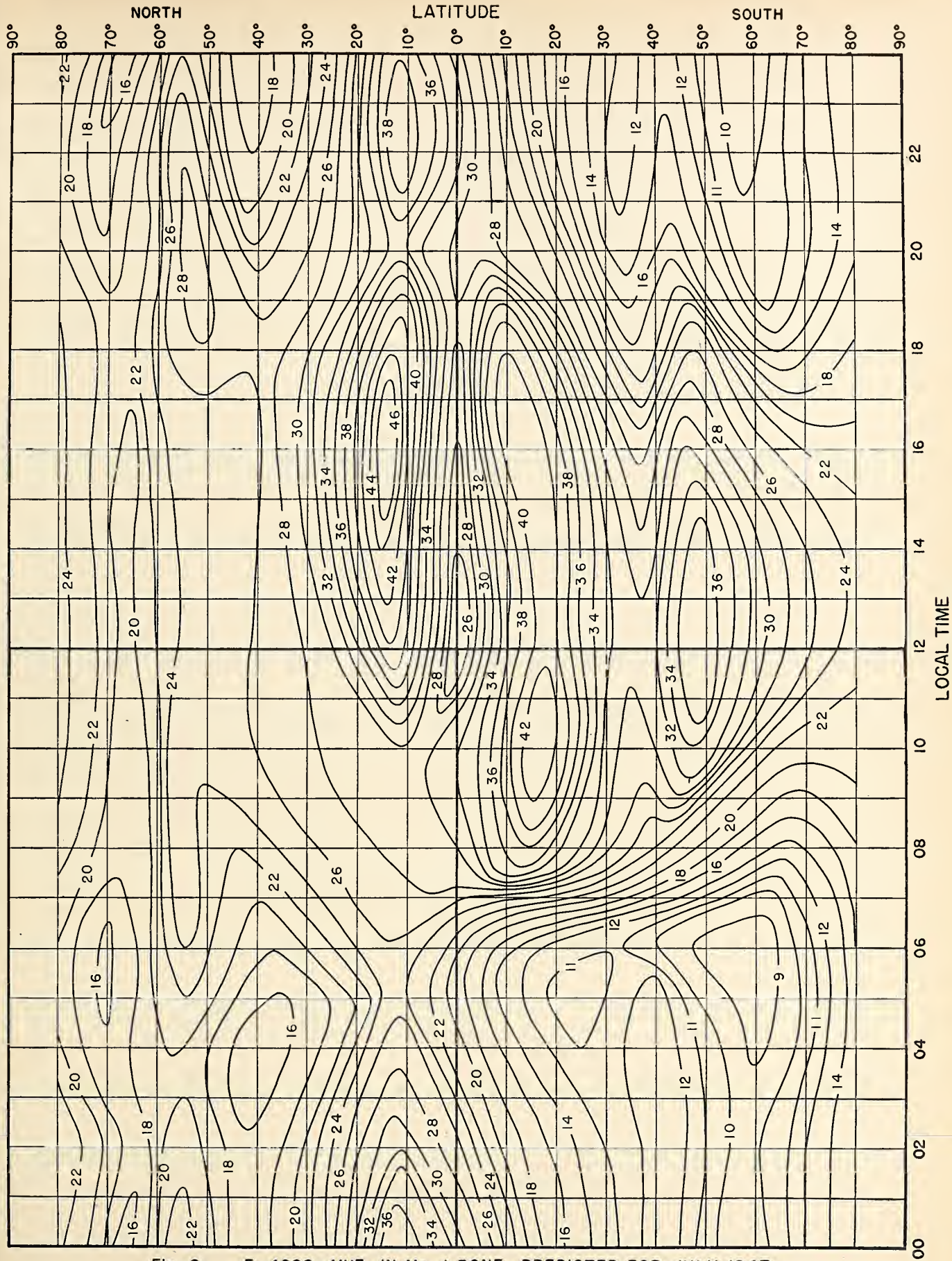
Fig. 8. F 2 4000-MUF, IN Mc, I ZONE, PREDICTED FOR JULY 1947
