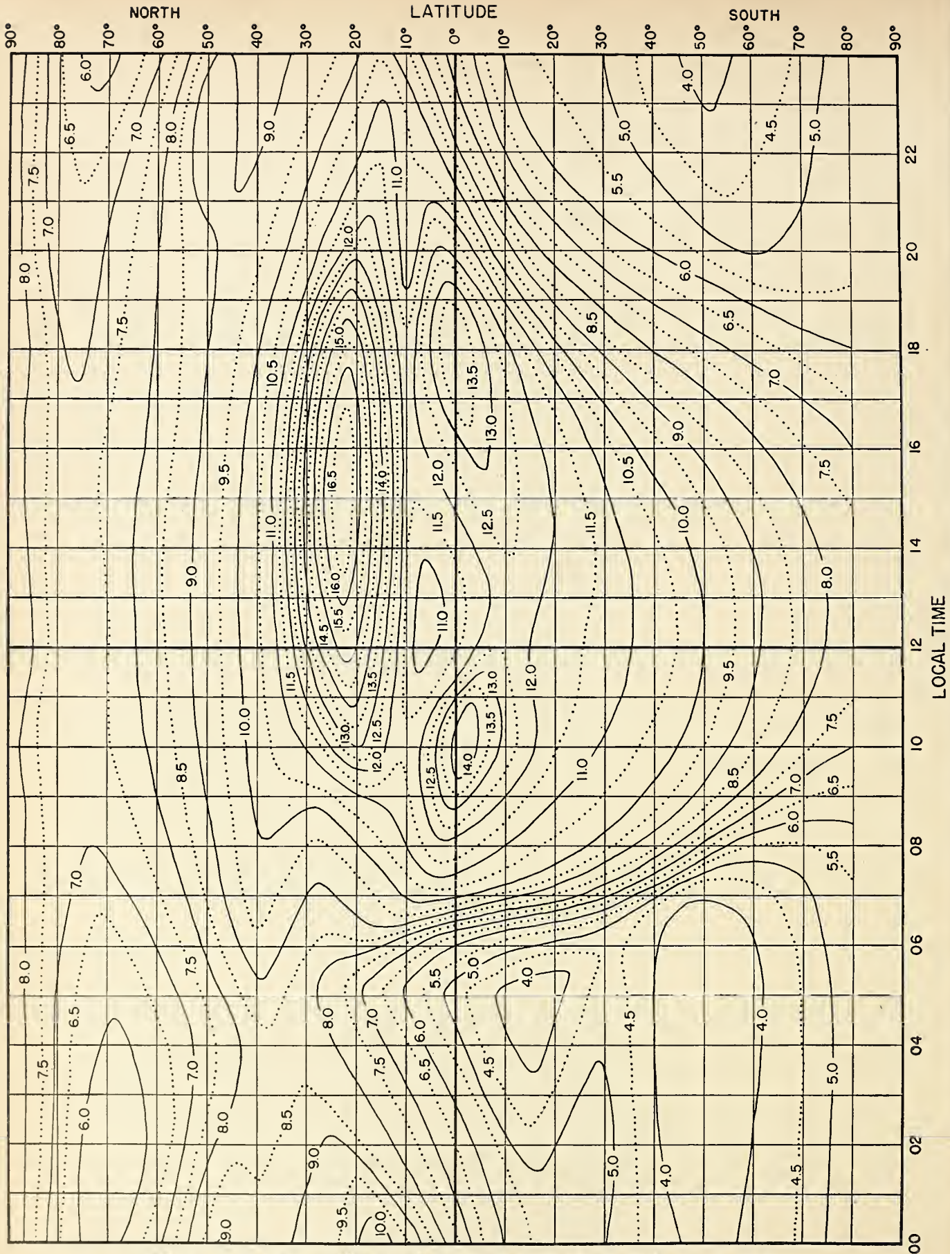
Fig. 9. F_2 ZERO-MUF, IN Mc, E ZONE, PREDICTED FOR JULY 1947
