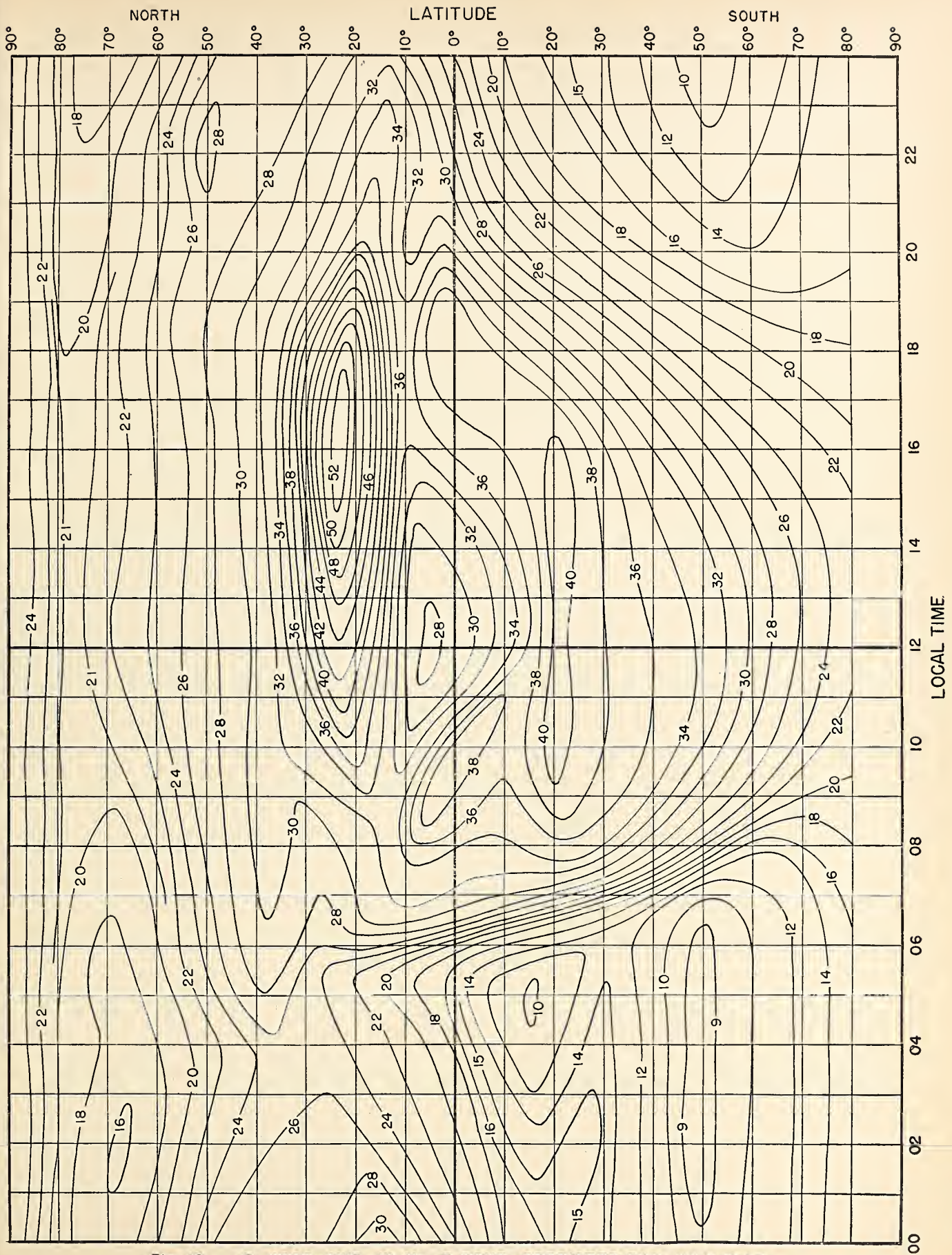
Fig. 10. F_2 4000-MUF, IN Mc, E ZONE, PREDICTED FOR JULY 1947
