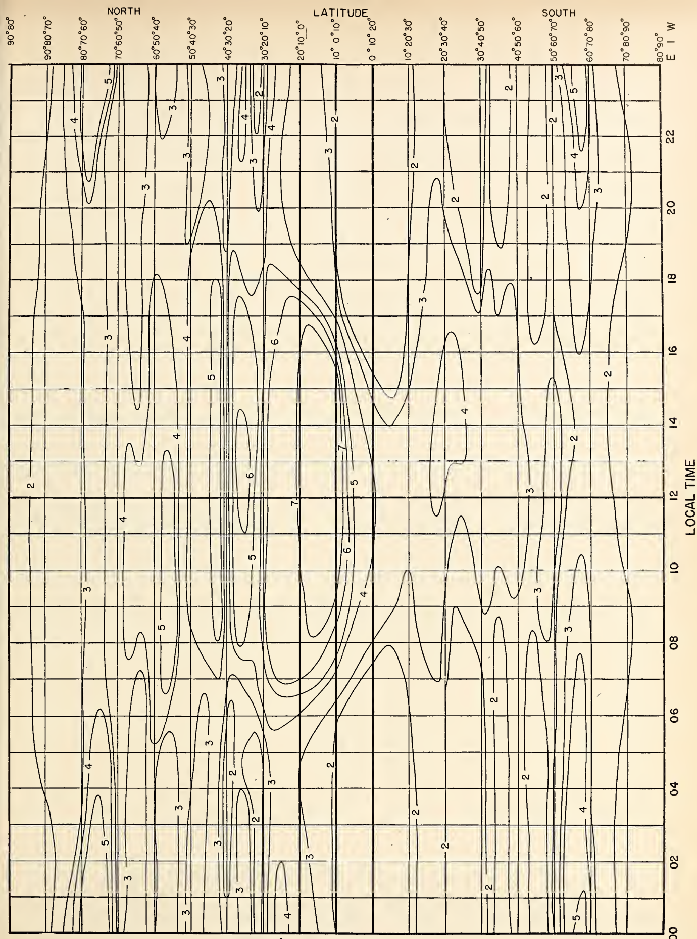
Fig. 12. MEDIAN fE_s , IN Mc, PREDICTED FOR JULY 1947
