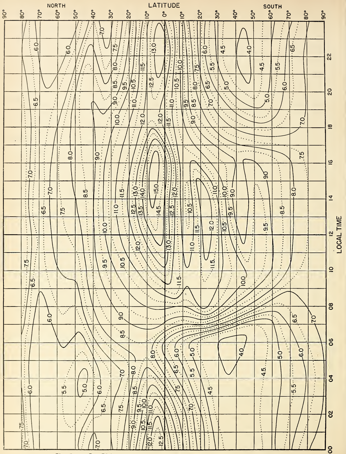
Fig. 5. F_2 ZERO-MUF, IN Mc, W ZONE, PREDICTED FOR JULY 1947
