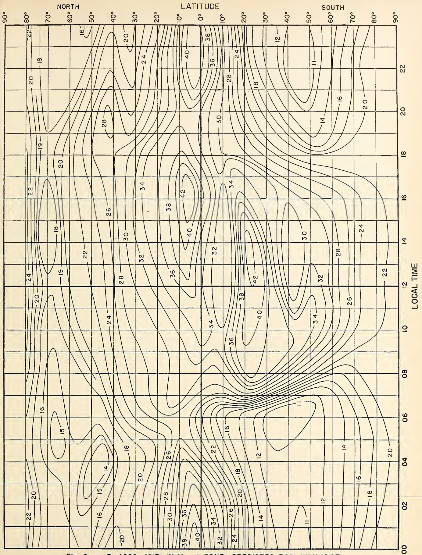
Fig. 6. F_2 4000-MUF, IN Mc, W ZONE, PREDICTED FOR JULY 1947
