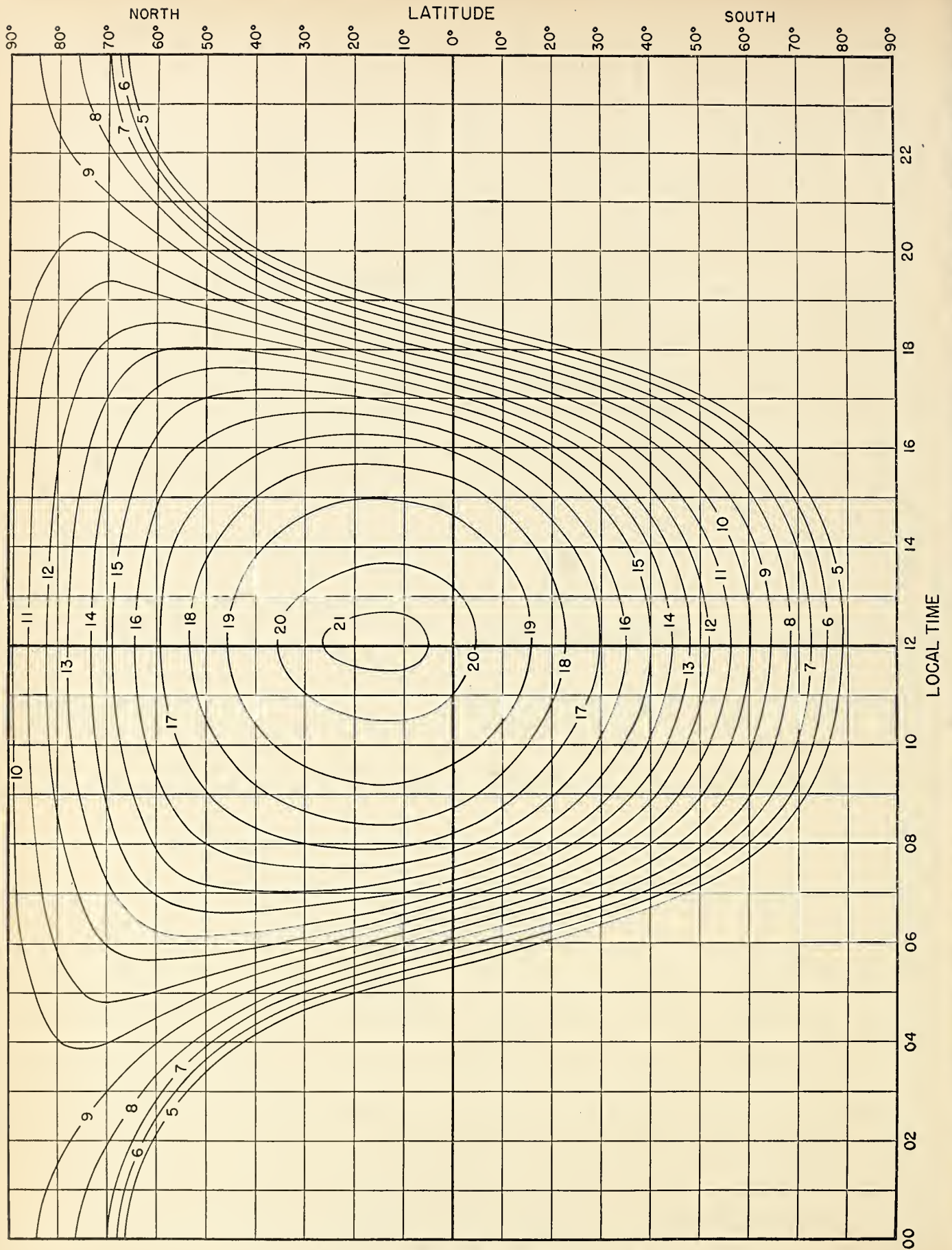
Fig. II. E-LAYER 2000-MUF, IN Mc, PREDICTED FOR JULY 1947
