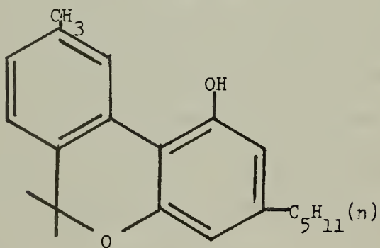
Cannabinol (CBN)
