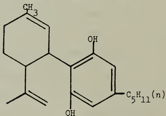
Cannabidiol (CBD)
