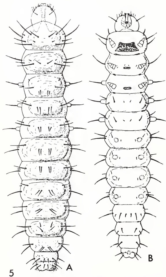
Leucoptera malifoliella . 4A-C. Ovipositor. A. Dorsal, B. Lateral, C. Ventral views. 5A-B. Last-instar larva. A. Dorsal view. B. Ventral view (From Zangheri and Ravelli 1957).
