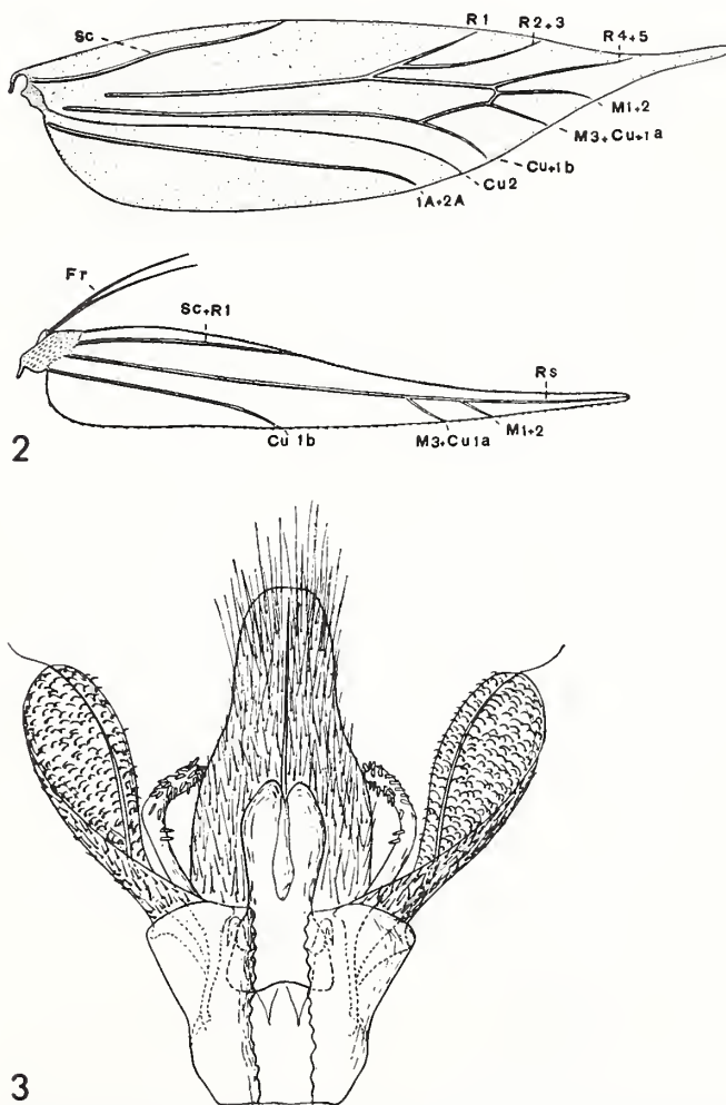
Leucoptera malifoliella . 2. Female wing venation. 3. Male genitalia, ventral view (2 from Ferro 1961; 3 from Zangheri and Ravelli 1957).
