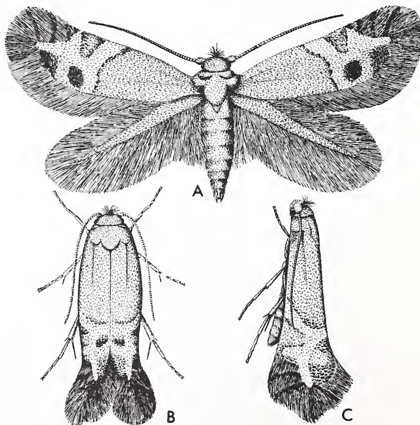
Leucoptera malifoliella adult. A. Wings expanded, dorsal view, B. At rest, dorsal view, C. Lateral view (From Ferro 1961).
