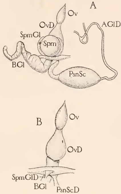
Fig. 2.—A, poison apparatus and sex organs of abnormal queen from dorsal side. \times 7\frac{1}{2} . B, ovary and oviduct of abnormal queen. \times 10 . AGID, duct of acid gland. BGI, alkaline gland. Ov, ovary. OvD, oviduct. PsnSc, poison sac. PsnScD, duct of same. Spm, spermatheca. SpmGID, duct of same.
