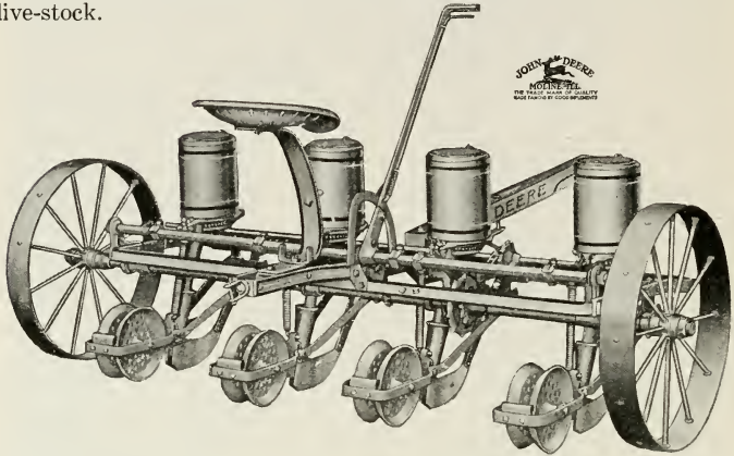
Four-Row Beet and Bean Planter .. This Machine Sows Sorghum, Broom Corn or Sudan Grass
