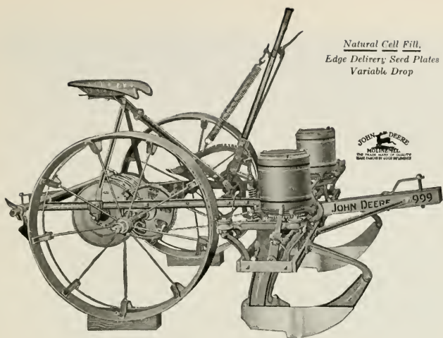
John Deere No. 999 Planter
