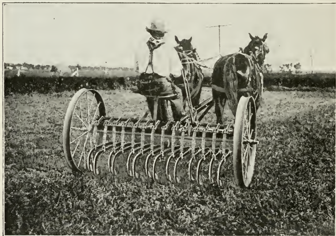
The Deere Alfalfa cultivator .. This Implement Breaks Up the Crowns, Stimulates the Growth of Plants. Removes Weeds and Thickens the Growth
