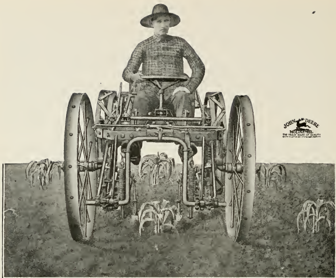
The "Tractor" Cultivating Corn on the Deere Experimental Farm
