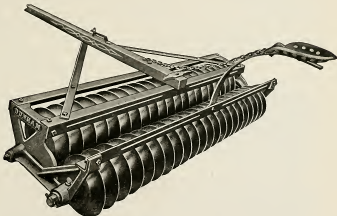
Culti-Packer: This Implement Is Invaluable as a Clod Crusher, Pulverizer and Mulch Former
