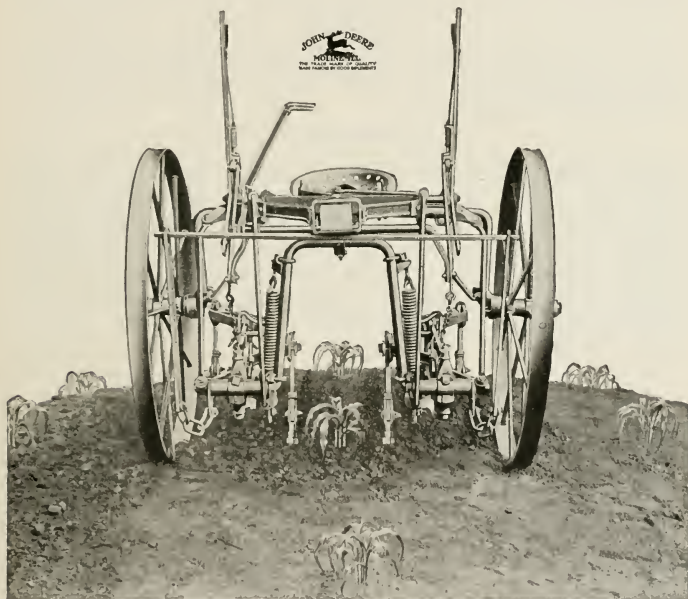
Hoof Shovels or Sweeps Can Be Used on this Corn Cultivator .. Sweeps Are Splendid for Surface Cultivation
