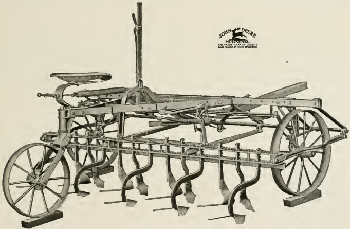
Four-Row Beet and Bean Cultivator
