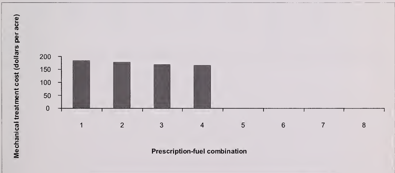
Figure 5—Average mechanical treatment cost for thinning from below to 50, 100, 200, and 300 trees per acre with machine piling and burning (categories 1, 2, 3, and 4, respectively). Mechanical treatment cost is zero for broadcast burning scenarios.
