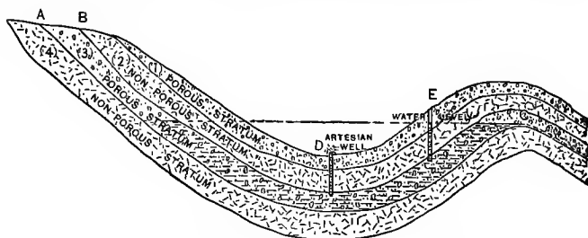
Fig. 7. Conditions producing artesian wells.
