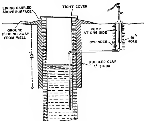
Fig. 10. A good dug well.
