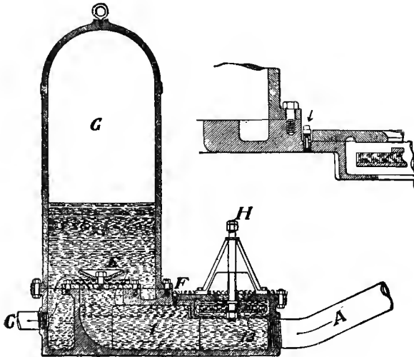
Fig. 75. Sectional view of Niagara hydraulic engine.
