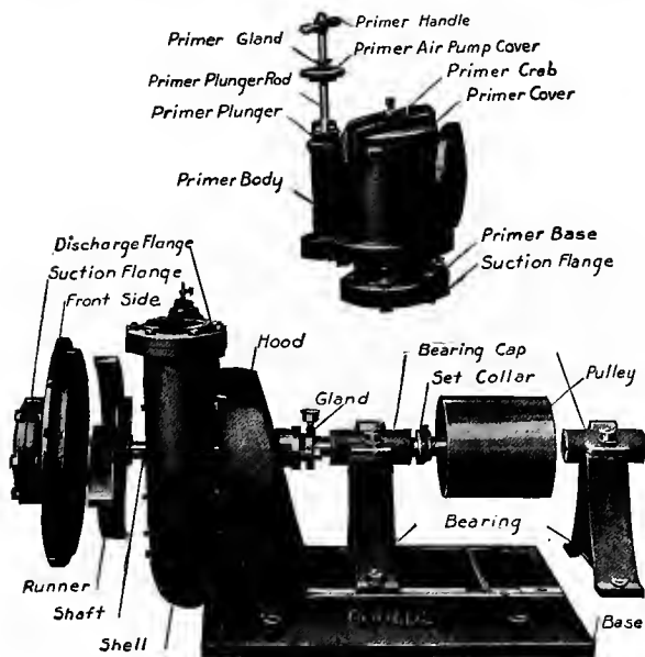
Fig. 44. Centrifugal pump.
