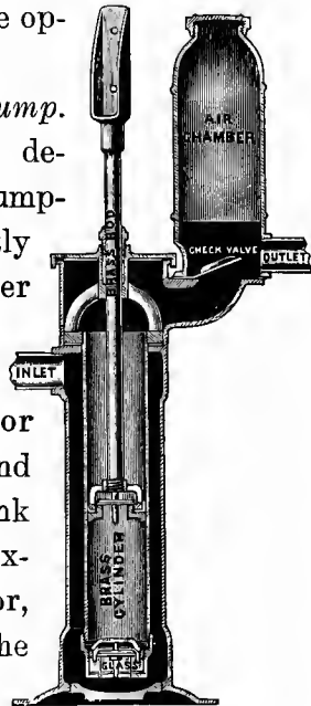
Fig. 40. Siphon force pump.
