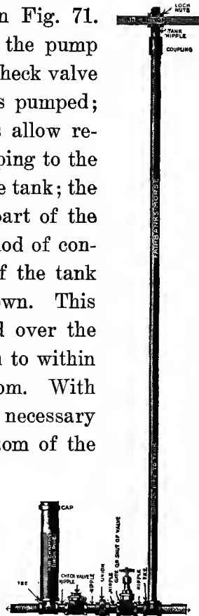
Fig. 71. Piping from pump to tank.
