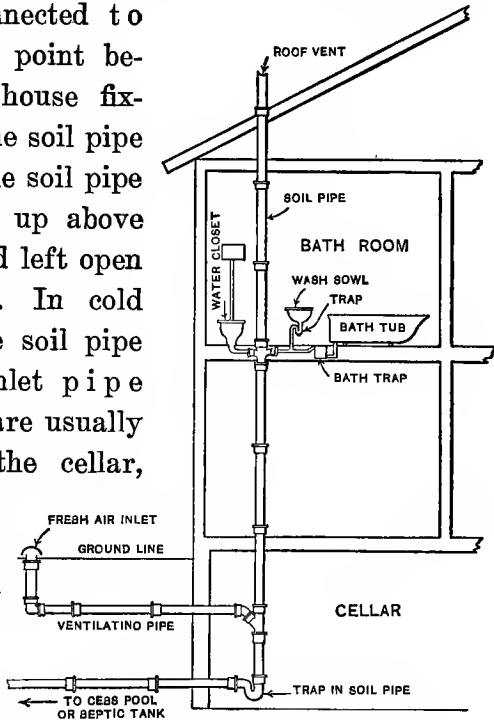
Fig. 104. Bathroom fixtures connected to soil pipe.
