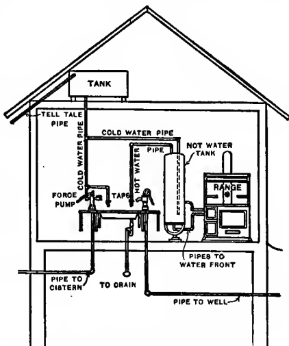
Fig. 4. Running hot water added to kitchen equipment.
