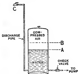
Fig. 53. Sectional view of pneumatic tank.
