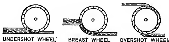
Fig. 98. Waterwheels.
