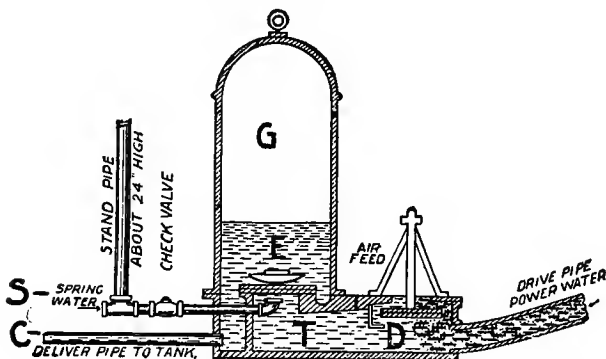
Fig. 76. Double-acting ram.
