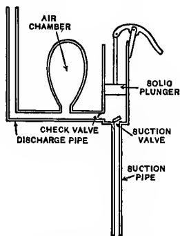
Fig. 32. Force pump with solid plunger.
