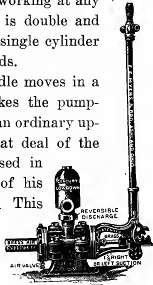
Fig. 41. Double-acting low-down force pump.
