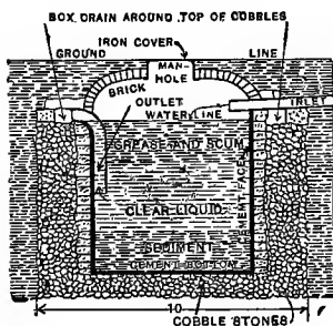
Fig. 105. Watertight cesspool.
