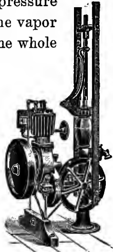
Fig. 85. Air-cooled engine.
