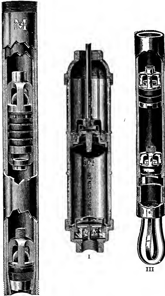
Fig. 42. Deep well cylinders.
