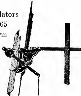
Fig. 63. Windmill regulator.
