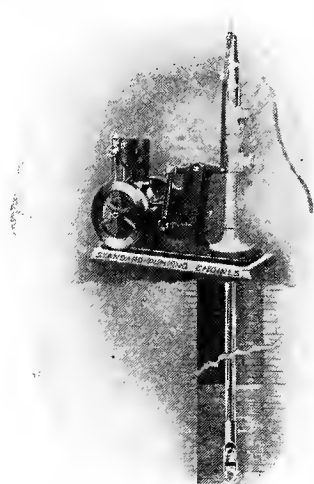
Fig. 90. Gasoline engine operating shallow well pump.
