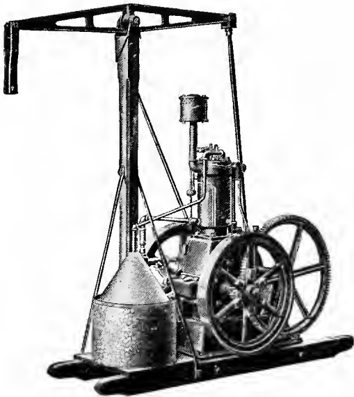
Fig. 87. Water-cooled engine geared to walking-beam pump jack.
