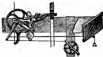
Fig. 65. Windmill regulator.
