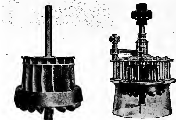
Fig. 101. The Samson runner. Fig. 102. The Samson turbine.
