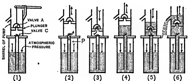
Fig. 31. How and why pumps work.
