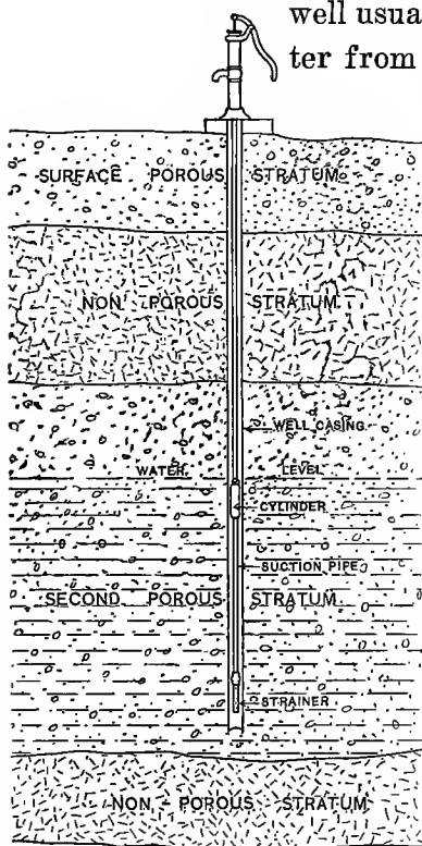
Fig. 15. The drilled well.
