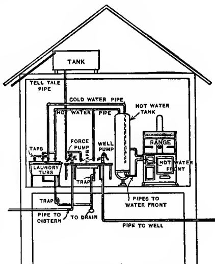
Fig. 5. Set laundry tubs added to kitchen equipment.
