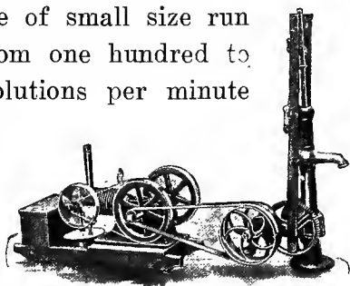
Fig. 89. Belt-driven pump jack.
