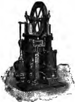
Fig. 80. Rider hot-air engine.
