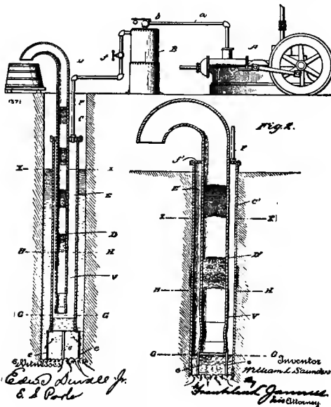
Fig. 45. Air-lift pump.
