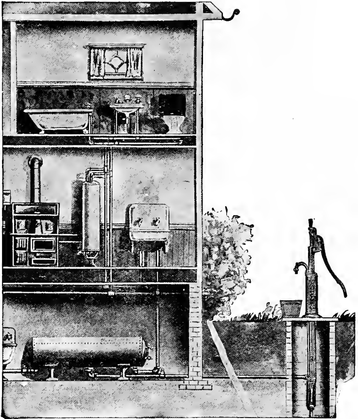
Fig. 51. Pneumatic tank water-supply system.
