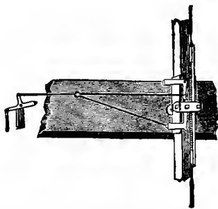
Fig. 64. Windmill regulator.
