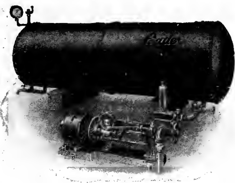
Fig. 95. Motor-driven pump operating a pneumatic tank.
