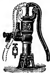
Fig. 36. Force pump.
