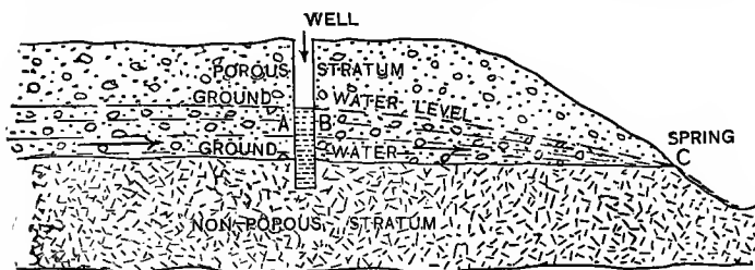
Fig. 6. Underground water, the source of water in wells and springs.
