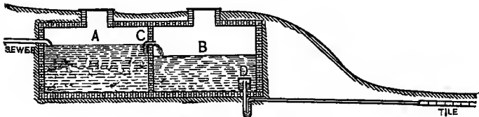
Fig. 106. The septic tank.
