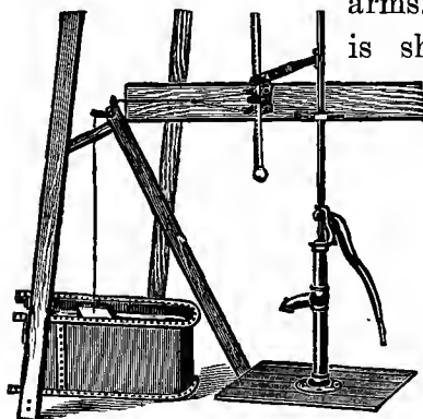
Fig. 61. Windmill regulator.
