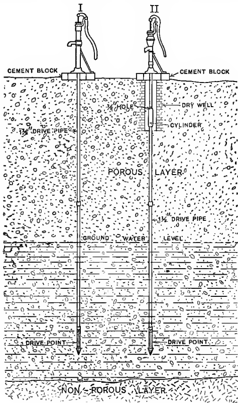
Fig. 12. Driven wells.
