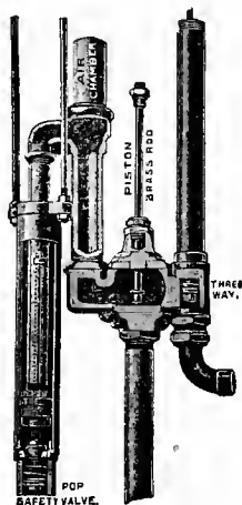
Fig. 66. Hydraulic cylinder.
