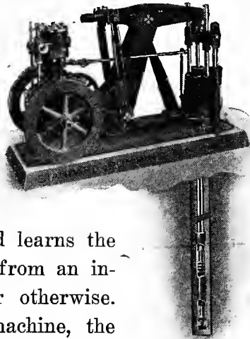
Fig. 91. Gasoline engine operating deep-well pump.
