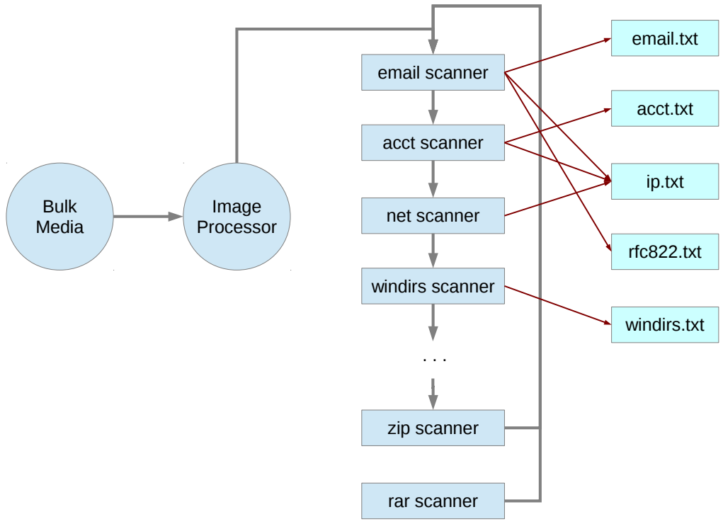
Figure 3.1: An abstract view of bulk_extractor processing chain and feature file population.
