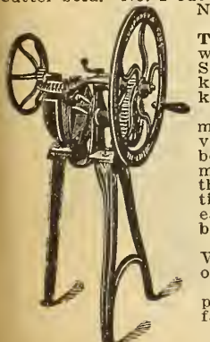
HUMPHREY'S BONE CUTTER
