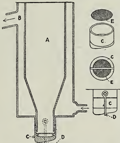
Fig. 3—Construction of Sediment Tester
