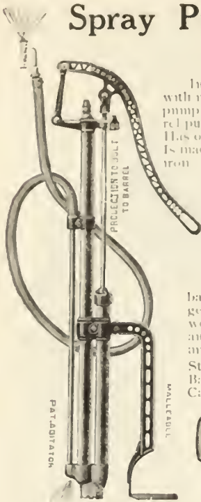
Holmes' Perfect Lever Bucket Pump
