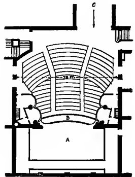
PLAN OF THE EMPIRE THEA- TER, NEW YORK
