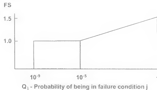
Figure 2: Factor of safety for continuation of flight
