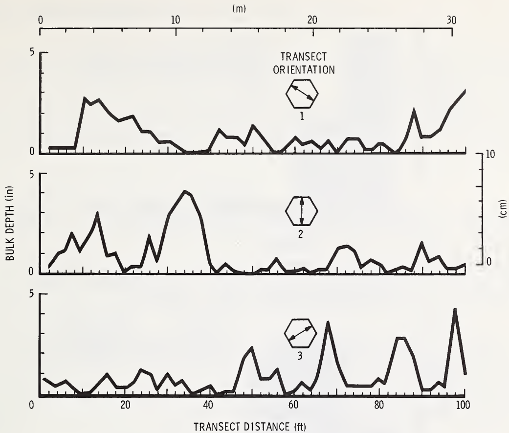
Figure 2.--A representative transect of the bulk depth evaluated every 2 feet. Three orientations are shown: (1) 60^\circ counterclockwise to the uphill direction, (2) uphill, and (3) 60^\circ clockwise to the uphill direction.
