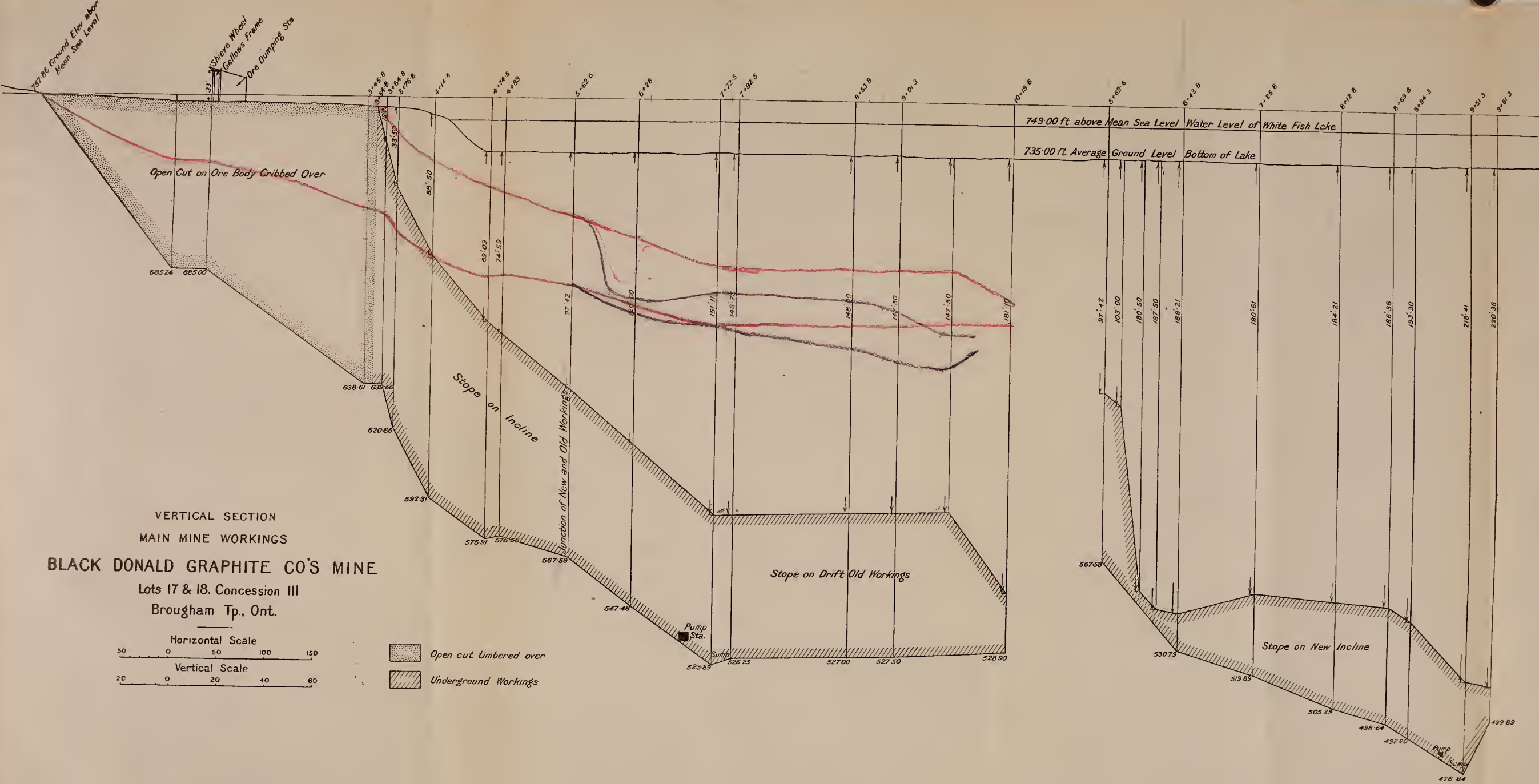
Fig. 4a. Section through working, Black Donald Mine, Brougham Township, Ont.
