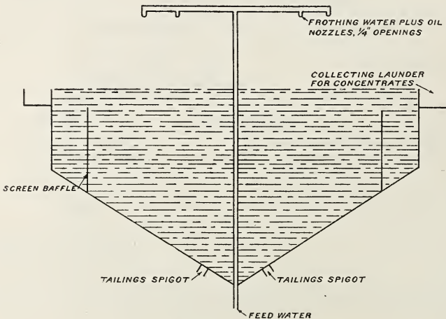
Fig. 32. Section through Simplex washer: not drawn to scale. Washer is elliptical, and measures about 6 feet by 3\frac{1}{2} feet. (United States Bureau of Mines.)
