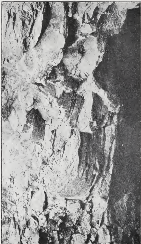
Folded structure in gneiss, range IV, lot 3, township of Buckingham, Que. The ore-body follows the crest of the pitching fold shown above.
