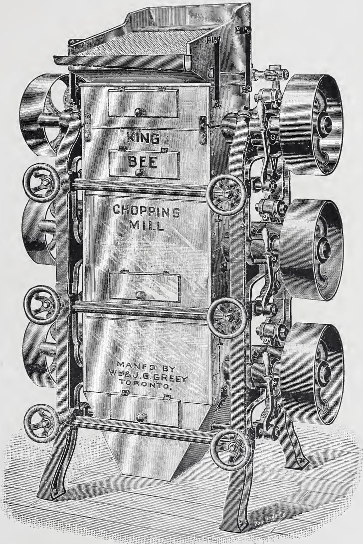
Type of rolls used in Canadian mills employing the dry concentrating process. (Wm. and J. G. Greay, Toronto, Ont.)
