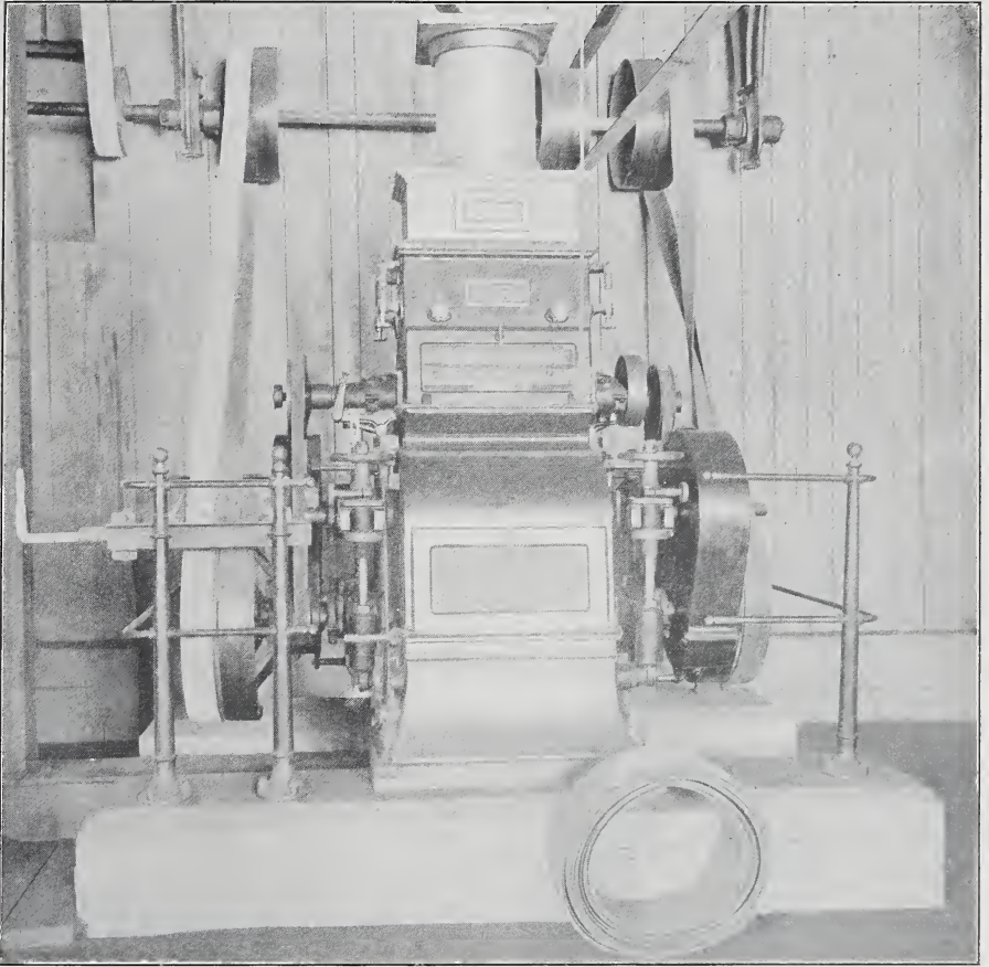
Photo, New Quebec Graphite Company, Buckingham, Que.
