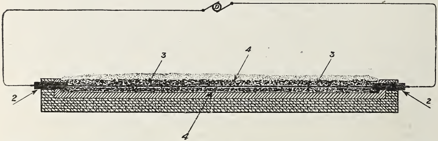
Fig. 39. Section through electric furnace for the production of artificial graphite. 2, electrodes; 3, core of powdered coal; 4, mixture of powdered coal or coke and sand; D, source of energy.
