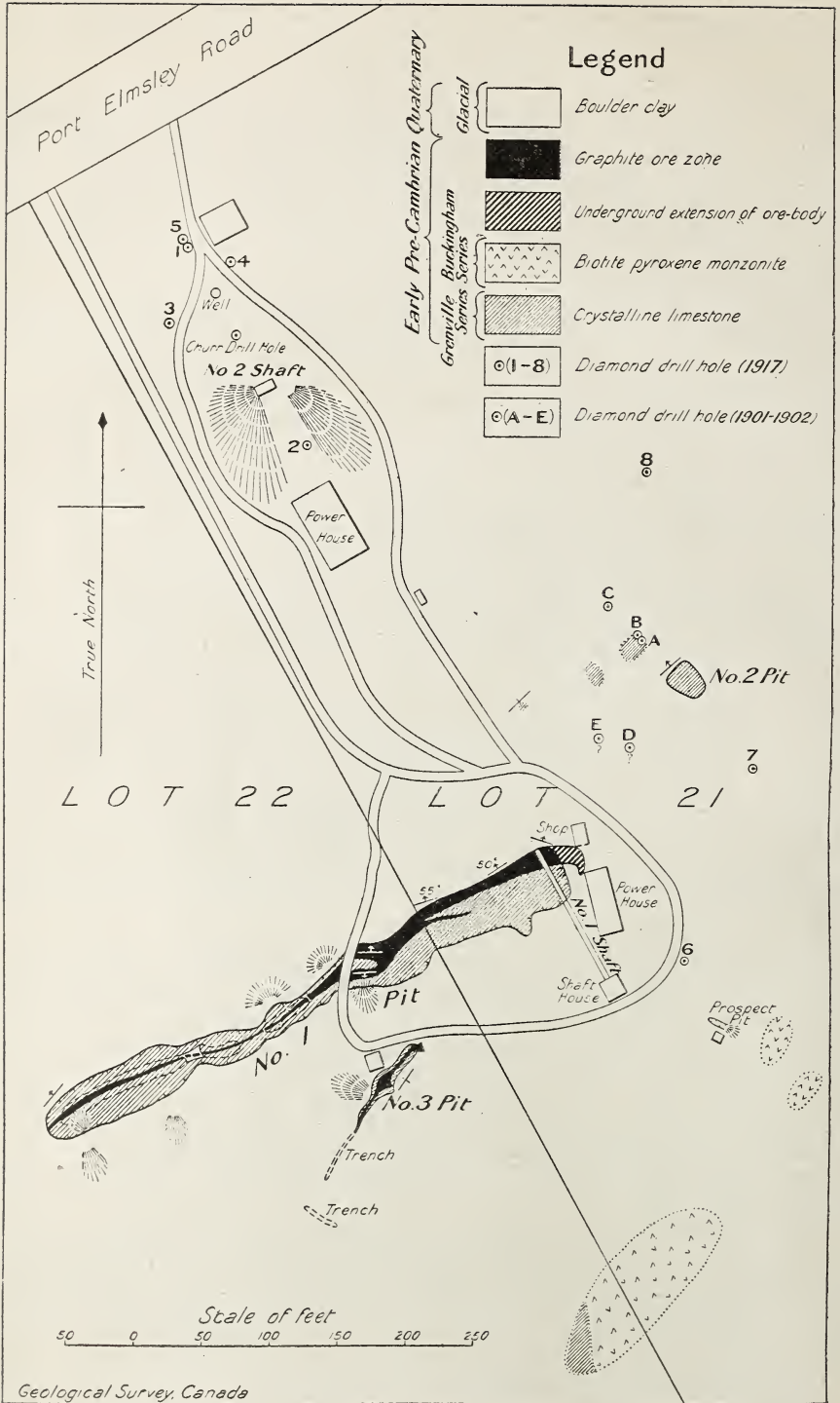
Fig. 1. Surface plan at mine of Globe Graphite Mining and Refining Company, lots 21 and 22, concession VI, North Elmsley township, Lanark county, Ontario.
