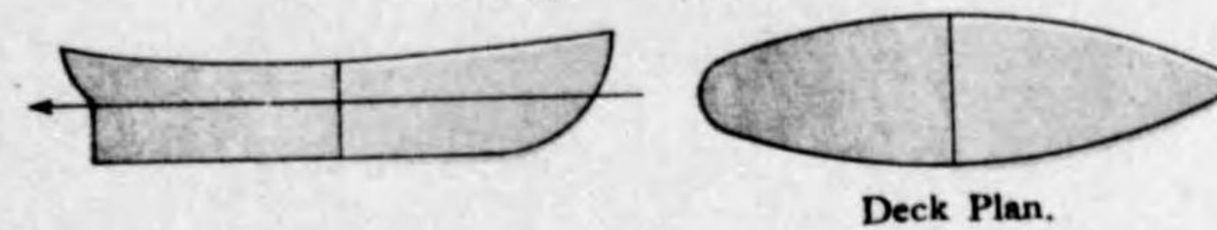
(1) Ship built head South on Magnetic Equator
