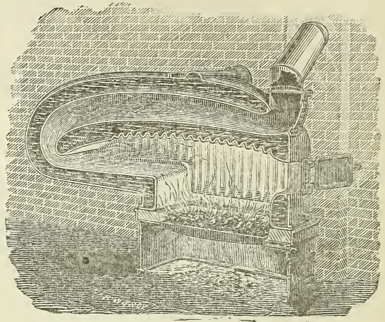
HITCHINGS' CORRUGATED BOILER.
