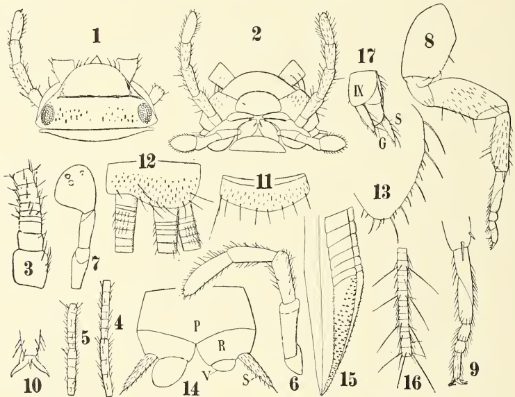
Fig. V. Lepidothrix pilifera MENGINE.
