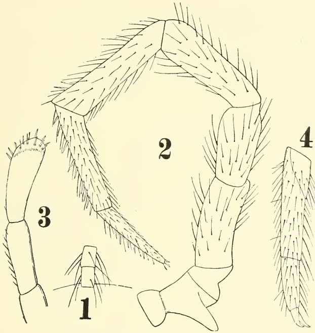
Fig. XII. Machilis capito v. OLF.
