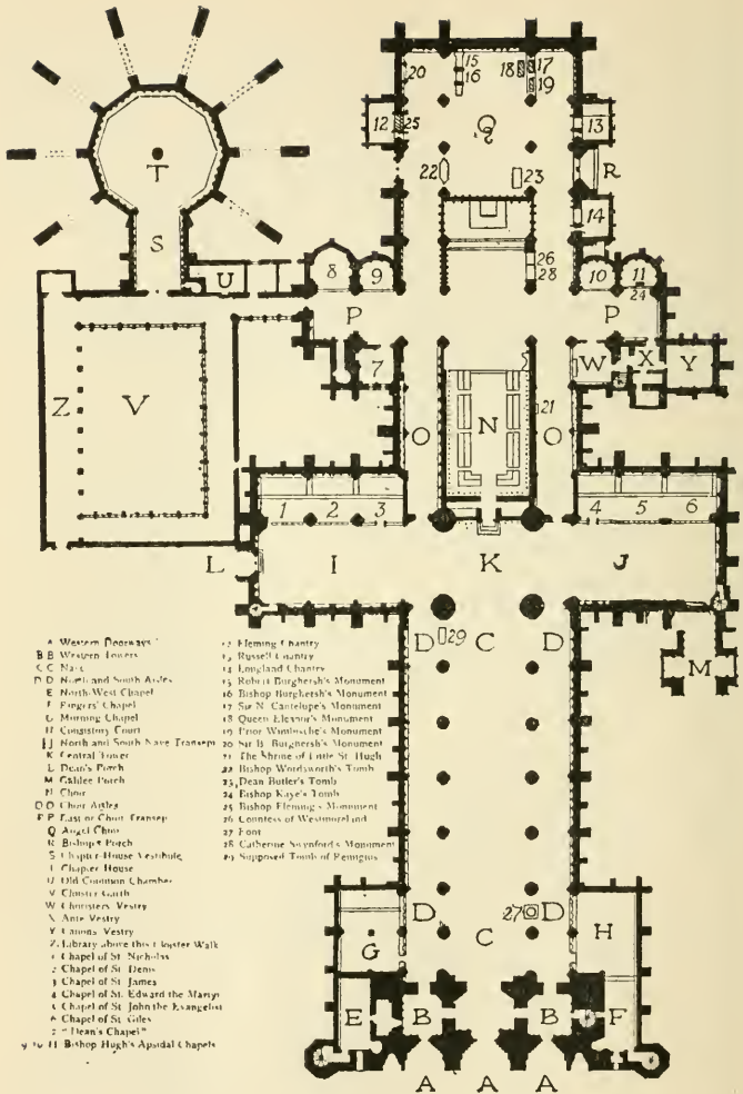
PLAN OF LINCOLN CATHEDRAL
