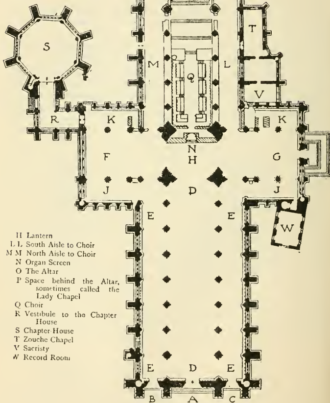
PLAN OF YORK CATHEDRAL
