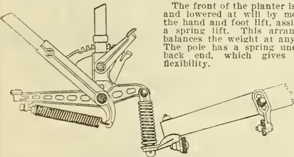
Spring Lift and Connection to Front Frame.
