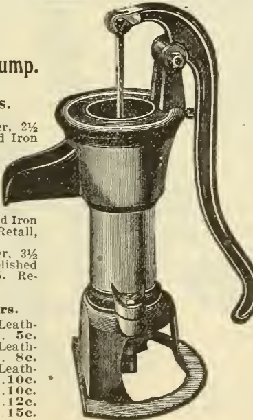
Fig. 72, No. 22. No. 22—Single-Acting, Set Length, Hand Force Pump, 6-inch stroke, 3-inch Iron Cylinder. Fitted for 1 1/4-inch pipe. Same as Fig. 41, but can be extended to 50 feet; will fit 5-inch cased well. Price, List, $12.50; Retail, $6.50.
