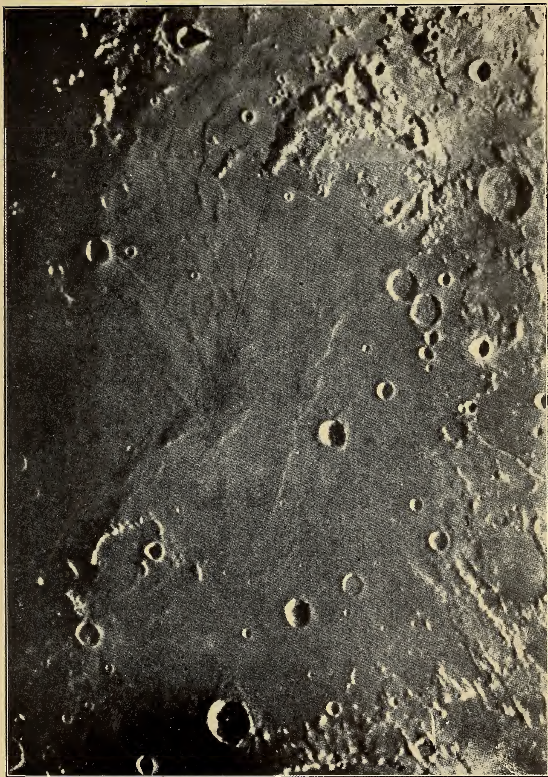
MARE TRANQUILLITATIS AND SURROUNDINGS
