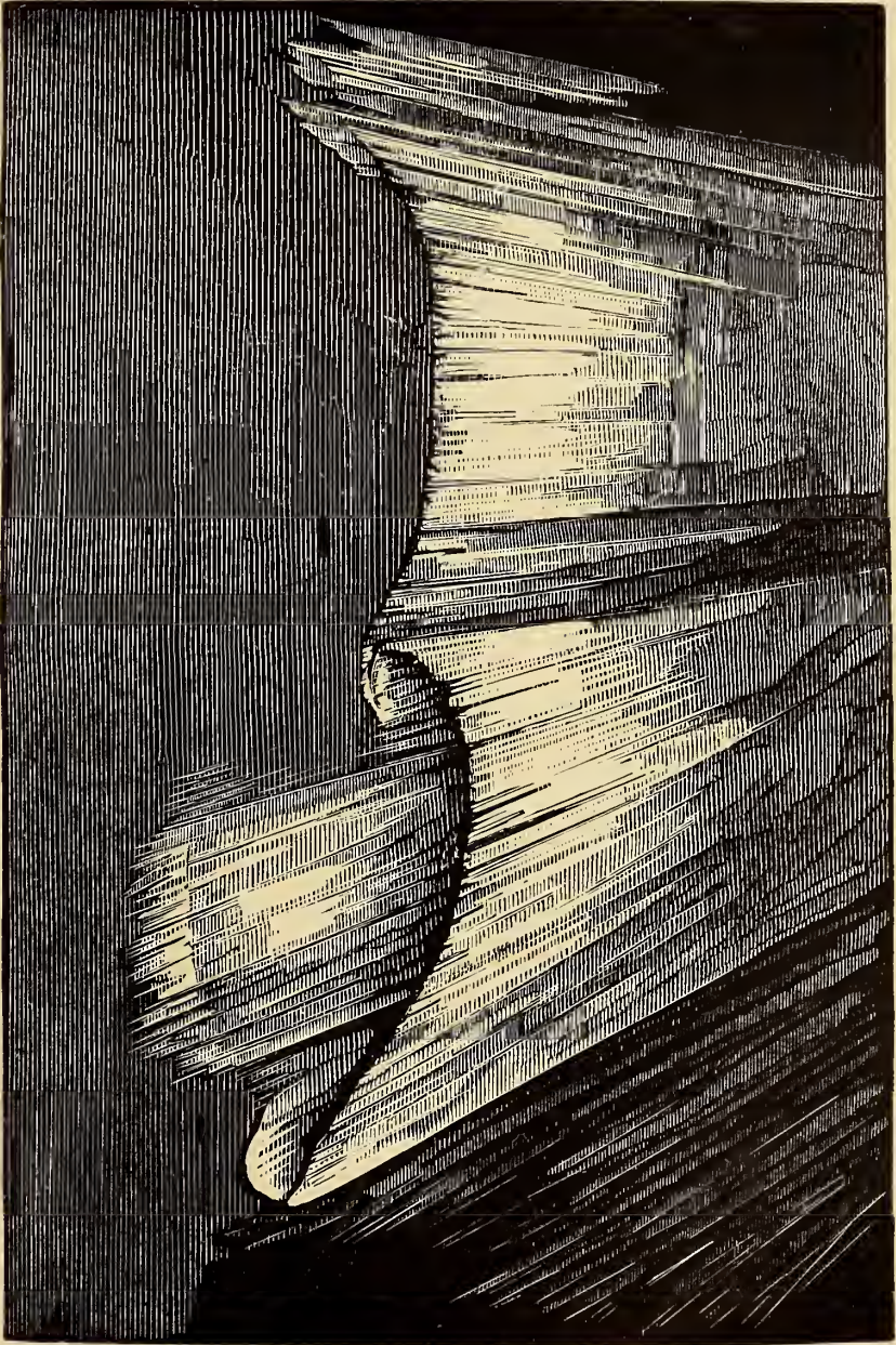
AURORAL CURTAIN SEEN IN SCANDINAVIA
