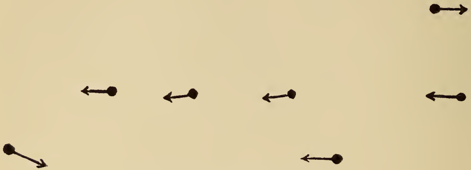
THE "GREAT DIPPER" AS IT IS
