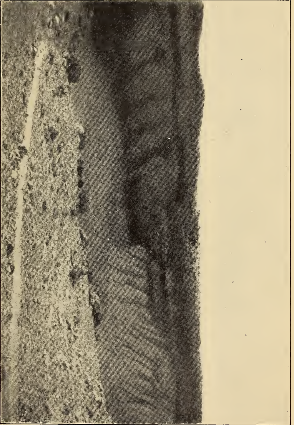
LOOKING ACROSS COON BUTTE CRATER FROM NORTHERN RIM
