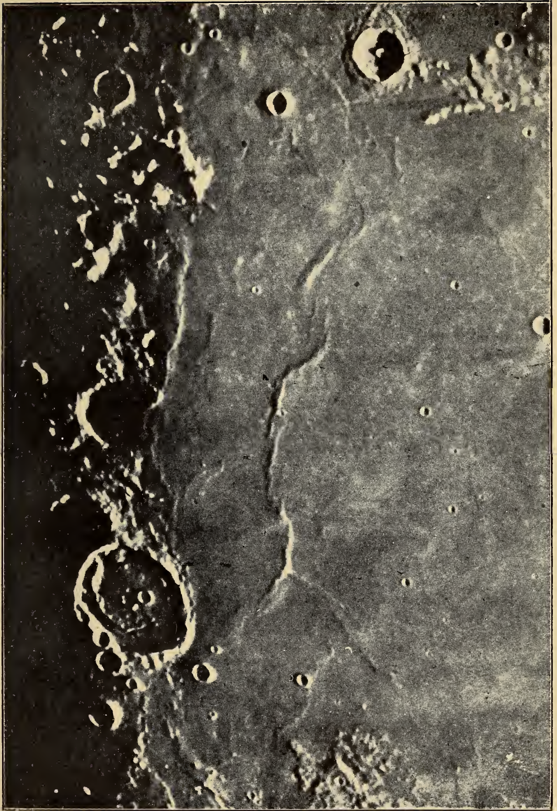
WESTERN PART OF THE MARE SERENITATIS
