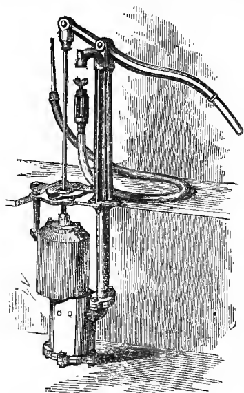
Fig. 24.—WEST'S FORCE PUMP.
