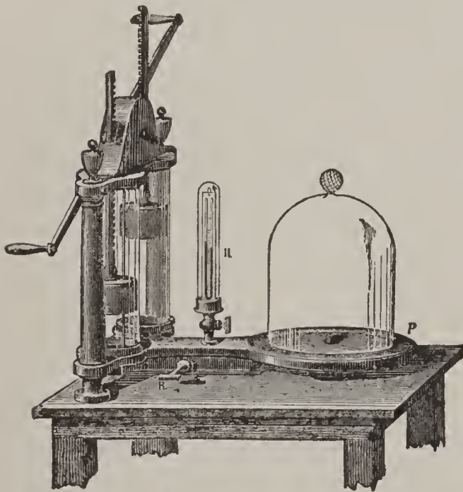
Fig. 2.—Air-pump.
