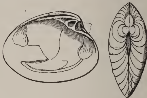
Bivalve Shell.
