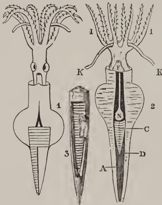
Belemnites.
