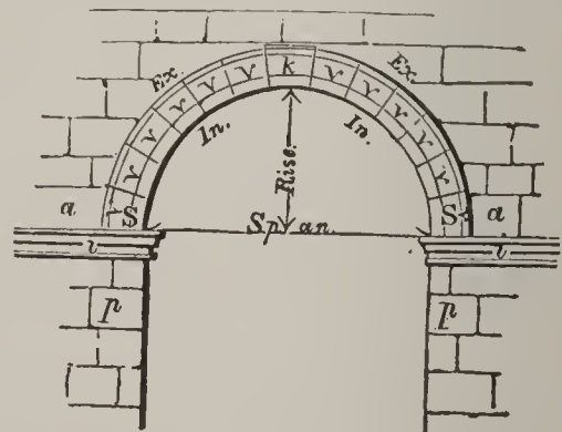
Parts of an Arch.
