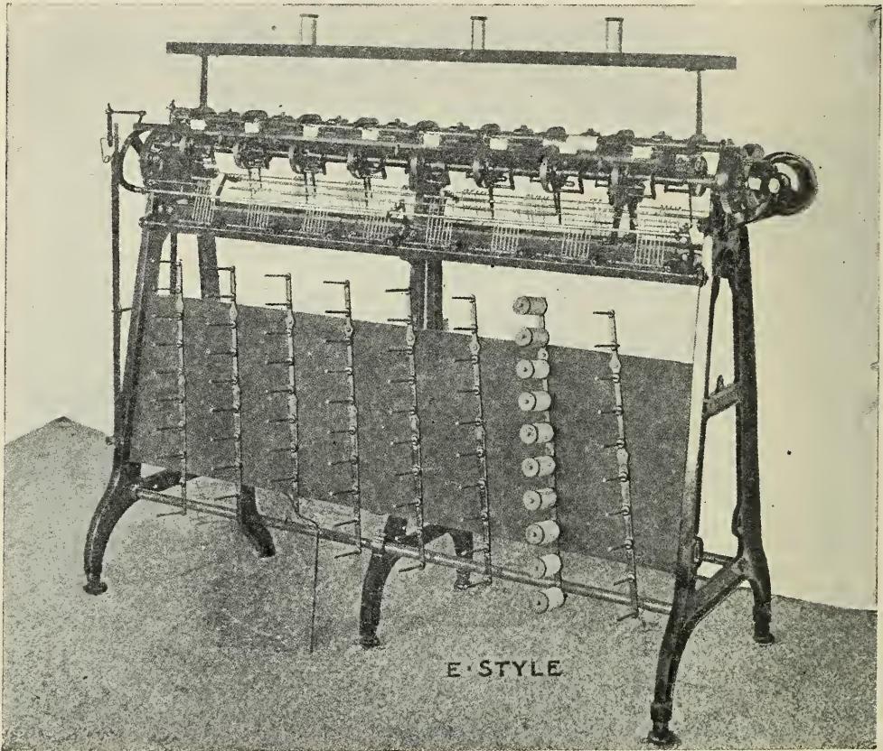
FIG. 17.— Doubling Machine.
