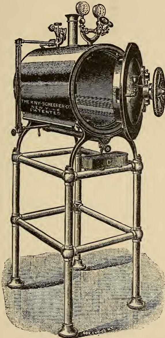
Steam-sterilizer (Kny-Scheerer).
