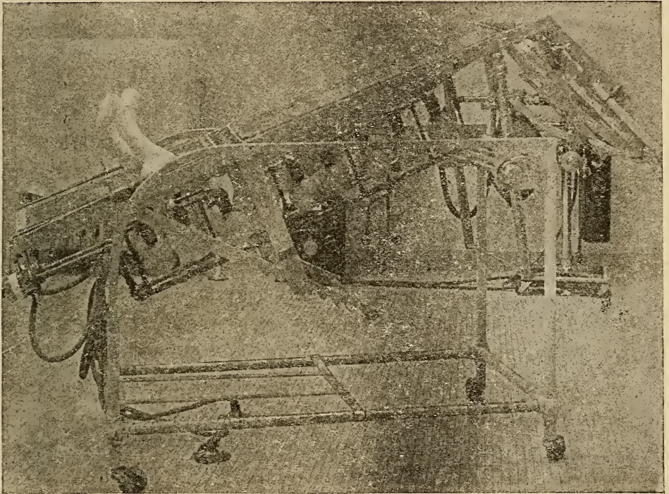
Boldt's operating-table, with (author's) electric light attachment.
