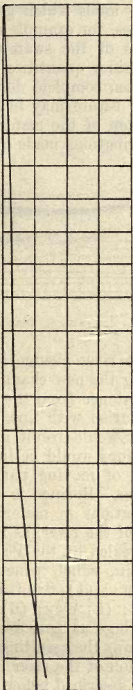
Fig. 5. Profile of Wabash river.
