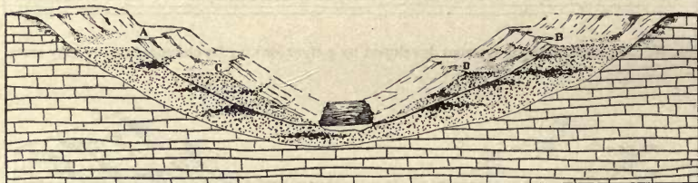
FIG. 28. Diagram showing two sets of terraces developed from aggradational flats.
