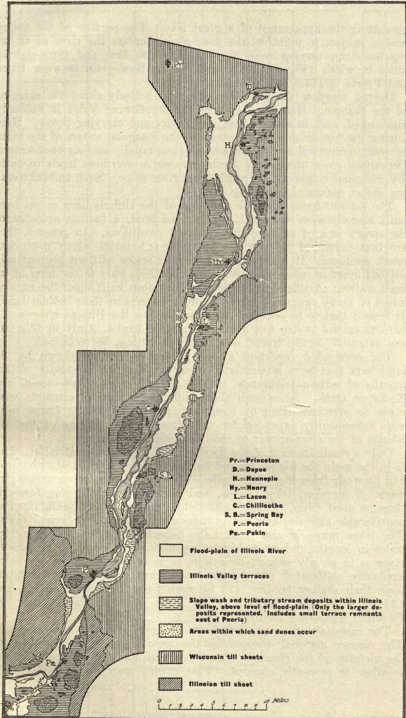
FIG. 3. Map showing general distribution of certain leading features of the region.
