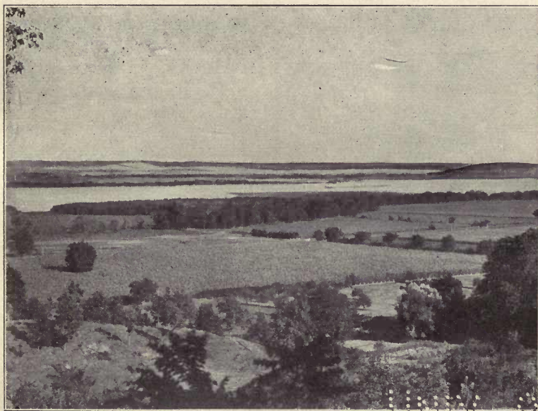
B. The flat in the middle foreground is part of an extensive terrace between Peoria and Mazon. The lower slopes of the valley side appear in the immediate foreground. (Photo by Dewein.)
