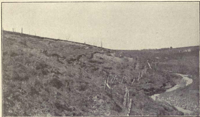
A. The widening of a valley by slumping.
