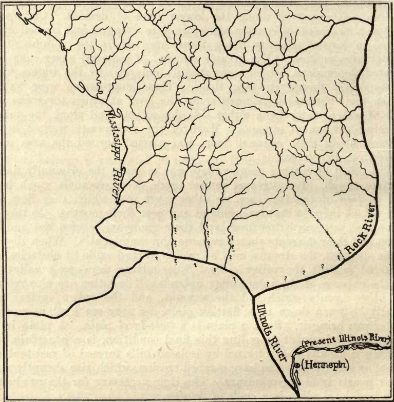
FIG. 16. Map showing portion of pre-glacial Rock-Illinois river system. (Leverett.)
