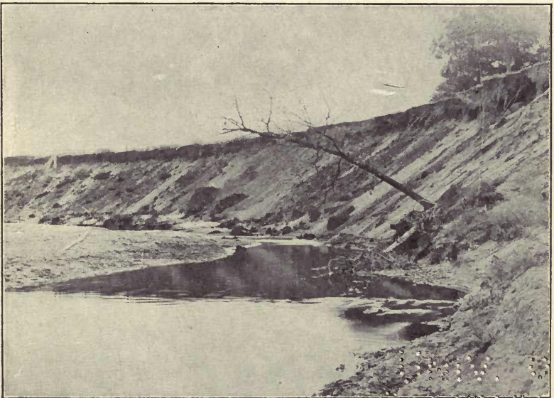
B. Crow creek, west of Henry, widening its valley by lateral erosion. (Photo by Crane.)
