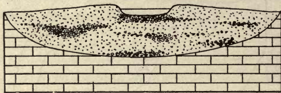
FIG. 10. Diagram showing general structure of stream deposits.
