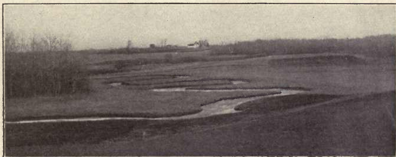
A. A meandering stream. (Photo by Neal.)
