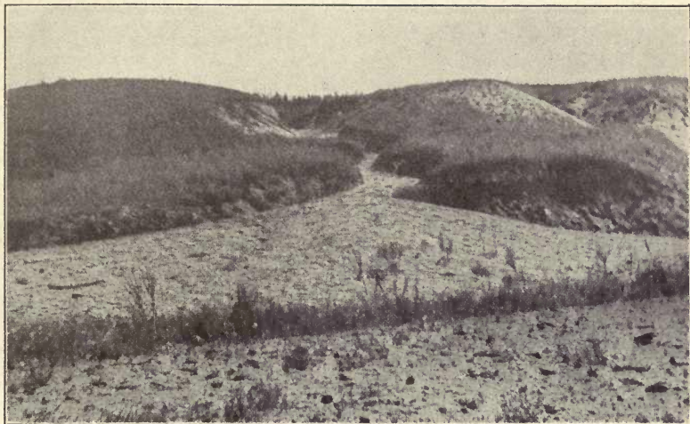
A. A small alluvial fan. (Photo by Crane.)
