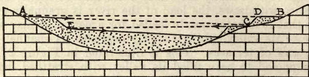
FIG. 27. Diagram illustrating development of terraces by a slowly degrading river which shifts from side to side of its valley.
