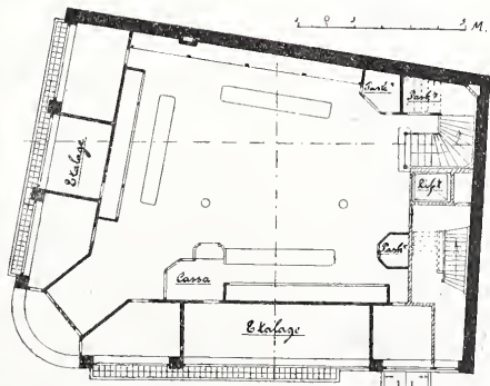
Plan beganegrond.
