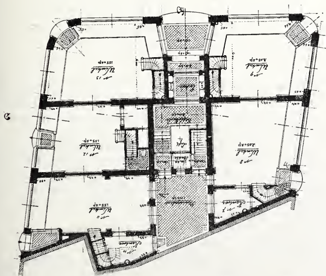
BEGANEGROUND.
