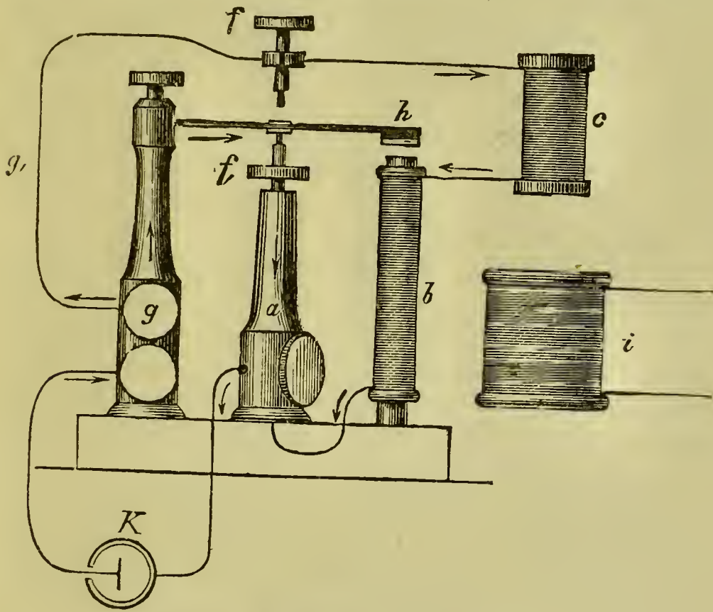
FIG. 74. HELMHOLTZ'S APPARATUS.
