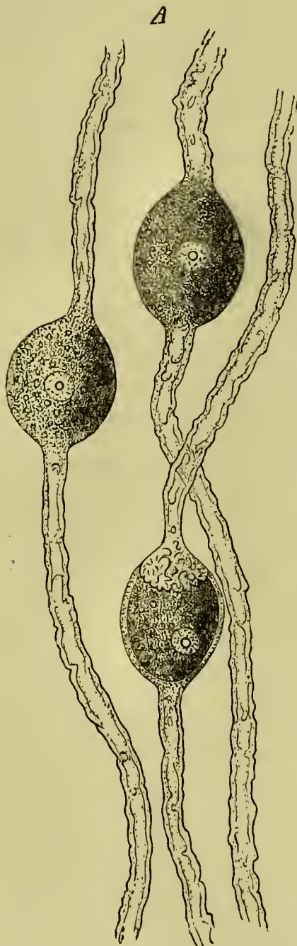
FIG. 27. GANGLION-CELLS WITH NERVE-PROCESSES.
