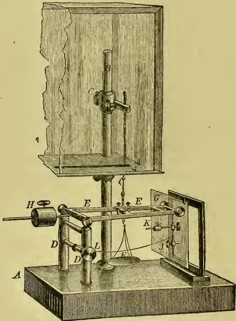
FIG. 8. SIMPLE MYOGRAPH.
