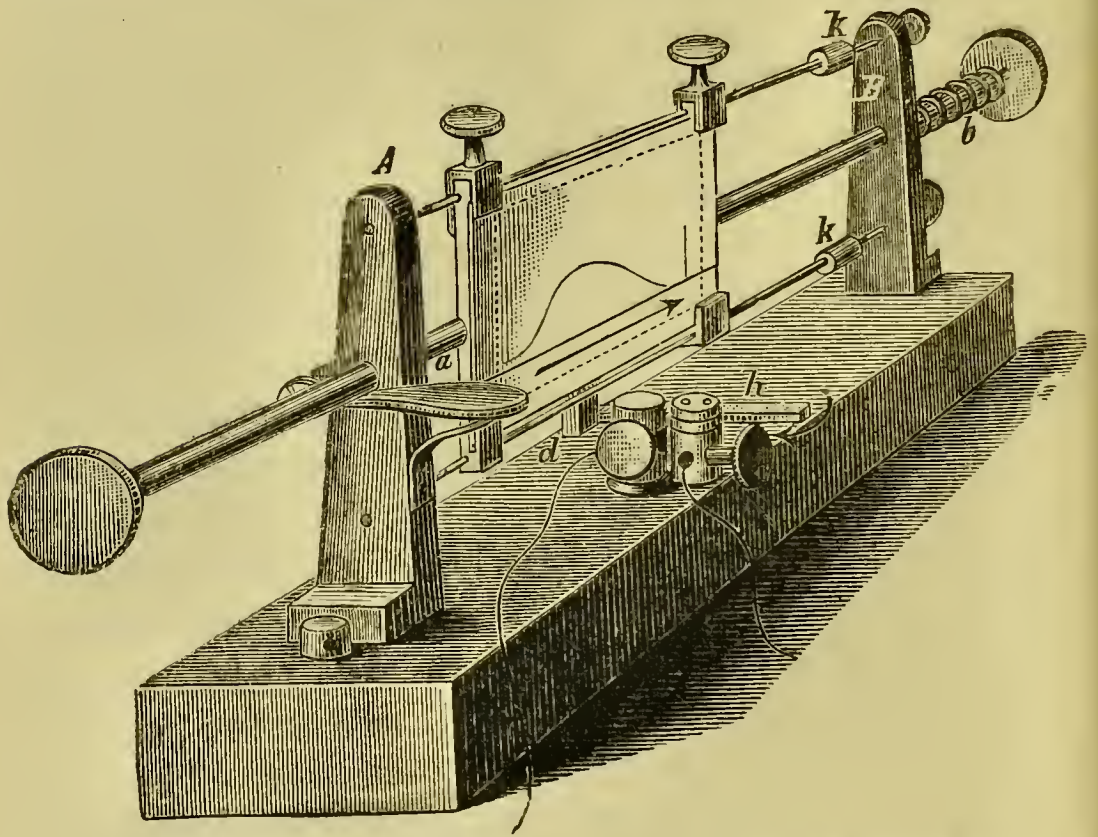
FIG. 28. SPRING MYOGRAPH, AS USED BY DU BOIS-REYMOND.
