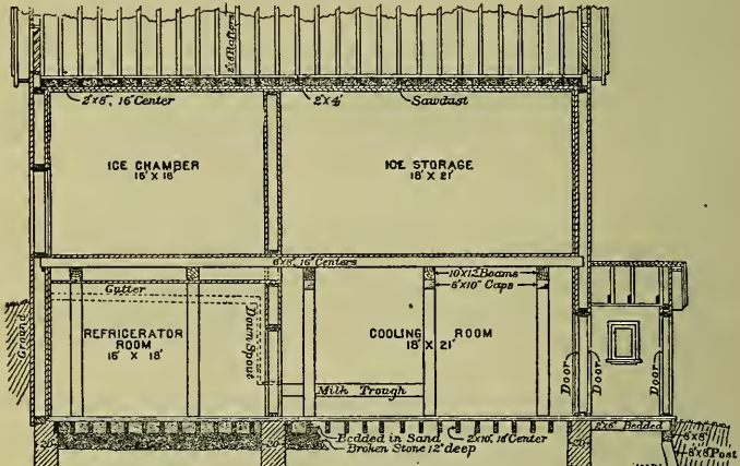
Fig. 56.—Kansas Cold Storage House; longitudinal section.
