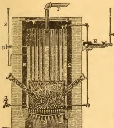
Sectional view of Magazine Boiler.
