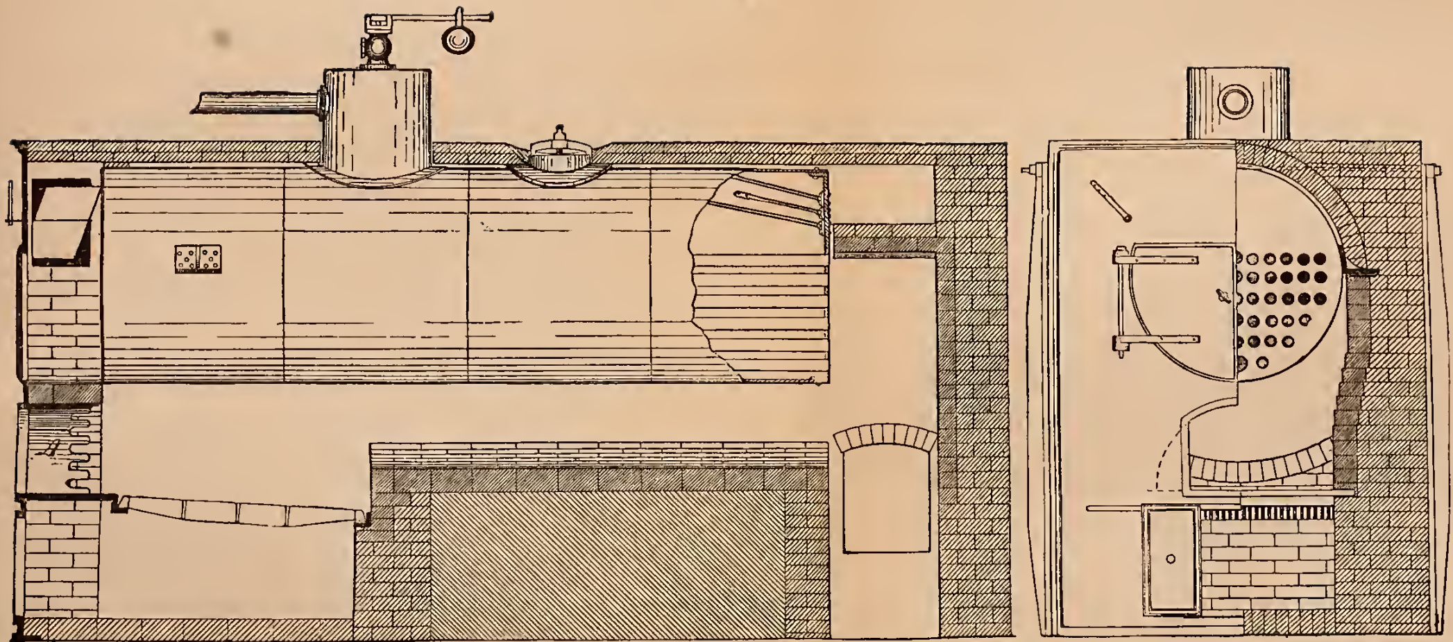
HORIZONTAL-MULTI-TUBULAR-BOILER.
