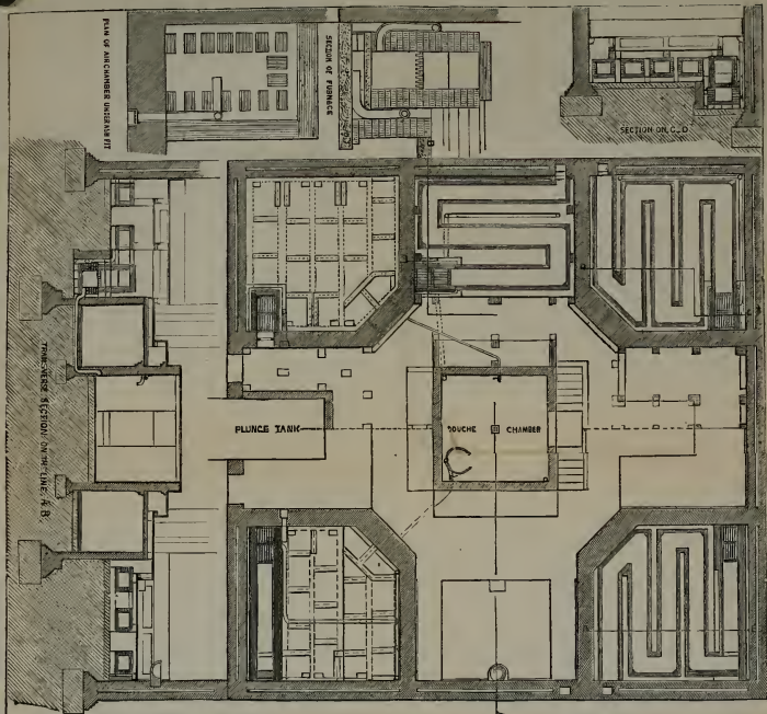
PLAN SHOWING SECTIONS AND FOUNDATIONS OF FLIES AIR PIPES &c
