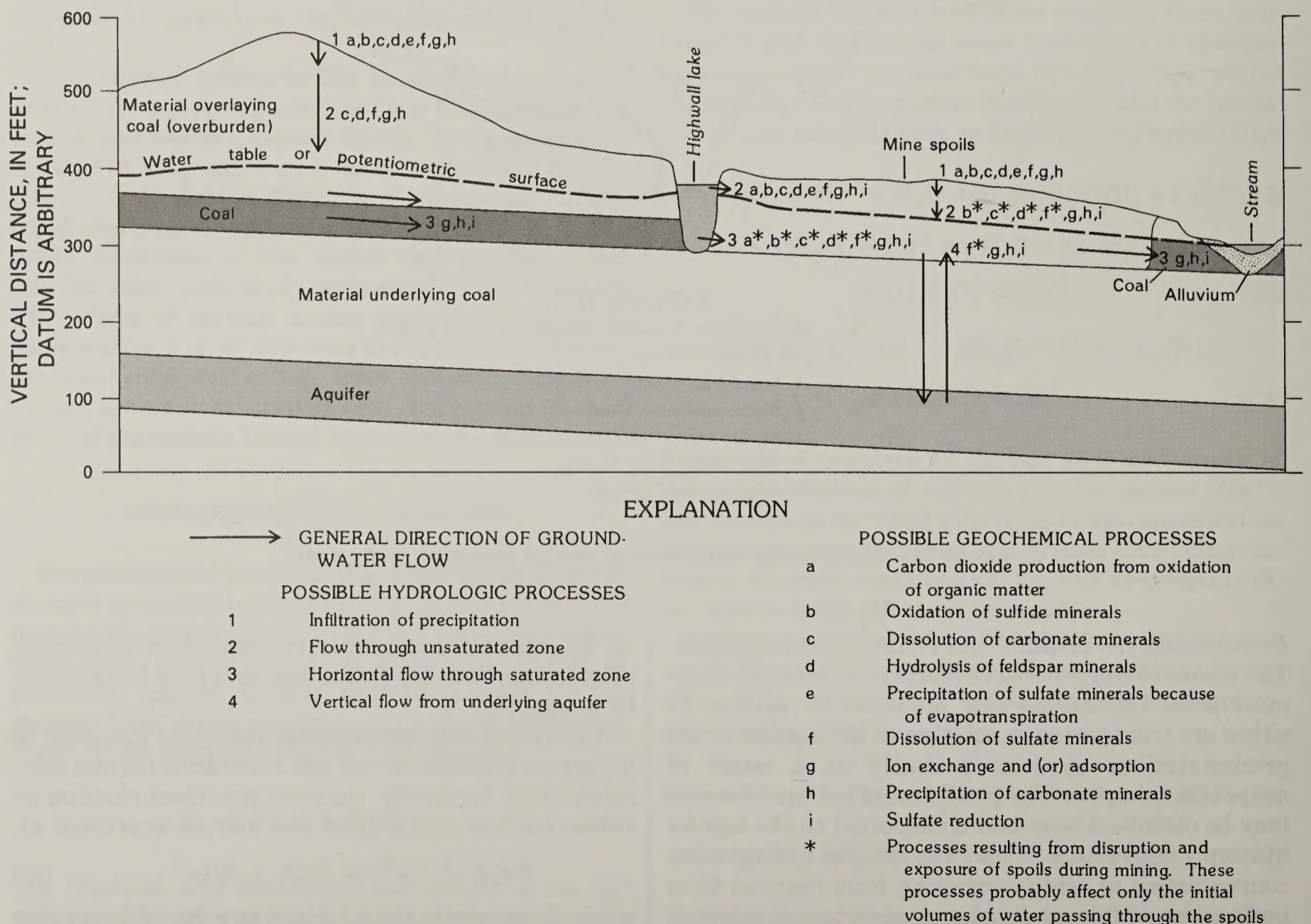
FIGURE 69.—Generalized section of hypothetical mine area and major hydrologic and geochemical processes.
