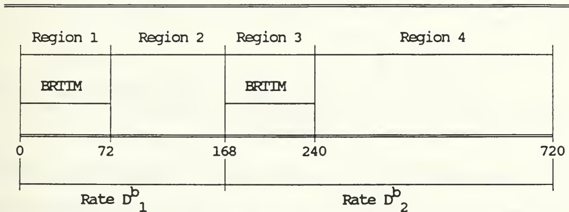
FIGURE 6-2 : TIME CHART FOR COMPUTATION OF THE BASE PIPELINE FOR LRU-D.
