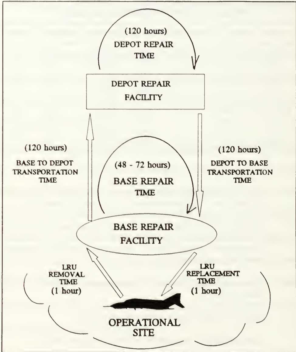
FIGURE 6-1 : MAINTENANCE STRUCTURE FOR THE EXAMPLE.
