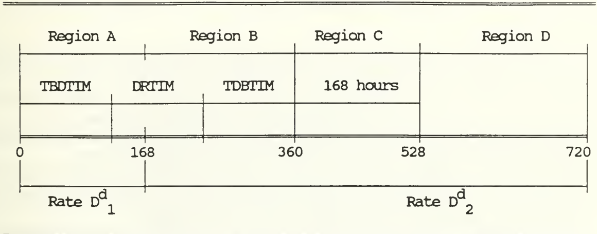
FIGURE 6-3 : TIME CHART FOR COMPUTATION OF THE TOTAL DEPOT PIPELINE FOR LRU-D.
