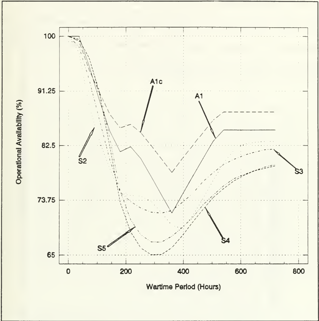
FIGURE 6-19: RESULTS OF OPERATIONAL AVAILABILITY ( A_0(t) ) FOR MODEL VARIATIONS WITH NO REPAIR CAPABILITY.
