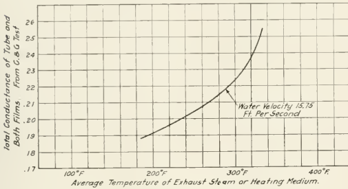
Fig. 5—Total Conductance for Various Average Temperatures at a Feed Water Velocity of 15.75 Ft. Per Sec.
