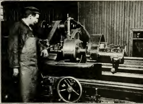
Fig. 11—Grinding Piston Valve Packing Rings
