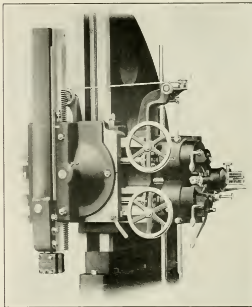
Fig. 4—Right Hand Head Showing Feed Mechanism
