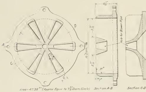
Fig. 20—Plain Annular Nozzle A-9
