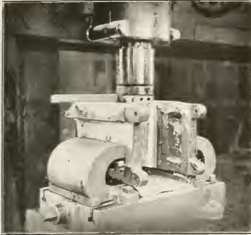
Fig. 7—Facing the Babbitted Surface of the Box
