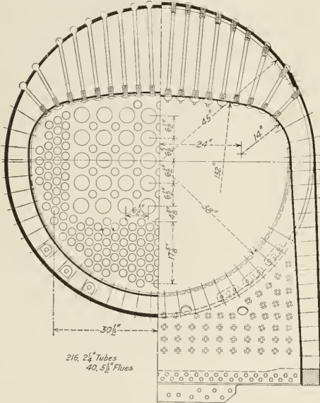
Sections Through the Firebox and Combustion Chamber
