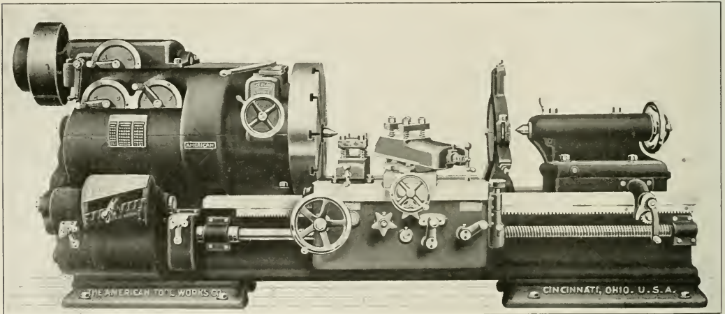
The American 36-In. Heavy Geared Head Lathe
