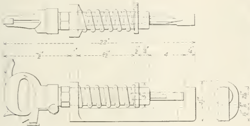
Nut Splitting Attachment for Thor Hammer
