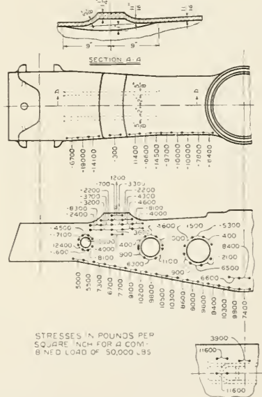
Fig. 7—Bolster "C" with Reinforced Side Bearings
