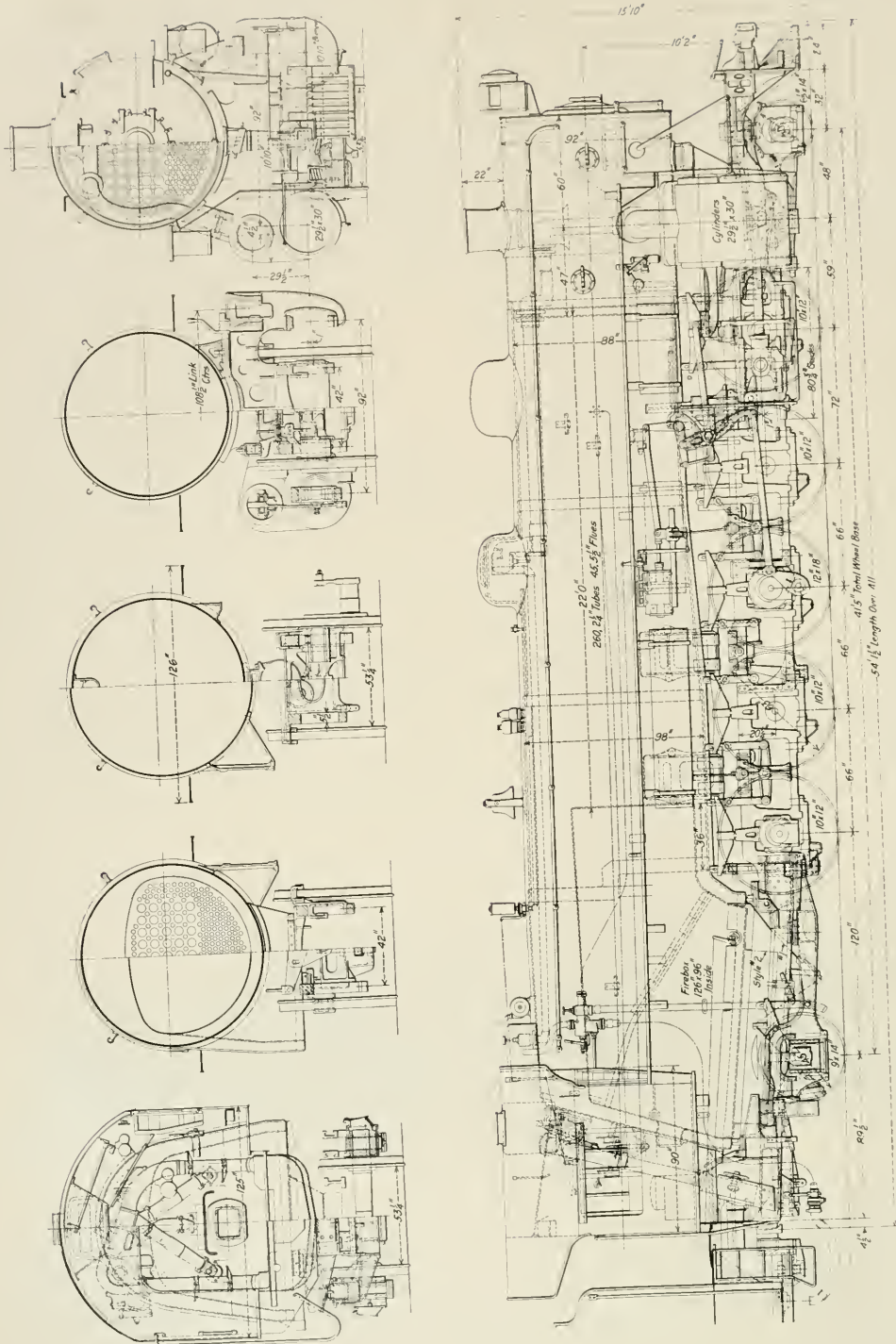
Elevation and Cross Sections of Union Pacific 2-10-2 Type Locomotive.
