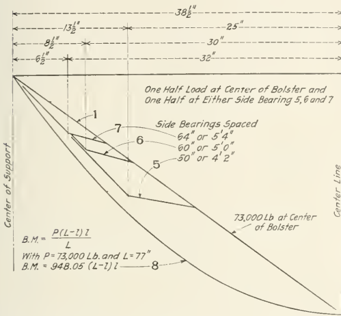
Fig. 2—Combined Bending Moment Diagrams
