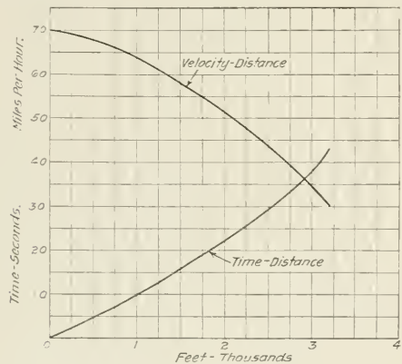
Fig. 7—Time-Distance and Velocity-Distance Curves for Deceleration
