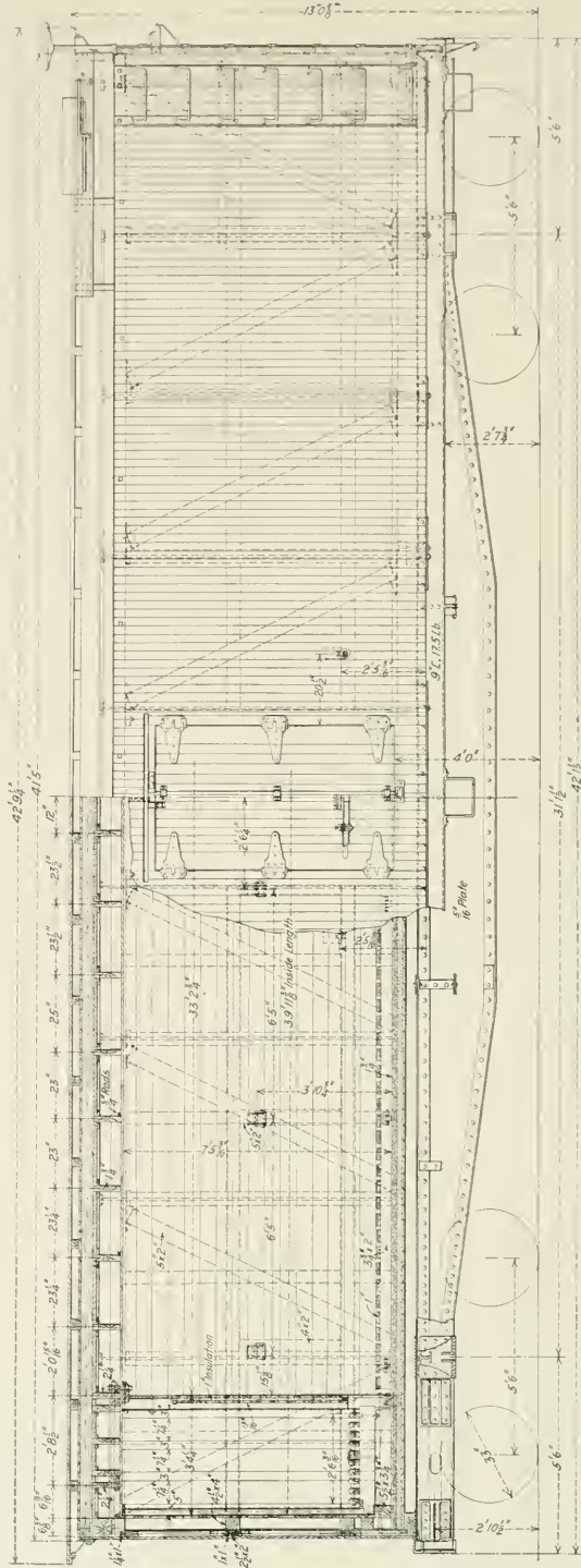
Elevation and Plan of U. S. R. A. Standard Refrigerator Car (Drawing No. 1386)
