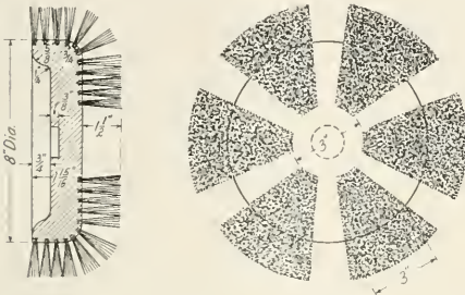
Rotary Brush Used for Car Cleaning
