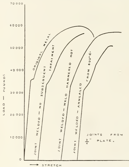
Stress-Strain Curves for Oxy-Acetylene Welded Joints.
