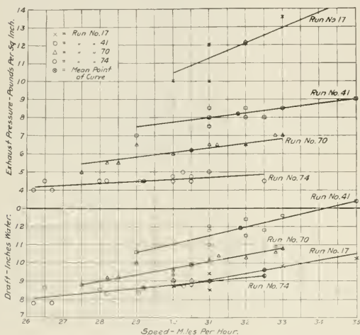
Fig. 24—Exhaust Pressure and Draft Diagrams for Runs 17, 41, 70 and 74, Showing Graphically the Improvement Effected in Draft Efficiency.
