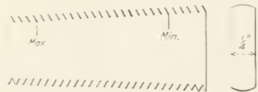
Fig. 7—Hardened Master Thread Gage
