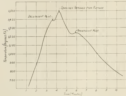
Fig. 1—Temperature Changes in a Piece of Steel Uniformly Heated and Allowed to Cool
