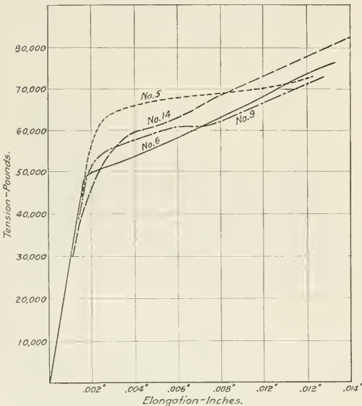
Fig. 7—Stress-Strain Curves For Zones C and D.
