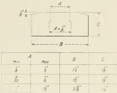
Fig. 4—Boiler Punch Dies Reduced to Three Sizes
