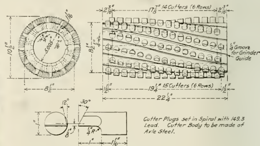
Fig. 8—Construction of Inserted Tooth Milling Cutter
