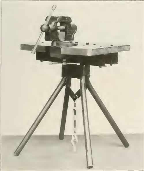
A Convenient Portable Vise
