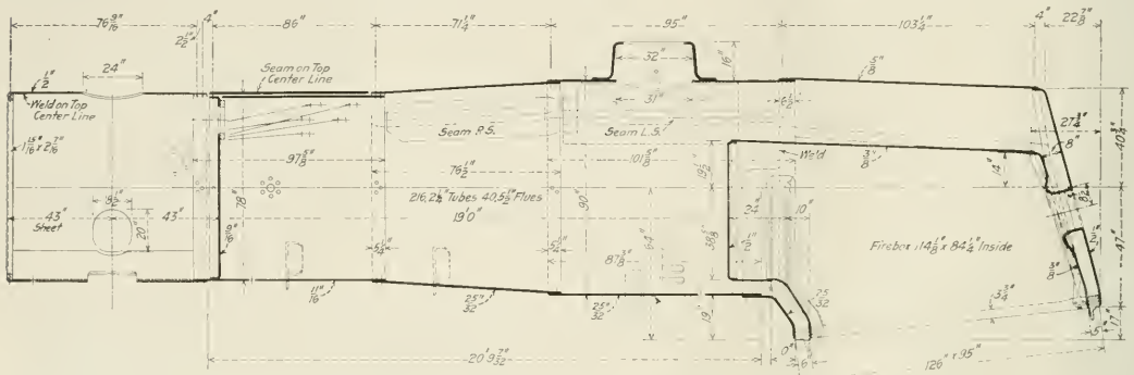
Boiler of the Railroad Administration Standard Light Mikado Type Locomotive
