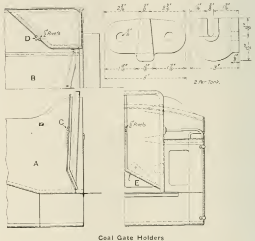
Coal Gate Holders
