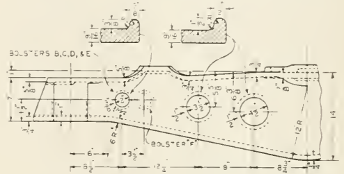
Fig. 6—Location of Holes in Sides of Bolsters "B," "C," "D," "E," and "F"
