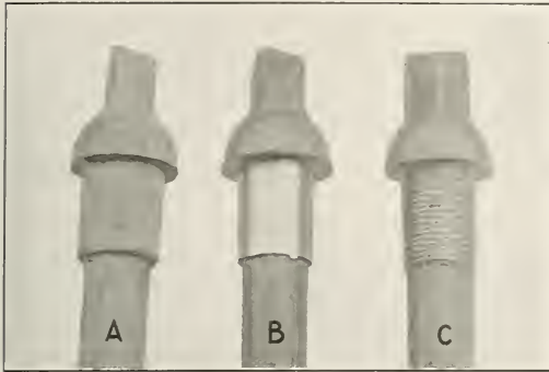
Fig. 7—Radial Staybolts Before and After Machining
