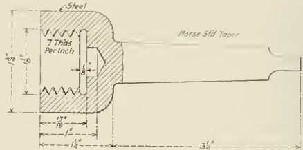
Fig. 4—Chuck for Holding the Cup or Spherical Grinder
