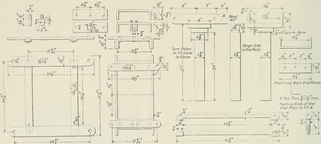
Fig. 4—Details of Universal Air Compressor Table
