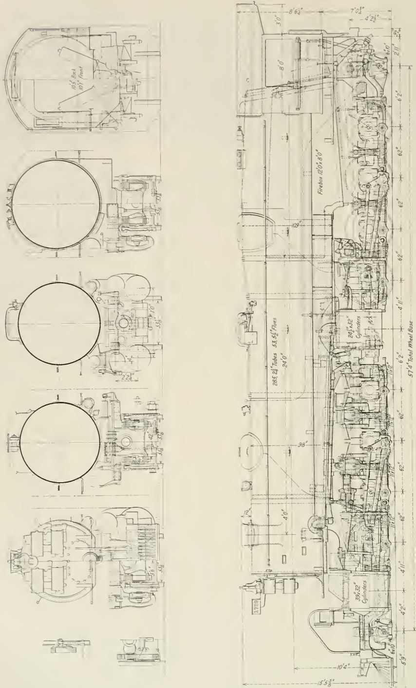
Elevation and Sections of the Norfolk & Western Mallet Locomotive
