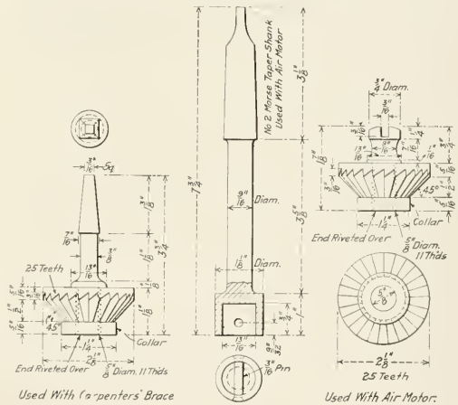
Fig. 2—Reamers for Superheater Header Seats
