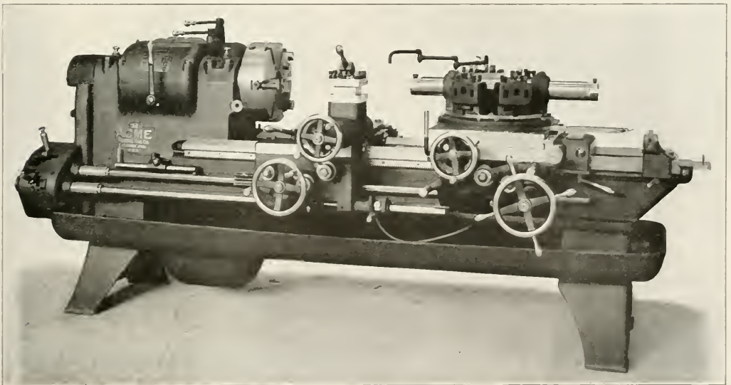
Fig. 1—Cincinnati Acme No. 3 Universal Flat Turret Lathe
