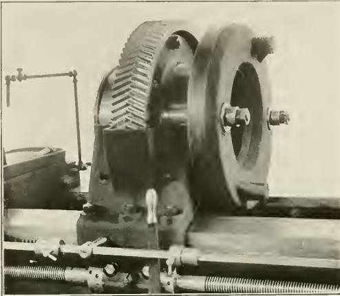
Fig. 2—The Herringbone Type Gear and Pinion Drive
