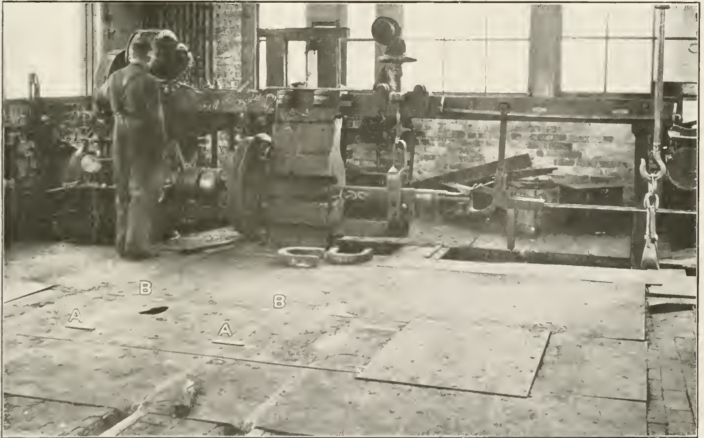
Fig. 1—Wheel Dismounting Press; Shifting Platform in the Foreground. Axle Carrier at the Right.
