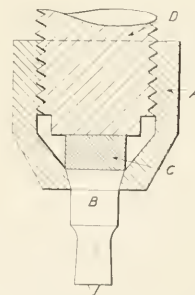
Fig. 3—Boiler Punch Holding Nut Arrangement
