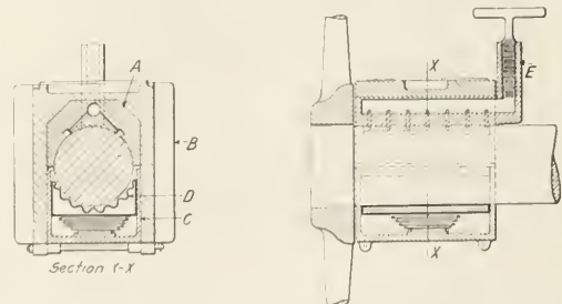
The Martin Truck Box Lubricator
