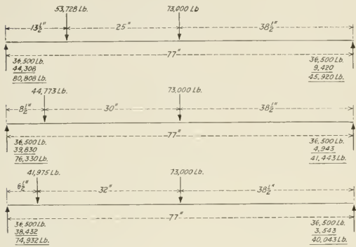
Fig. 4—Diagrams Showing the Reactions Due to Combined Vertical and Horizontal Forces
