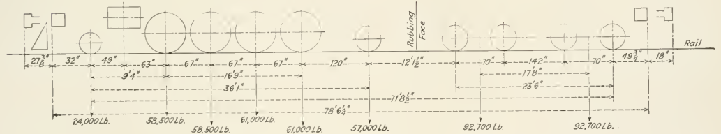
Heavy Mikado- Weight in Working Order. 10,000 Gal. Tender - Freight Trucks
