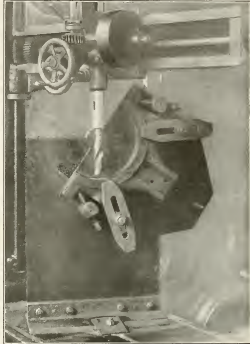
Fig. 2—Fixture for Holding Eccentric Straps
