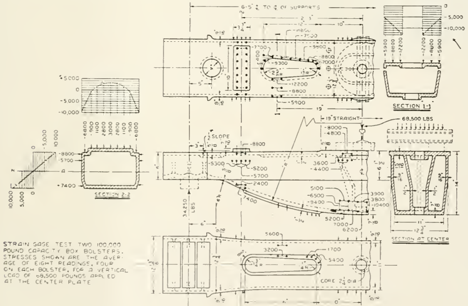
Fig. 13—Bolster "I" Under a 68,500 Lb. Load at the Center Plate
