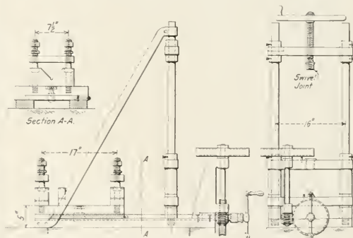
General Arrangement of Keyway Milling Machine
