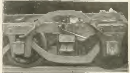
Fig. 1—Yoke for Use in Removing Elliptic Truck Springs
