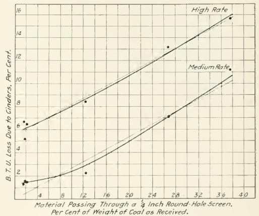
Fig. 2—The Cinder Loss in Relation to the Fine Material in the Coal
