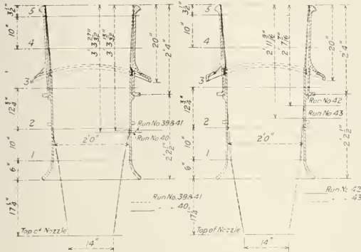
Fig. 9—Exhaust Stack Diagrams for Runs 39-41, 40, 42 and 43
