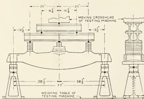
Fig. 2—Method of Combined Loading
