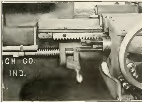
Fig. 3—Screw Cutting Attachment and Carriage Stops
