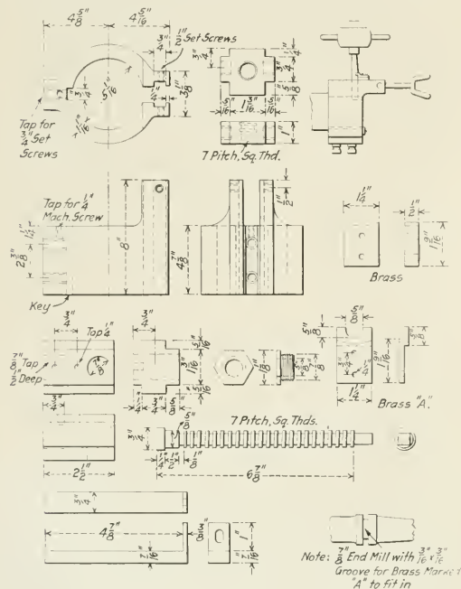
Details of Keyway Milling Attachment
