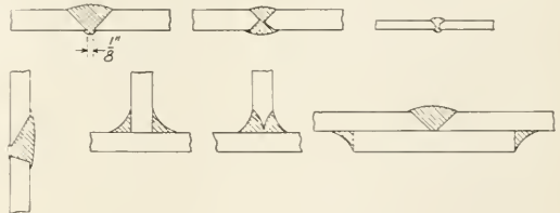
Fig. 1—Typical Arc Weld Scrap
