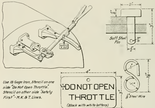
Safety Pin for Locking Throttle Levers
