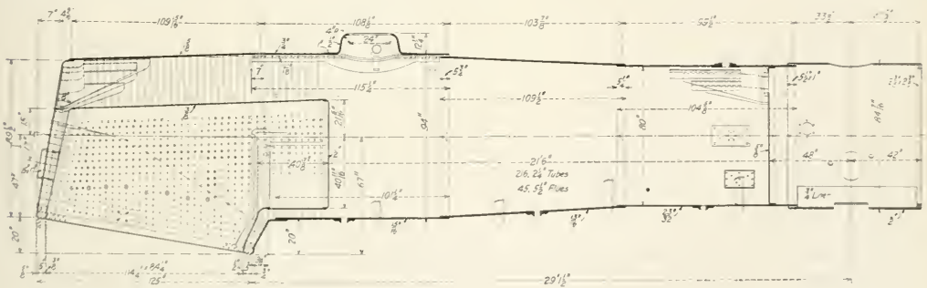
Sectional Elevation of the Boiler
