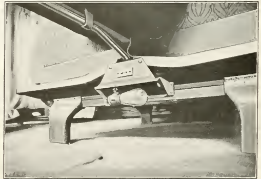
Arrangement of Aisle Light Under the Berth
