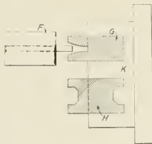
Fig. 6—Double Stroke Heading Dies
