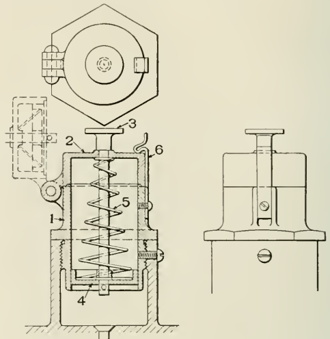
Automatic Hard Grease Cup
