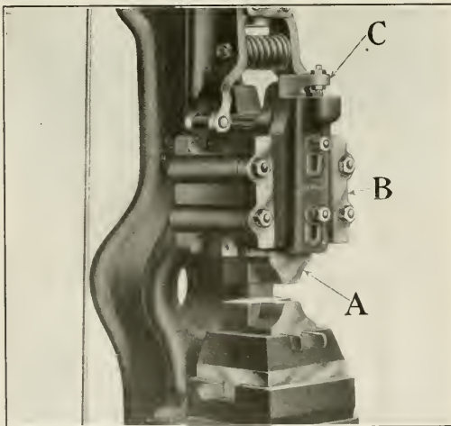
Power Hammer Attachment for Taking Up Wear
