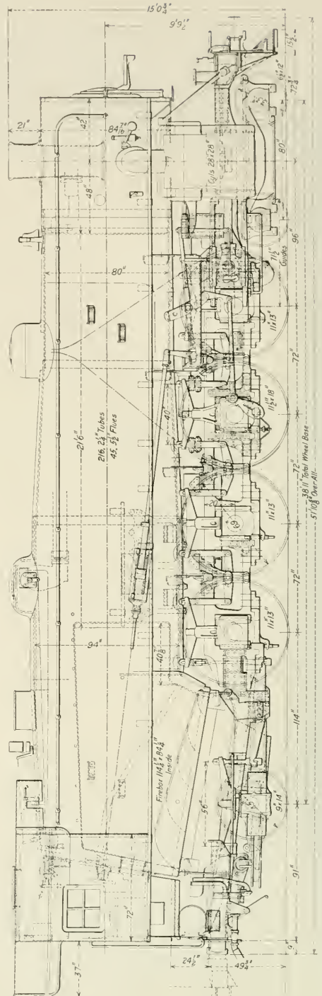
Elevation Showing the General Arrangement of the New York Central 4-8-2 Type Freight Locomotive
