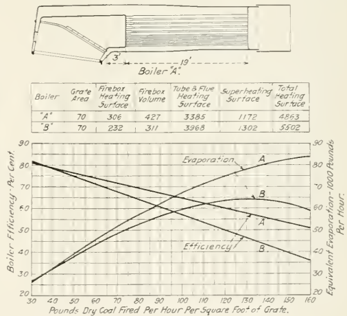
Fig. 2—A Comparison of the Rate of Actual Evaporation for Firebox and Tube Heating Surfaces in Relation to Rate of Combustion
