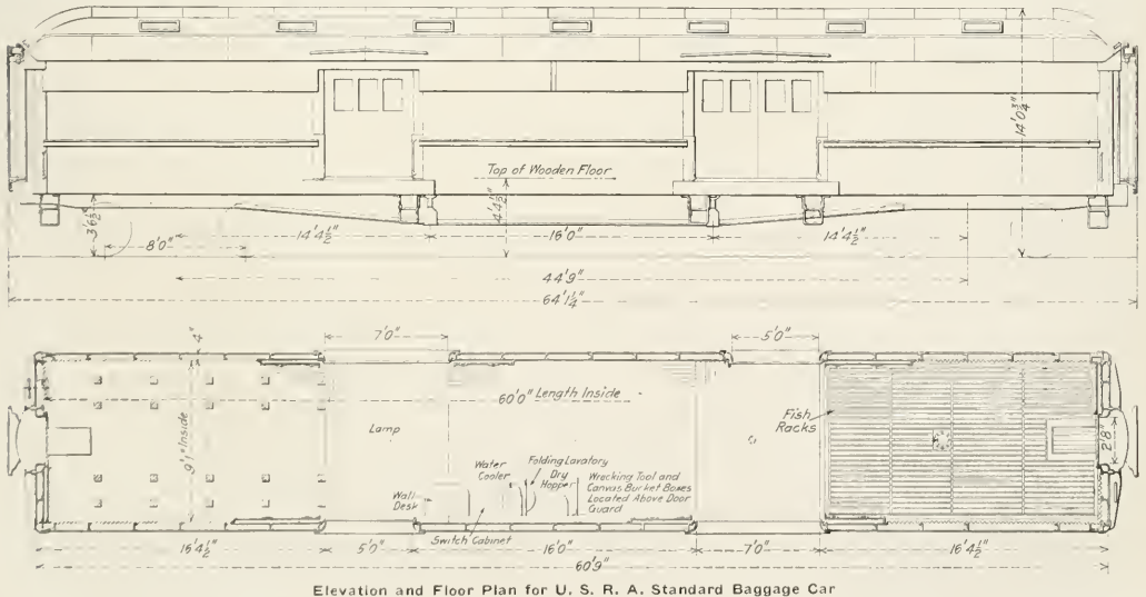
Elevation and Floor Plan for U. S. R. A. Standard Baggage Car
