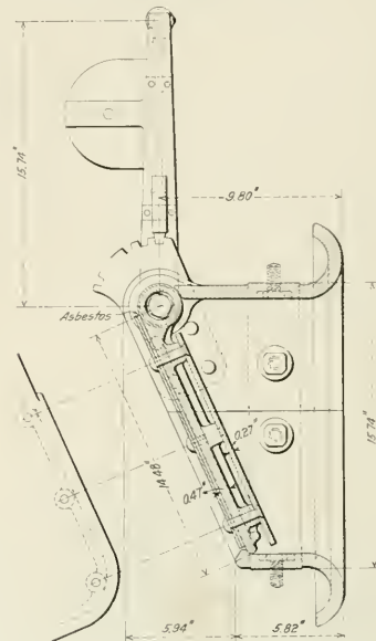
Inside—Opening Fire Door for the French Locomotives.
