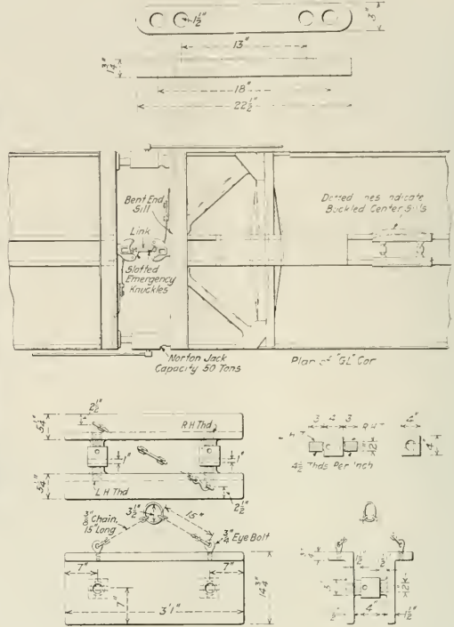
Method of Straightening Steel Car Sills Without Removal from the Car
