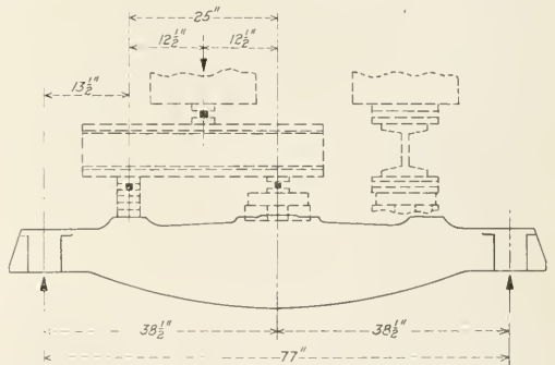
Fig. 11—Method of Loading Bolster for Test
