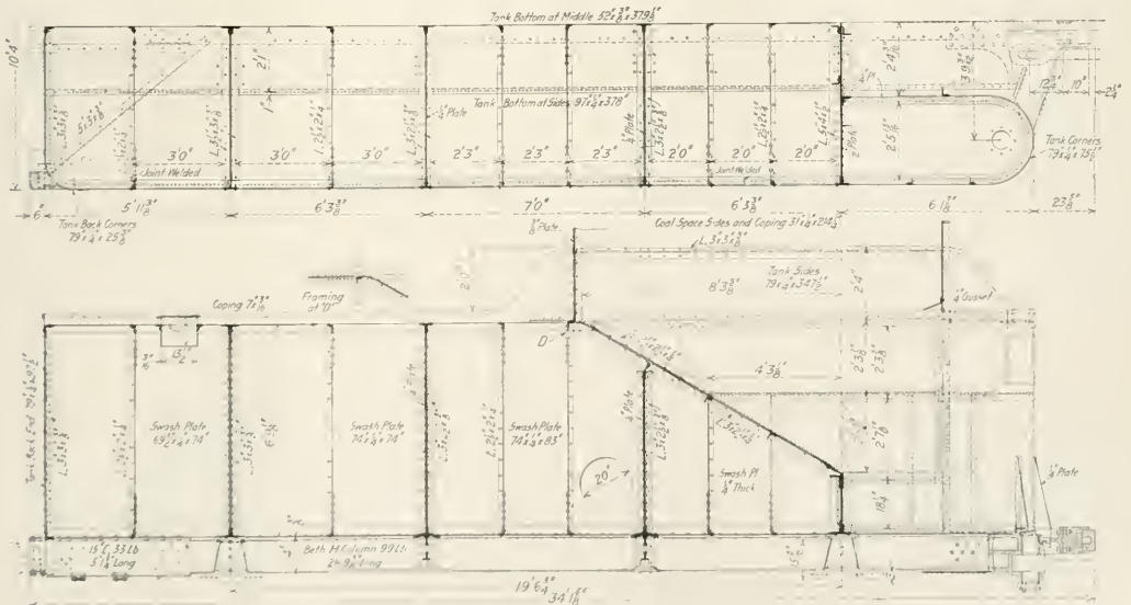
Elevation and Half Plan of the Tank
