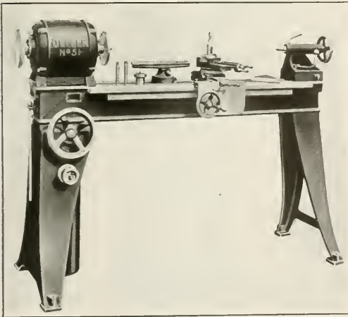
"Oliver" No. 51 Motor Head Speed Lathe
