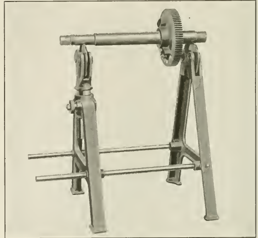
Stand Used in Balancing Pulleys, Fly-wheels, Etc.
