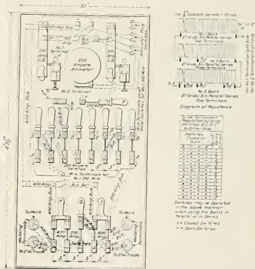
Two-Man Welding Panel.
