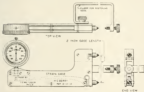
Fig. 1—Berry Strain Gage
