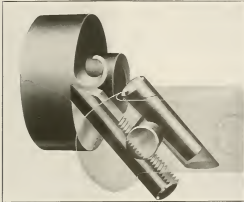
Lovejoy Positive Lock, Inserted Cutter, Turning Tool
