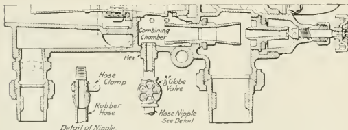
Water for the Sprinkler Hose Supplied from the Injector Combining Chamber
