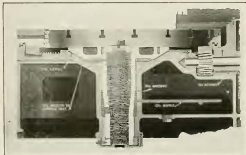
Fig. 3—Table Spindle and Oiling Arrangement
