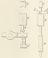
Fig. 4—Cold Heading Machine Arrangement
