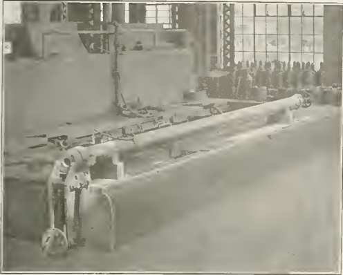
Fig. 1—Hydraulic Superheater Flue Tester
