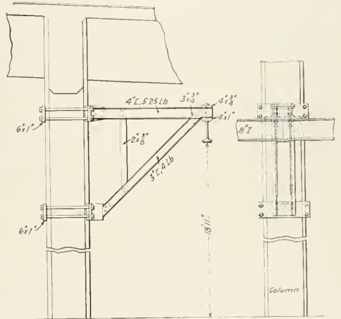
Trolley Hoist Track Supported from Enginehouse Columns
