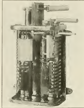
Master Controller with Case Removed
