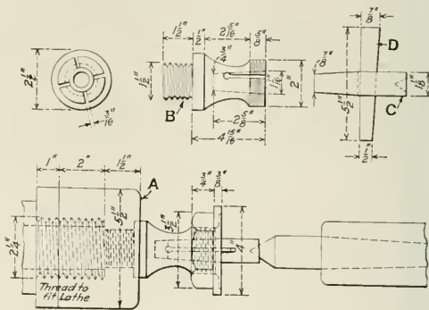
Method for Facing Nuts.
