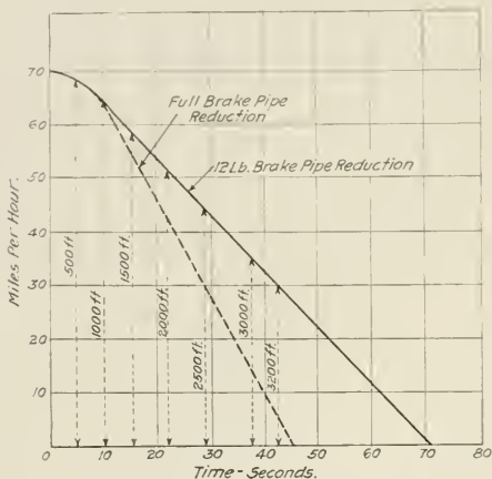
Fig. 6—Velocity-Time Curve for Deceleration
