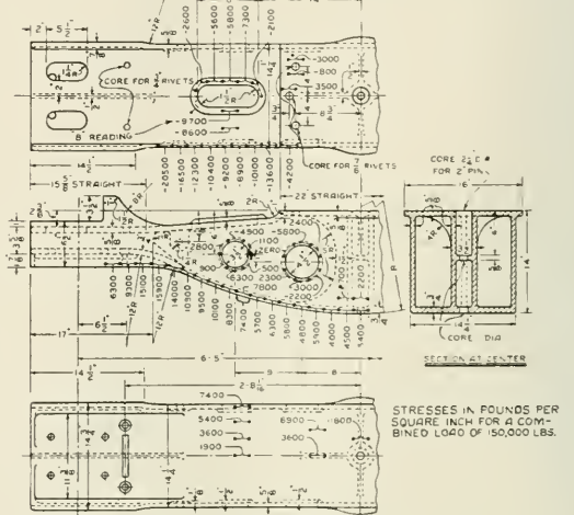
Fig. 11—Bolster "G"
