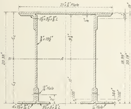
Section Used as Basis for Calculations
