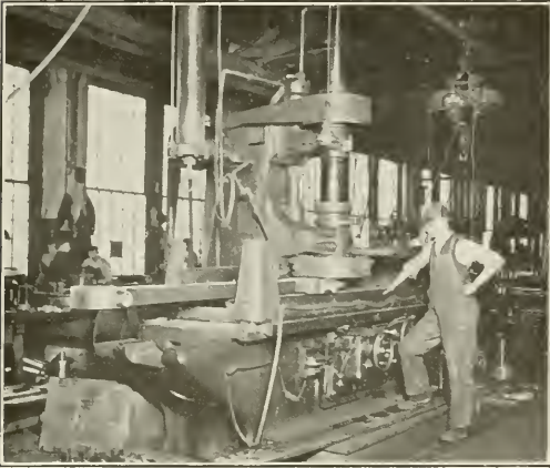
Fig. 4—Locomotive Side Rod Being Finished on a Surface Grinder
