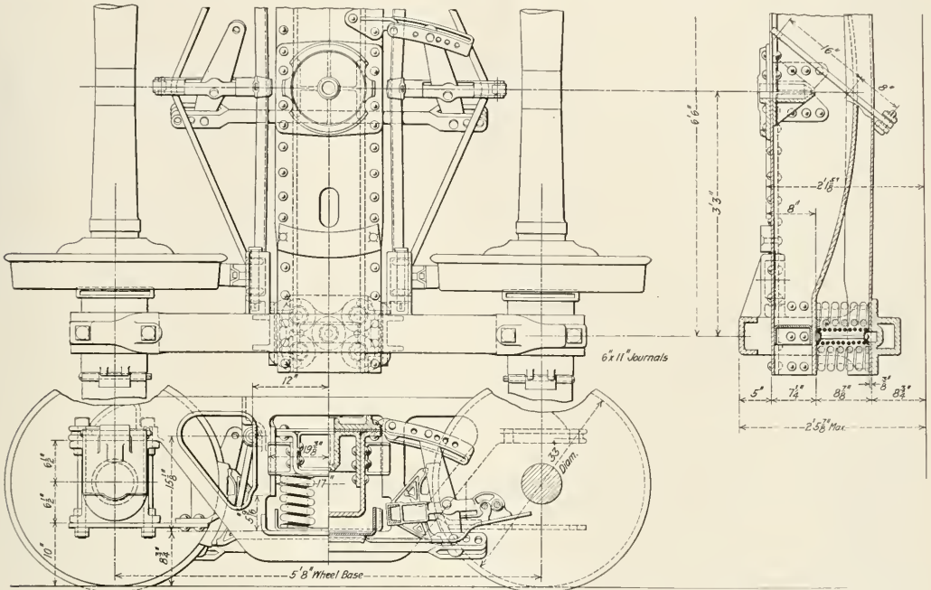
Fig. 21—General Plan of the Standard 70-Ton Truck
