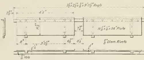
Construction of the Drop Doors
