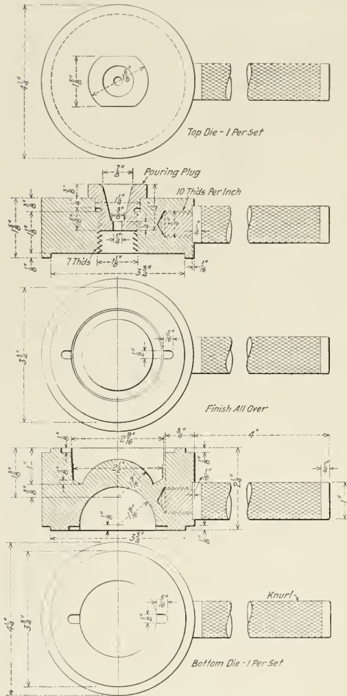
Fig. 3—Mold and Holder for Soft Metal Grinders
