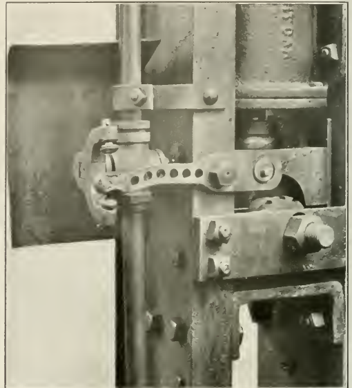
Fig. 5—Automatic Valve Used with Flue Swager
