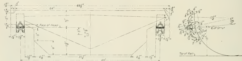
Fig. 25—Limiting Outline for the Standard Brake Beams
