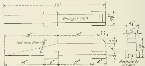
Wedge Blocks Used in the Place of Jacks for Raising Locomotives
