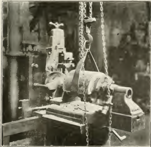
Fig. 2—Setting Brass in Draw Cut Shaper Fixture
