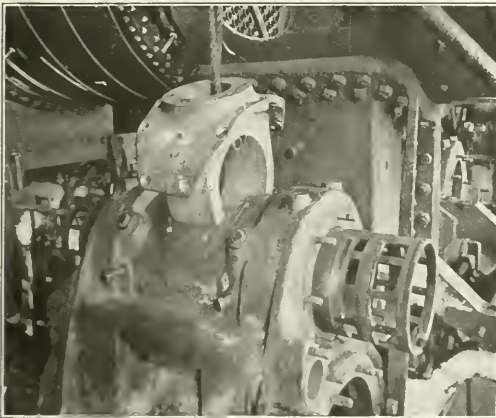
Fitting Yoke Casting to Steam Chest
