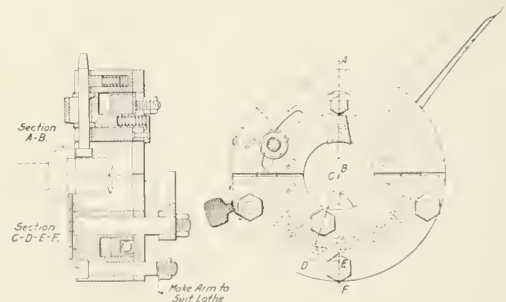
No. 2—Details of Hinged Self-Opening Die.
