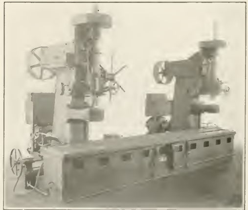
Baker Brothers 4-K Rod Drill
