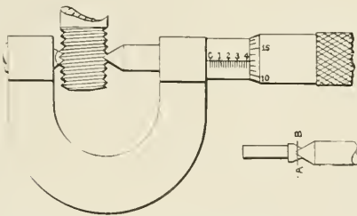
Fig. 1—Thread Micrometer Calipers
