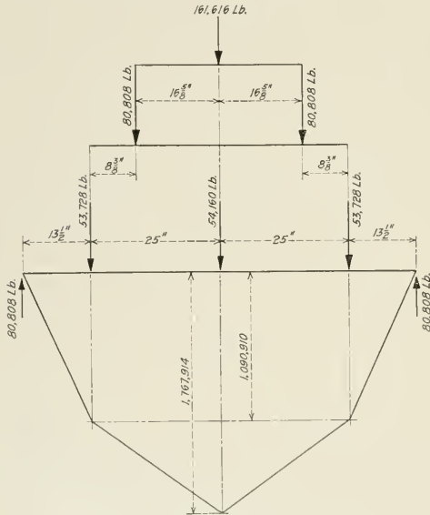
Fig. 12—Bending Moment Diagram Shown at 9, Fig. 5
