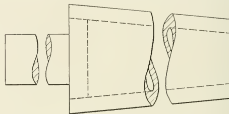
Fig. 3—Hollow Taper Gage for Large Holes
