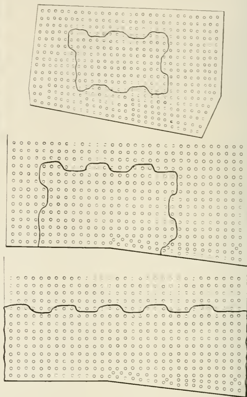
Fig. 2—Serpentine Seams as Applied to Patches and Half Side Sheets
