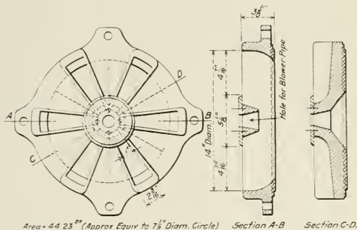
Fig. 13—Plain Annular Nozzle A-4a
