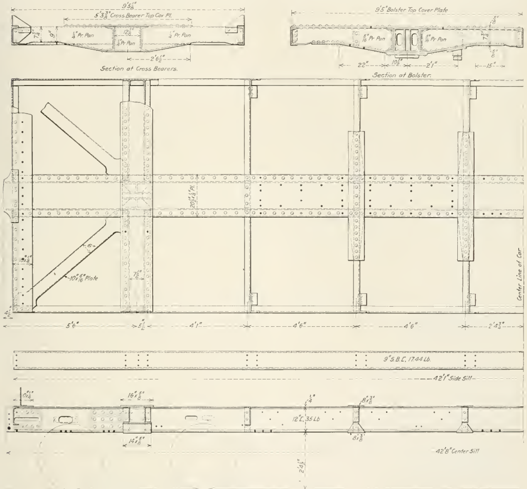
Fig. 12—Underframe for the 50-Ton Composite High Side Gondola
