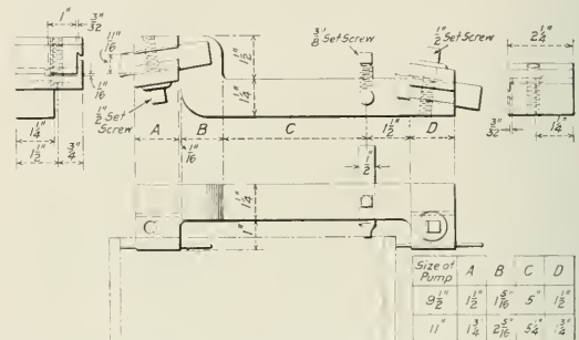
Tool Which Cuts Off and Faces Piston Rings.
