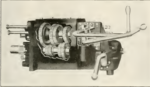
Fig. 5—Primary Speed Change Case
