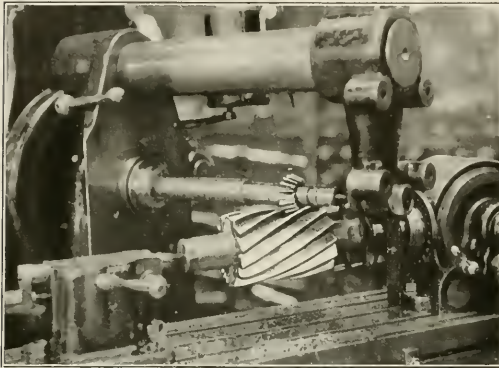
Fig. 5—Recutting a Worn Milling Cutter
