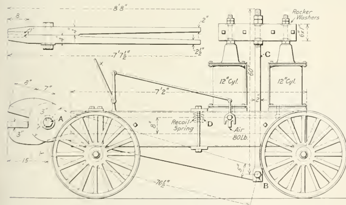
Portable Alligator Shears for Cutting Scrap
