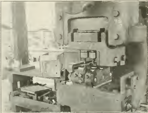
Fig. 16.—Gang Punch for Tie Plates
