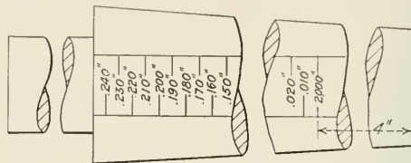
Fig. 2—Taper Gage for Small Holes
