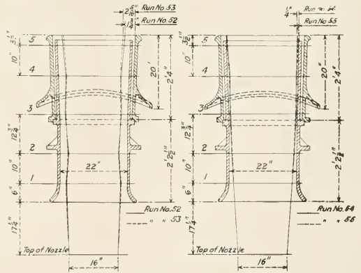
Fig. 15—Exhaust Stack Diagrams for Runs 52, 53, 54 and 55
