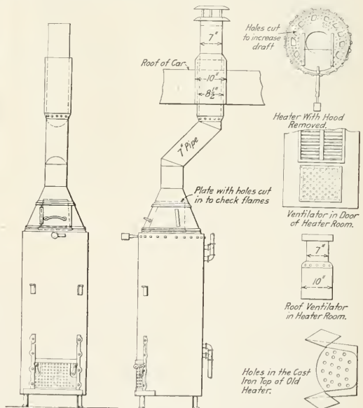
Fig. 2—Changes Made in Baker Heaters to Burn Soft Coal
