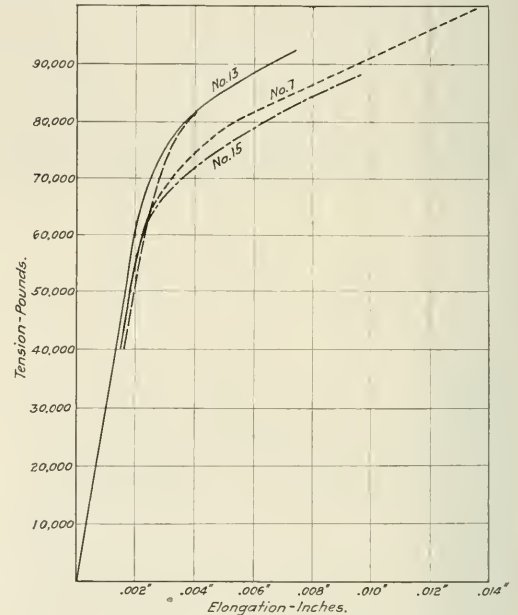
Fig. 8—Stress-Strain Curves For Zone B.
