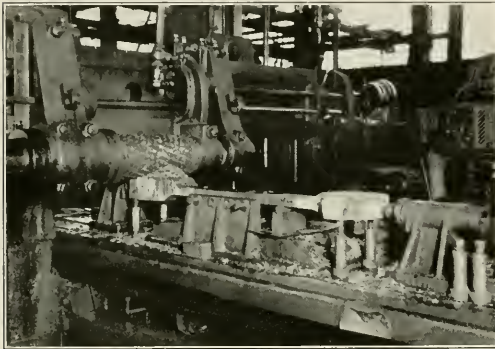
Fig. 8—Milling Side Rods
