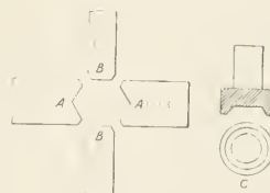
Fig. 2—Heading Dies Used with Hammer Header
