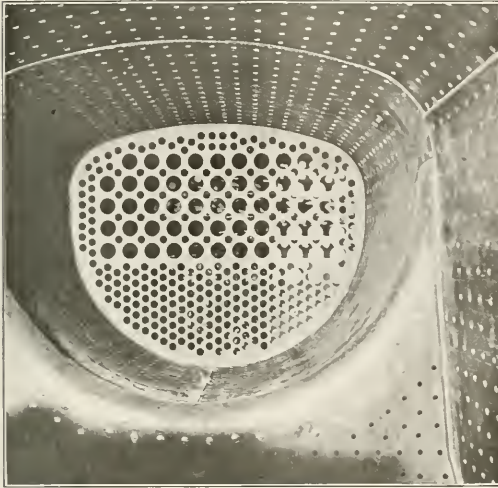
Electrically Welded Firebox Seams
