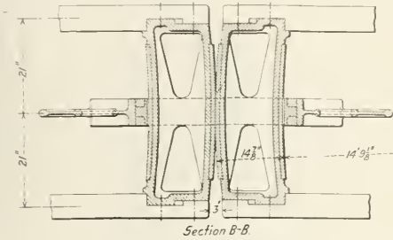
Section Plan of the Curved Bumper Castings and Articulating Link
