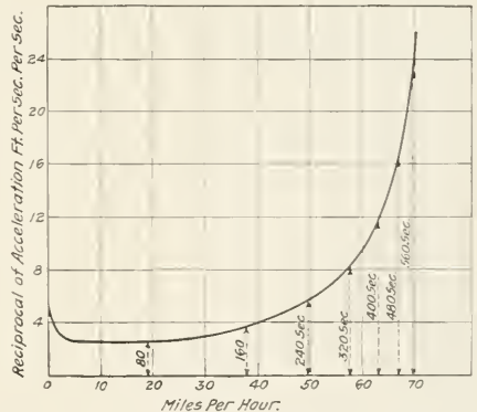
Fig. 2—Time Required to Accelerate to Various Speeds
