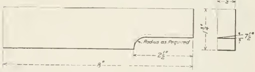
Fig. 11—The Corner Rounding Tool
