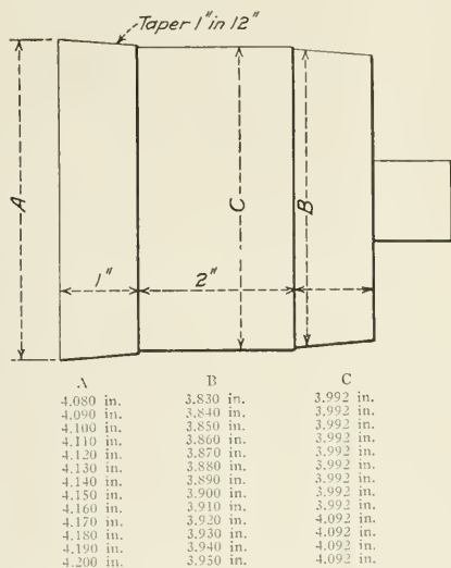
Fig. 7—Suggested Sizes for Side Rod Knuckle Pins
