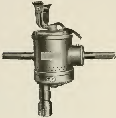
Fig. 1—Portable Electric Drill
