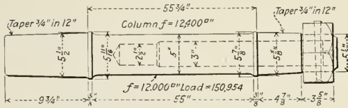
Fig. 3—Design of Piston Rod of Annealed Carbon-Vanadium Steel for 2-10-2 Type Locomotive
