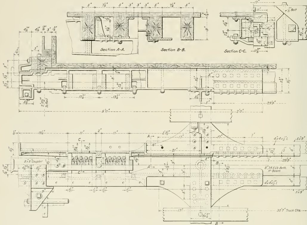
Details of Draft Arm and Bolster
