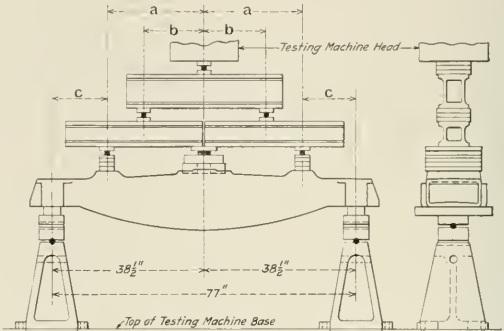
Fig. 13—Proposed Method of Testing Bolsters
