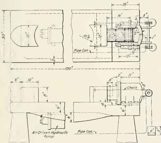
Self Contained Hydraulic Press for Shortening Drawbars
