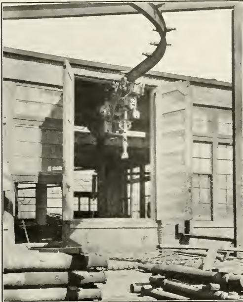
Fig. 5—Overhead Monorail Crane Serving Shop and Storage Platform
