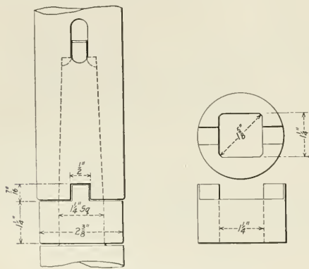
Collar Used for Driving Large Drills
