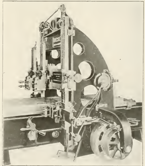
Fig. 3—Arrangement of Driving Pulleys and Operating Levers
