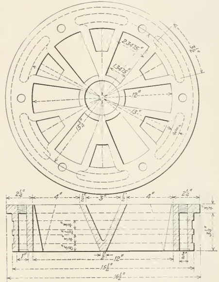
The Annular Ported Exhaust Tip
