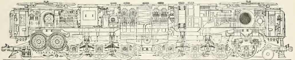
Longitudinal Section of the Pennsylvania Electric Locomotive
