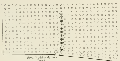
Fig. 1—Method of Reinforcing Welded Cracks
