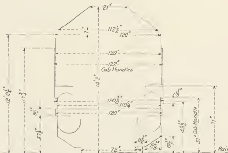
Six-Wheel Switcher- For Loaded Engine. For Light Engine, Heights Will Be About \frac{1}{2} Greater.
