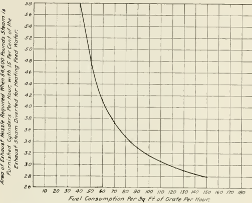
Fig. 2—Area of Nozzle in Square Inches for Various Rates of Combustion
