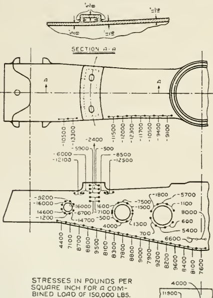
Fig. 9—Bolster "E"
