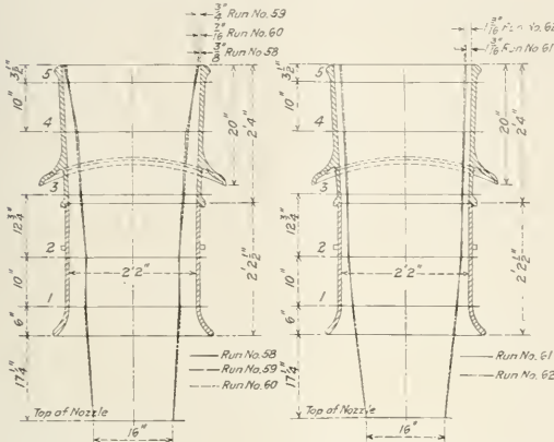
Fig. 22—Exhaust Stack Diagrams for Runs 58, 59, 60, 61 and 62
