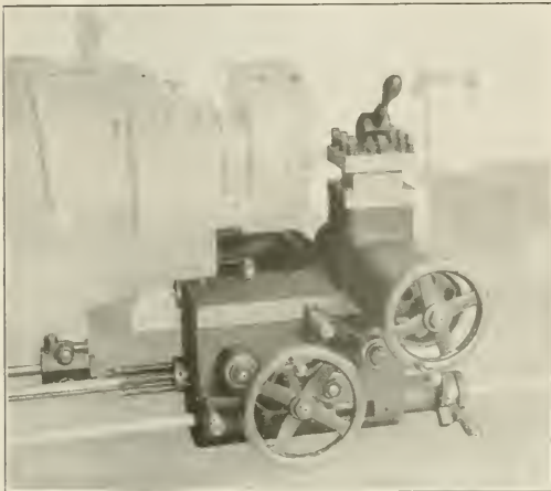
Fig. 2—Sliding Carriage Showing Apron and Independent Stops
