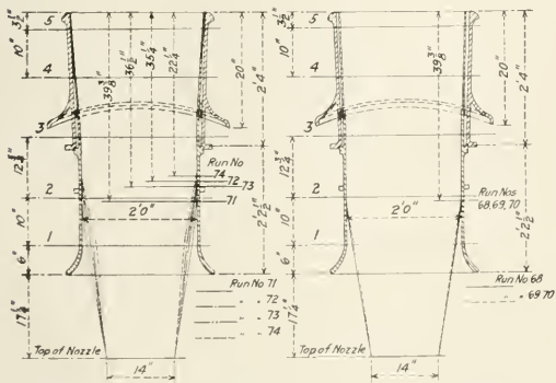
Fig. 11—Exhaust Stack Diagrams for Runs 68, 69-70, 71, 72, 73 and 74
