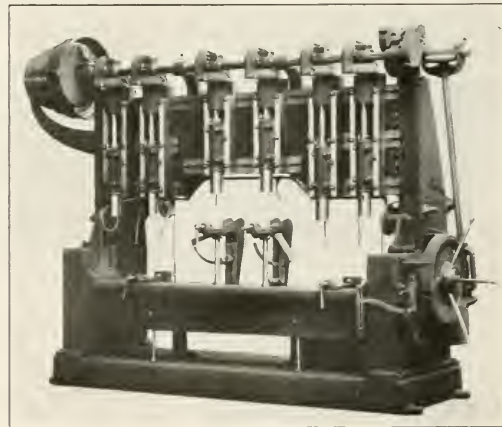
Foot-Burt Six Spindle Arch Bar Drilling Machine.
