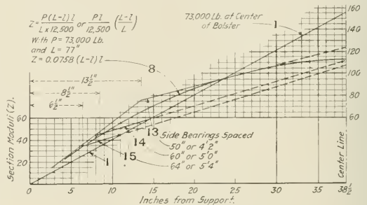
Fig. 9—Section Modulus Diagram
