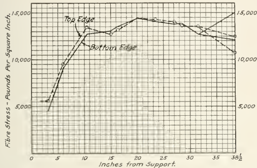
Fig. 14—Curves Showing Calculated Values of Bolster Stresses
