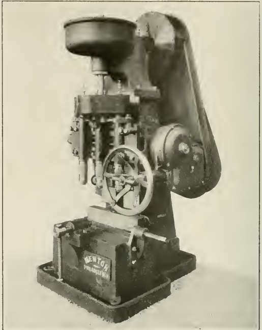
Newton Three Spindle Rail Drilling Machine.
