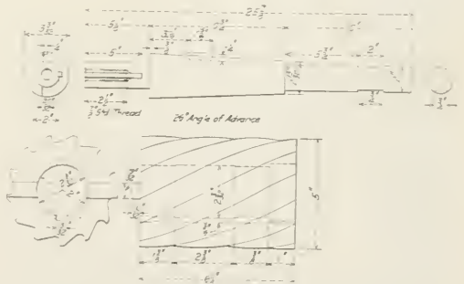
Fig. 4—Details of Milling Cutter for Vertical Machine
