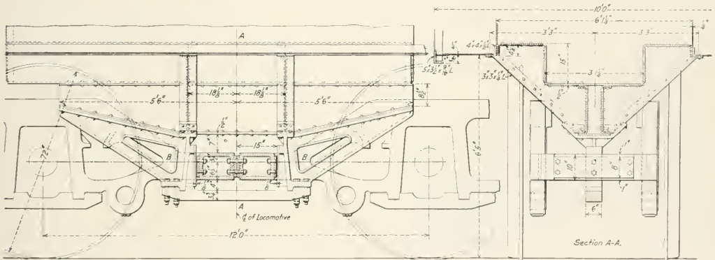
The Articulating Device—Pennsylvania Electric Locomotive
