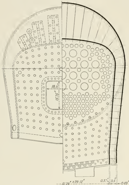
Back Head and Section Through the Firebox
