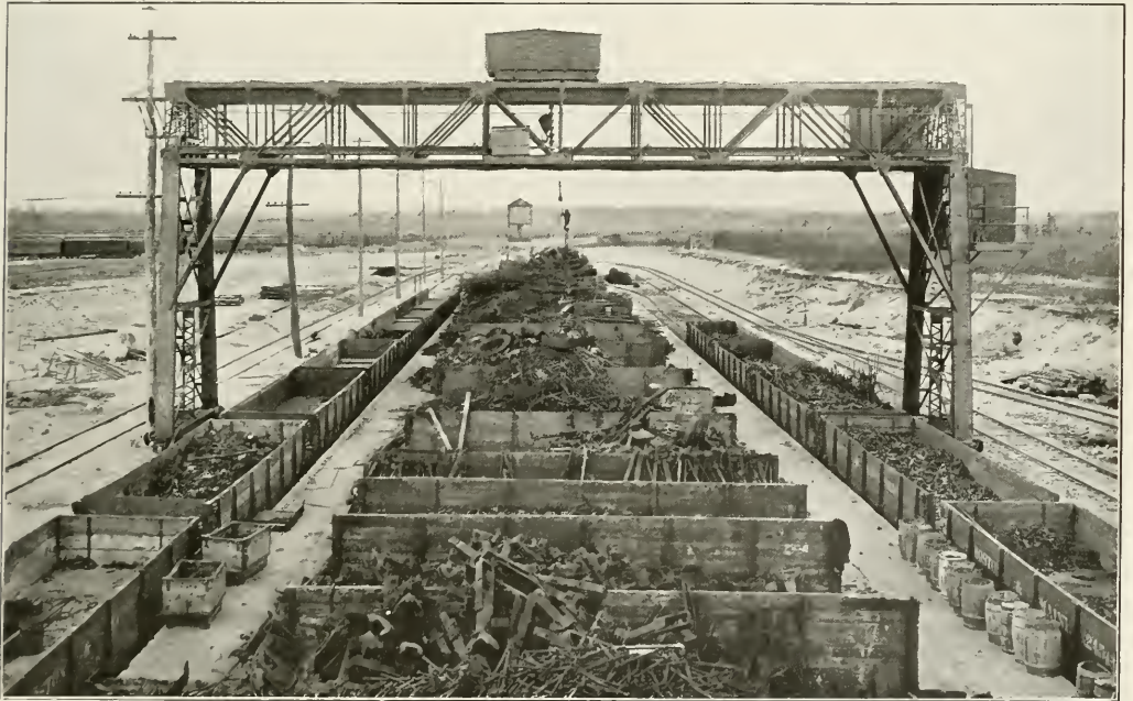
Scrap Dock with Gantry Crane—Boston & Maine Reclamation Plant
