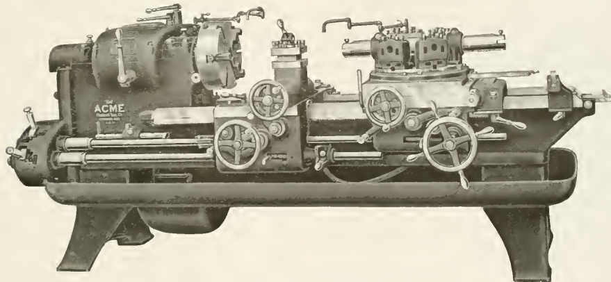
Cincinnati Acme Flat Turret Lathe
