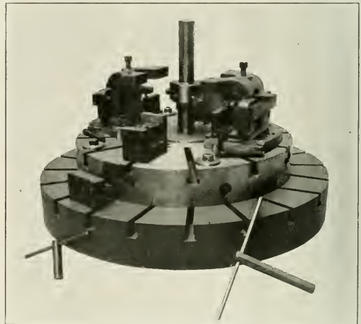
Fig. 10—Special Chuck Used on Gisholt Machine
