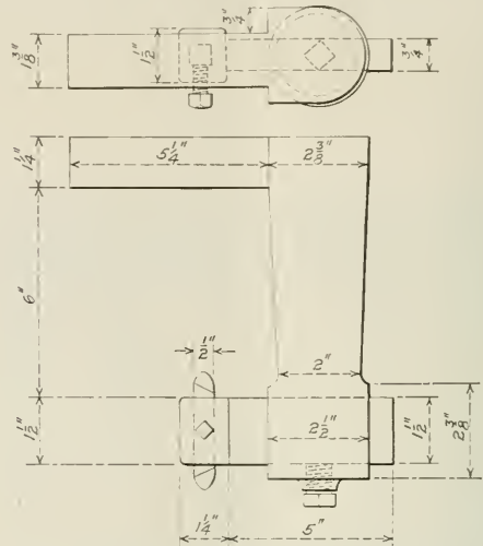
Tool Which Cuts the Time for Machining Crossheads
