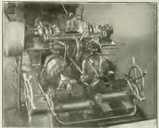
Fig. 6—Radial Staybolt Cutter
