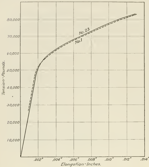
Fig. 6—Stress-Strain Curves For Original Material.
