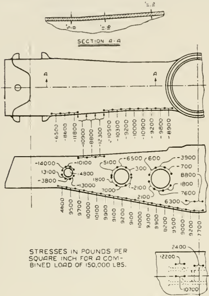
Fig. 8—Bolster "D" without Side Bearing
