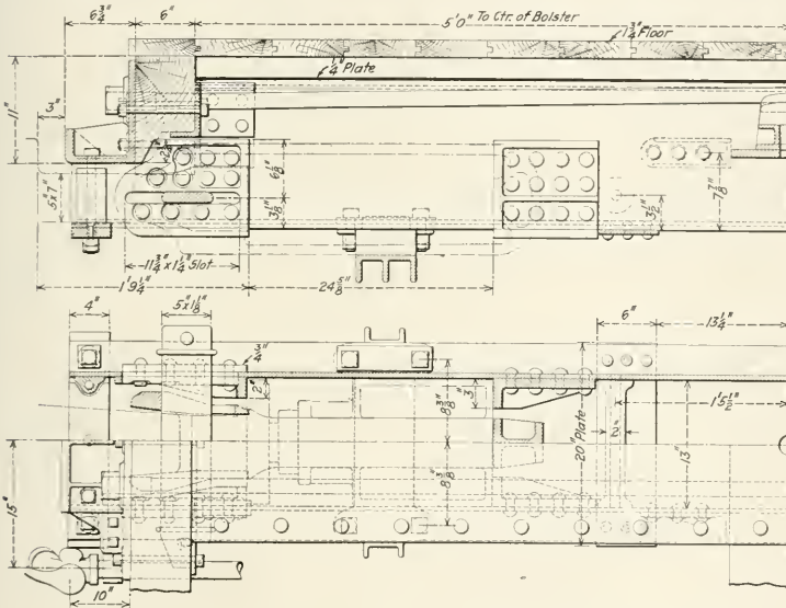
Details of Center Sills and Draft Attachments
