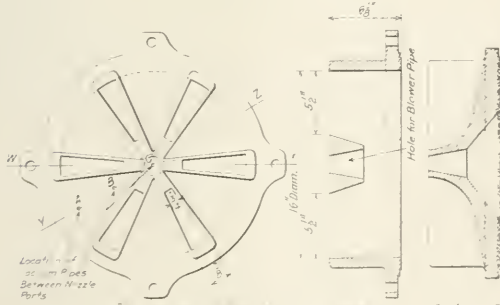
Fig. 18—Plain Annular Nozzle A-6, Showing Location of Vacuum Gages Between the Ports
