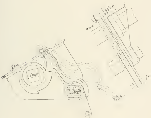
Hopper Door Operating and Locking Device
