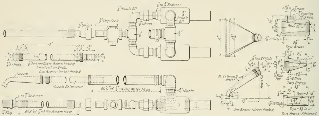
A Simple Shop-Made Vacuum Cleaner
