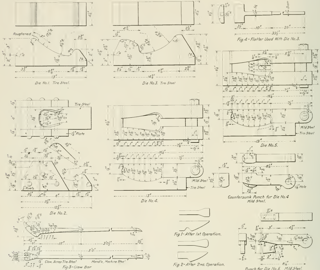
Dies Used In Making Claw Bars
