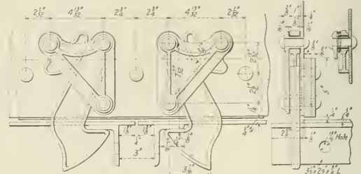
The Drop Door Latch and Lock
