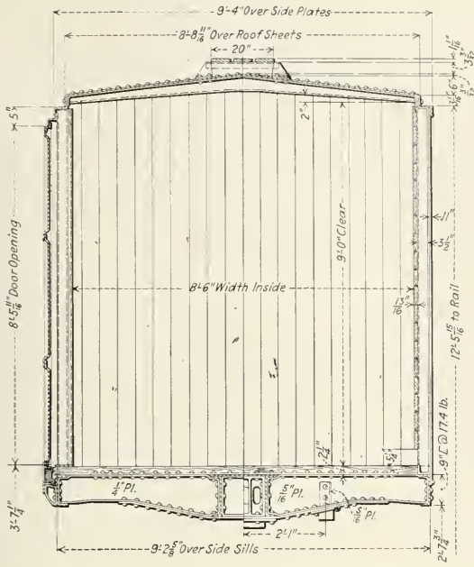
Section and End Views of the Standard Steel Box Car
