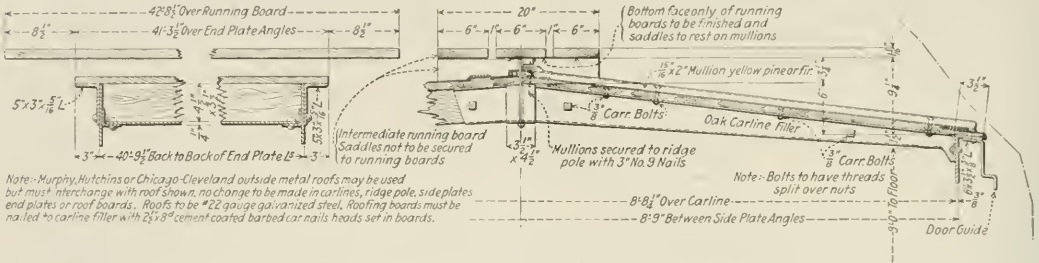
Fig. 6—Roof Construction for the Standard Box Cars
