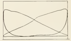
Fig. 2—Representative Indicator Cards, Union Pacific 2-10-2 Type Locomotive
