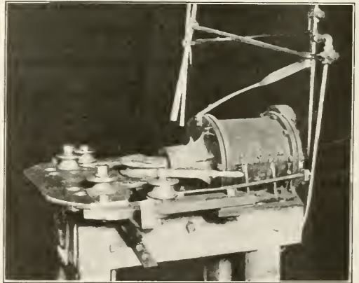
A Pipe Bender Designed for Car Work
