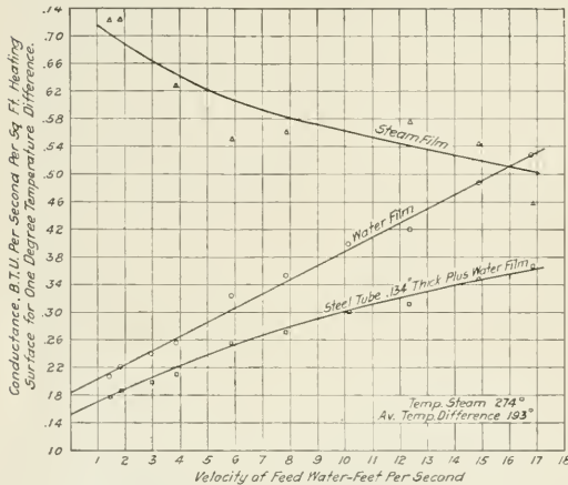
Fig. 8—Conductance Curves for Waste Gas Heater Tubes
