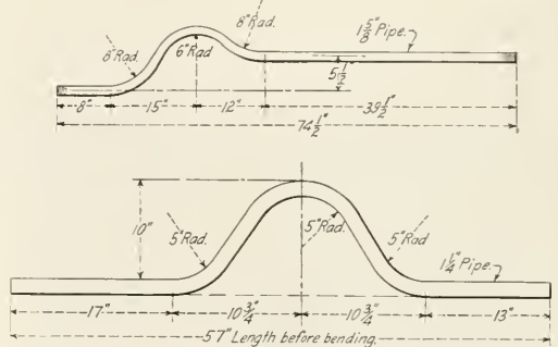
Parts Formed in One Operation on Pneumatic Pipe Bender
