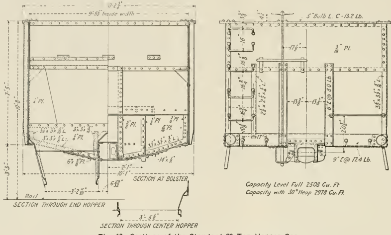
Fig. 19—Sections of the Standard 70-Ton Hopper Car
