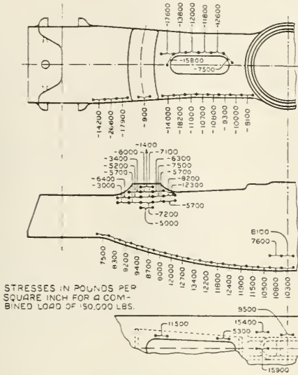
Fig. 4—Stresses in Bolster "A"
