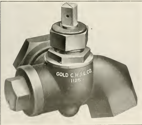
End Valve with Automatic Condensation Drip Port
