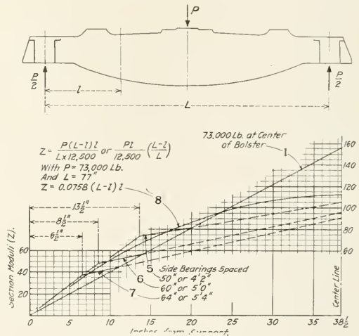
Fig. 3—Section Modulus Curve
