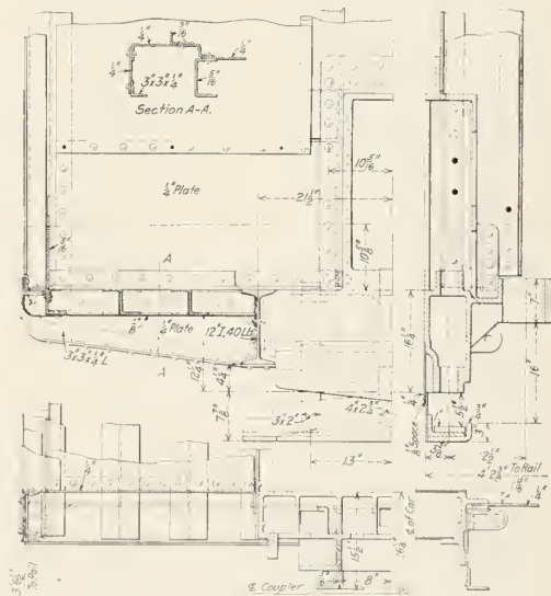
Platform Arrangement—Built-Up Construction
