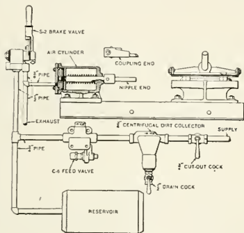
Fig. 1—Hose Mounting Machine
