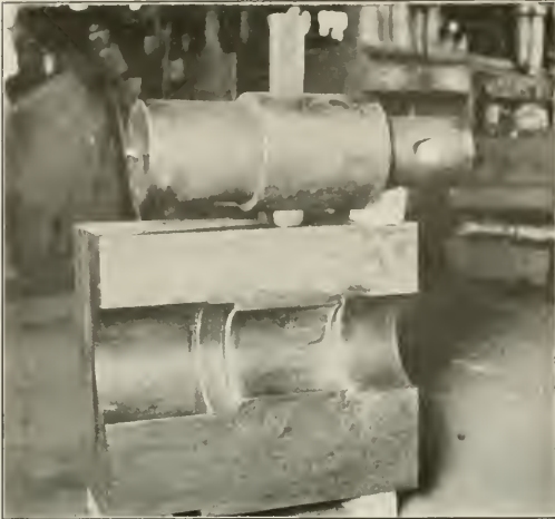
Dies Used for Forming the Ends of the Axles
