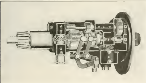
Fig. 6—Secondary Speed Change Case
