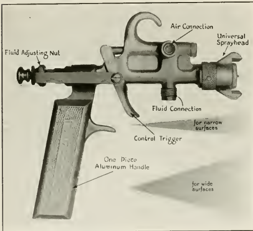
Fig. 1—Paint Spraying Nozzle.
