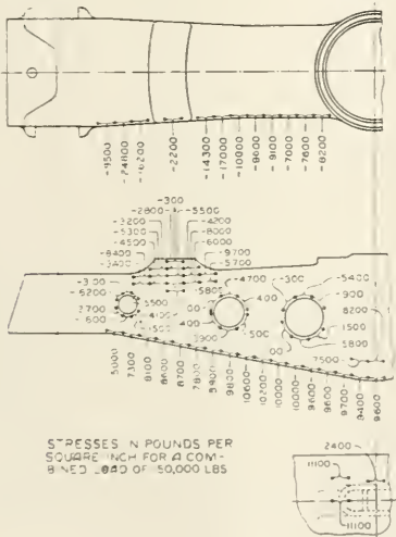
Fig. 5—Bolster "B"
