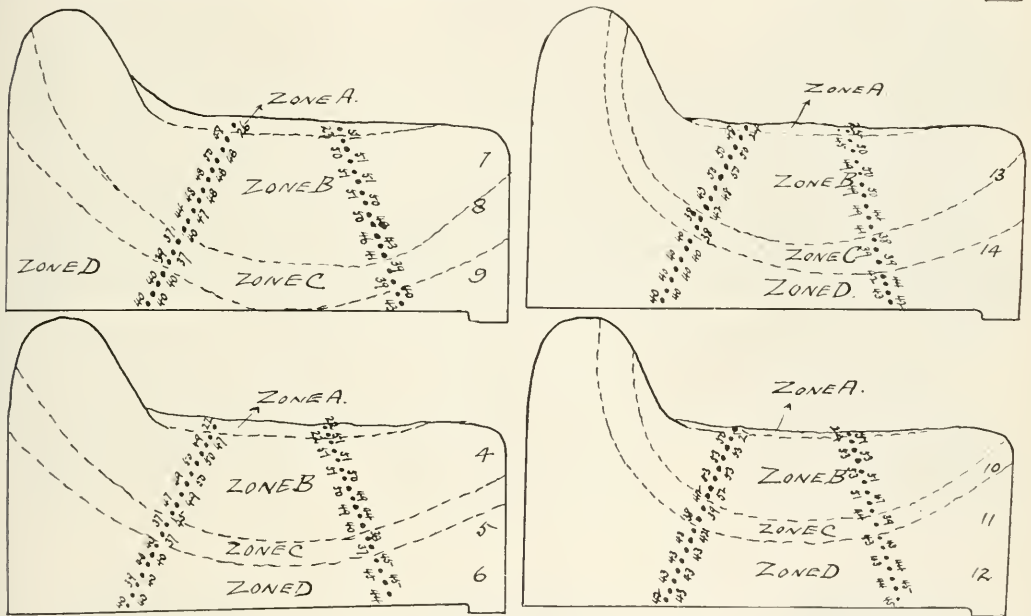
Fig. 9—Limits of Zones Determined by Hardness Tests.
