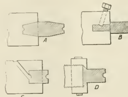
Fig. 3—Methods of Holding Dies
