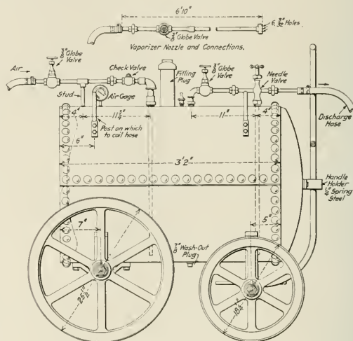
Locomotive Fire Kindler
