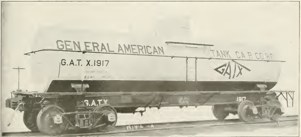
Class III—Tank Car Built According to MCB 1917 Specifications
