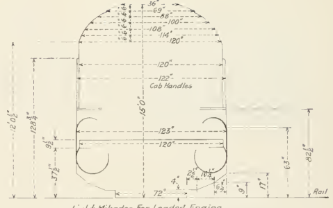
Light Mikado- For Loaded Engine. For Light Engine, Heights Will Be About \frac{1}{2} Greater.
