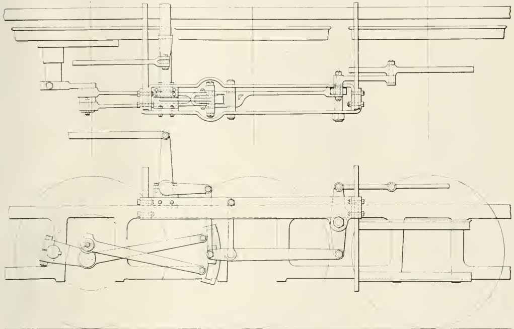
Fig. 2—Plan and Elevation of Anderson Valve Gear
