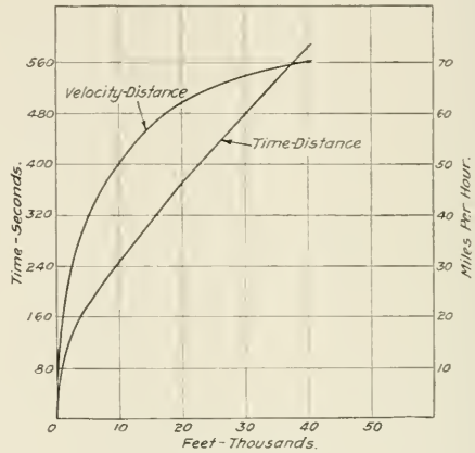
Fig. 4—Time-Distance and Velocity-Distance Curves for Acceleration
