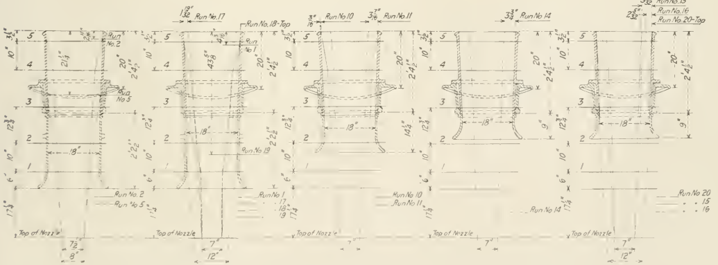
Fig. 5—Exhaust Stack Diagrams for Runs 1, 2, 5, 10, 11, 14, 15, 16, 17, 18, 19 and 20
