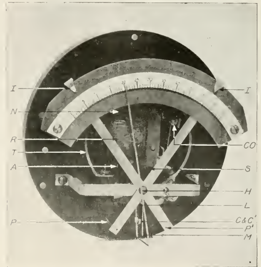
Fig. 1—Internal Mechanism for a Pressure Governor
