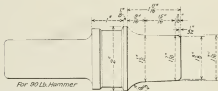
Combination Mandrel and Flaring Tool. For 2" Flues. Back End.
