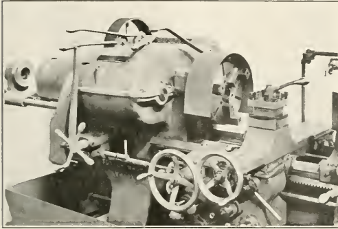
Fig. 2—Lathe Head, Cross Slide and Carriage
