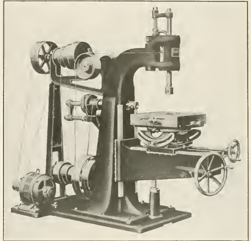
Oliver No. 75 Wood Milling Machine
