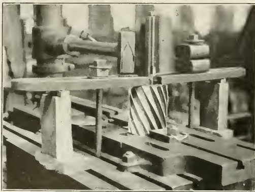
Fig. 6—Putting Arbor Keyway in Cutter
