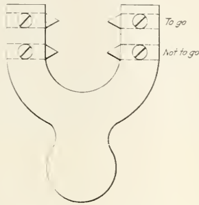
Fig. 5—A Convenient Form of Adjustable Thread Gage
