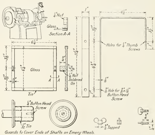
Safety Devices for Grinding Wheels Used on the North Western
