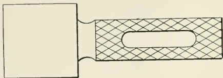
Fig. 1—Standard Plug Gage
