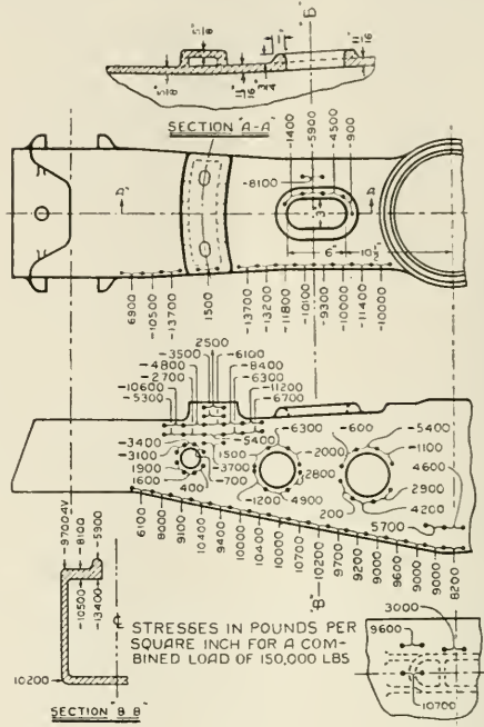
Fig. 10—Bolster "F"
