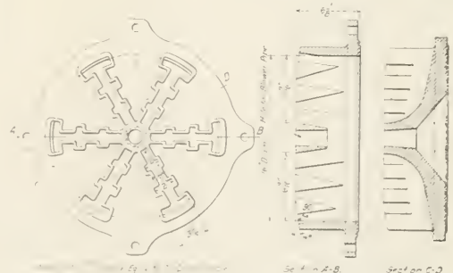
Fig. 19—Waffle Iron Nozzle A-8
