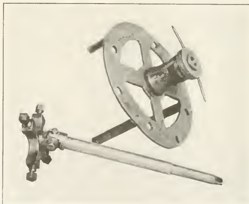
Device for Grinding Superheater Joint Rings
