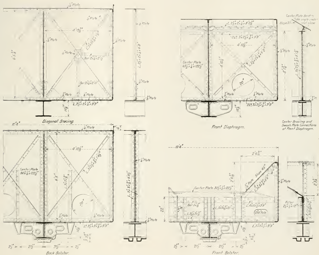
Sections Showing the Tender Bolster and Diaphragm Construction
