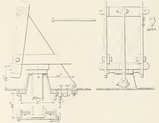
Fig. 2—Air Compressor Table Assembled
