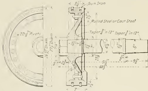
Pistons for the U. S. Standard Heavy Mikado Locomotive.
