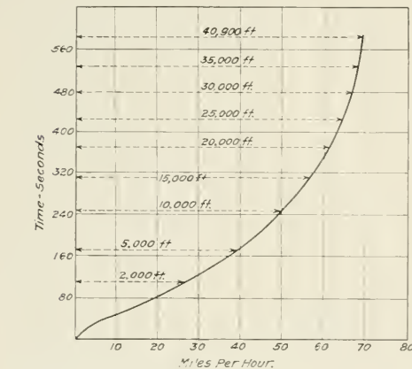
Fig. 3—Time and Distance Required to Reach a Given Speed
