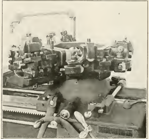
Fig. 4—Hexagon Turret and Saddle with Bar Tools
