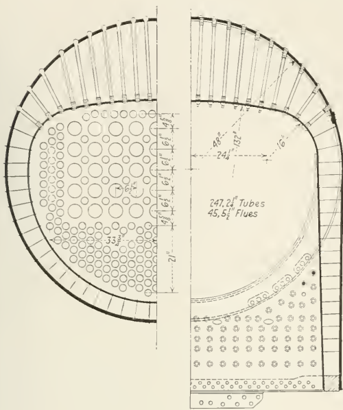
Sections Through the Combustion Chamber and Firebox
