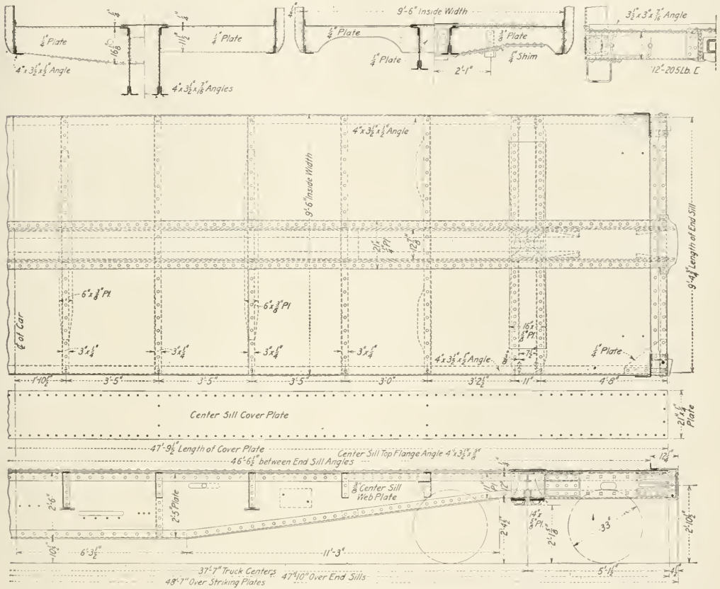
Fig. 16—Underframe for the 70-Ton Steel Gondola Car
