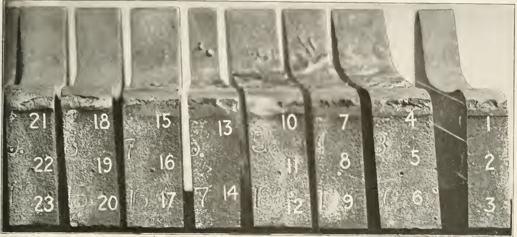
Fig. 3.—Sections Cut From the Tire for Test.
