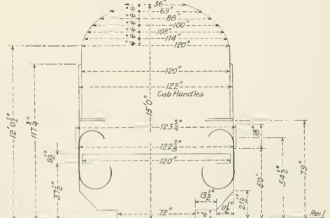
Eight-Wheel Switcher- For Loaded Engine. For Light Engine, Heights Will Be About \frac{1}{2} Greater.
