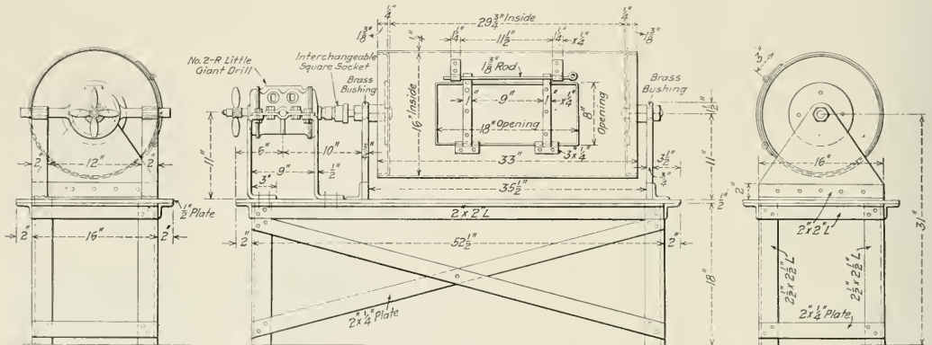
Flexible Staybolt Cap Rattler.
