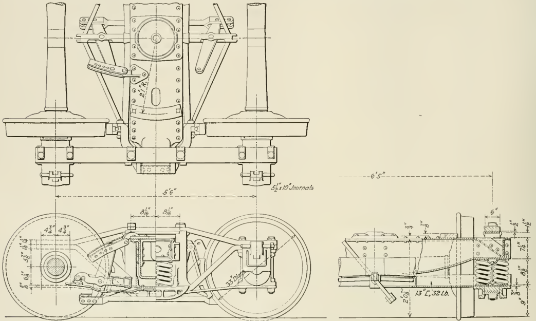
Fig. 20—General Plan of the Standard 50-Ton Truck
