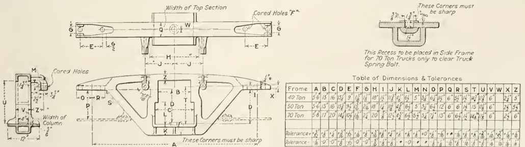
Fig. 22—Limiting Dimensions for the Cast Steel Truck Side Frames
