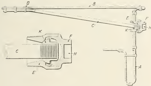
Boiler Brace Coupling
