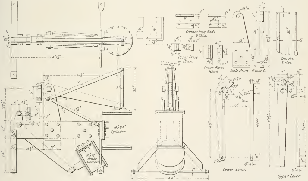
A Machine for Applying Bands to Locomotive Springs
