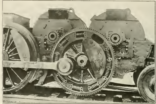
Motor and Jack Shaft Mounting
