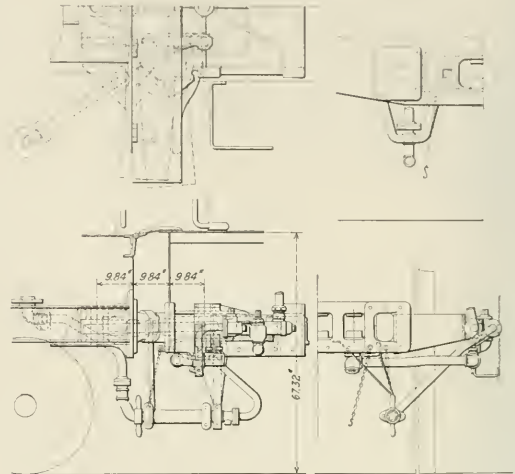
Details of the Engine and Tender Connection.
