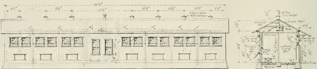
Side Elevation and Section with Partitions Removed—Columbus Welding Shop
