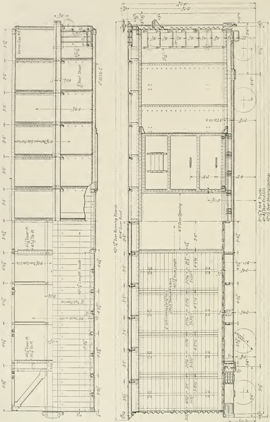
General Plan of the United States Standard Steel Sheathed Box Car
