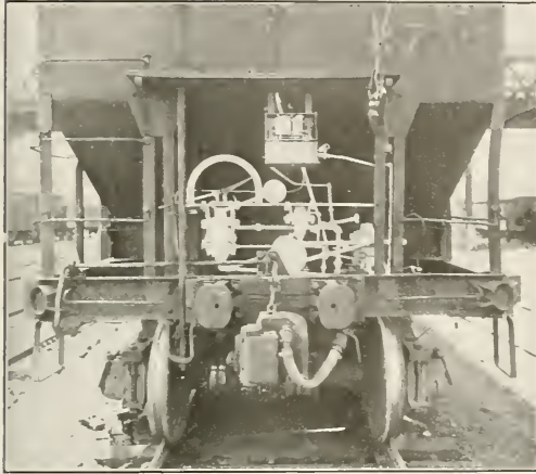
The Rear End of the One-Hundredth Car, Showing the A. S. A. Brake Equipment and the Trainagraph
