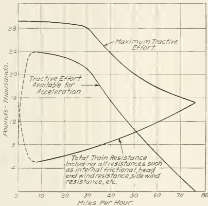
Fig. 1—Train Resistance and Tractive Effort Curves
