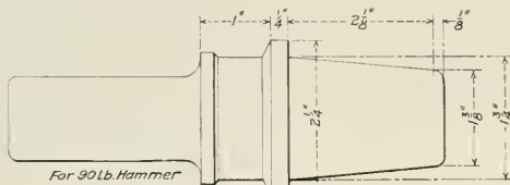
Combination Mandrel and Driver. For 2" Flues. Front End.
