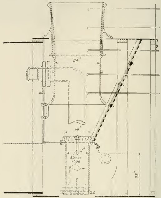
Fig. 2—Front End Arrangement of the N. & W. Mountain Type Locomotives Developed as the Result of the Drafting Tests
