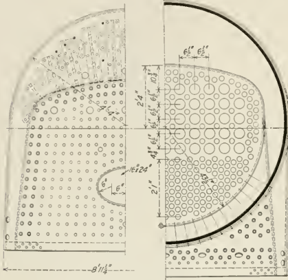
The Back Head and Tube Sheet Layout
