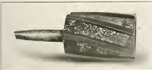
Fig. 1—A Helical Reamer Made of Thermit Steel and High Speed Blades
