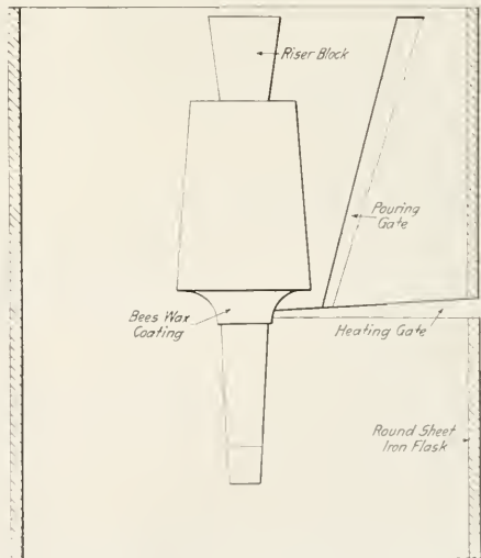
Fig. 3—Set Up of Mould Before Pouring
