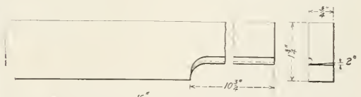
Fig. 10—The Facing Tool
