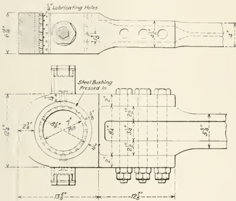
Fig. 1—Detail of Solid Butt End Arrangement
