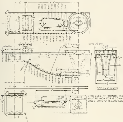
Fig. 12—Bolster "H" Under 150,000 Lb. Combined Load
