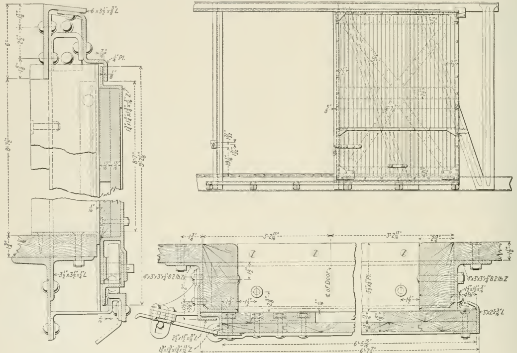
Fig. 7—Box Car Door for the United States Standard Cars
