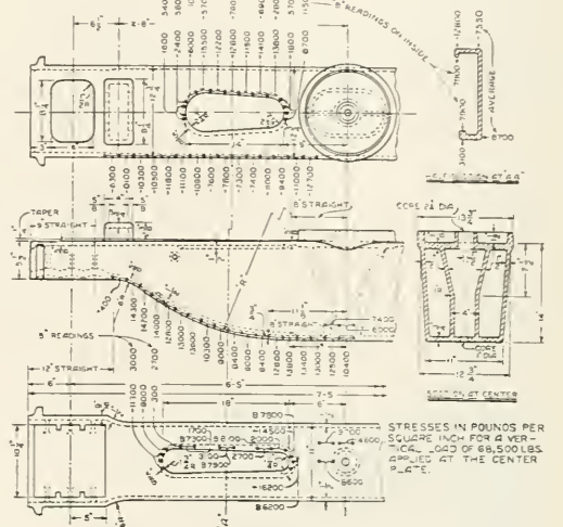
Fig. 14—Bolster "H" Under 68,500 Lb. Load at Center Plate
