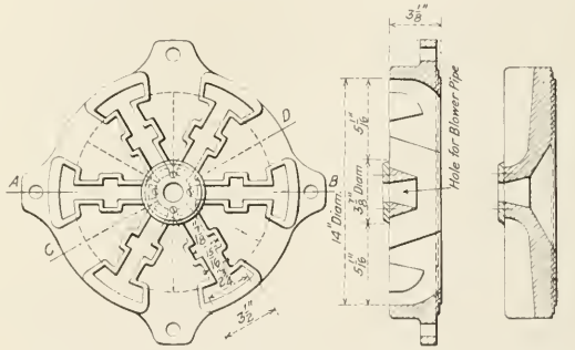
Area = 44.32 sq. in. (Approx. Equiv. to 7½ Diam. Circle) Section A-B. Section C-D.
