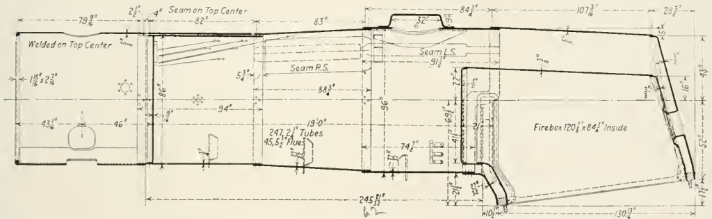
The Boiler for the U. S. Heavy Mikado Type Locomotive.
