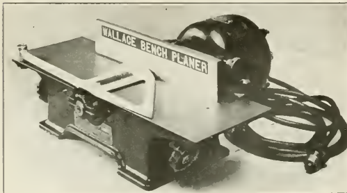
A Portable Wood Planer
