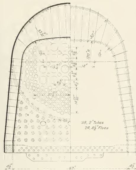
Sections Through Six-Wheel Switch Locomotive
