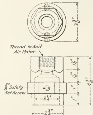
Socket Used with Air Motor for Removing Boiler Tubes
