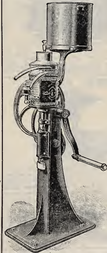
Improved "Baby" No. 1.
