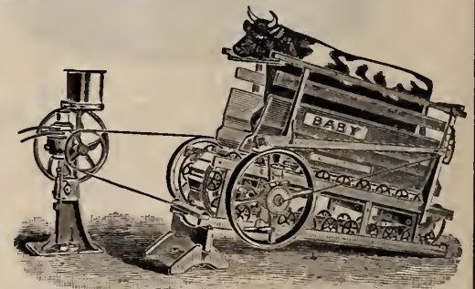
BABY POWER, for Running Cream Separators.
