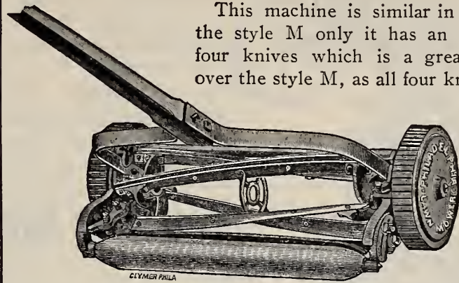
STYLE S. 4-KNIFE. OPEN WIPER. 7 IN. WHEEL.
