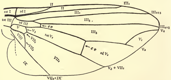
FIG. 580.—Wing of Platypeza .
