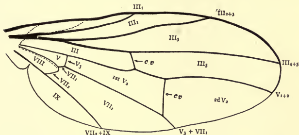
FIG. 591.—Wing of Callophistria annulipes .
