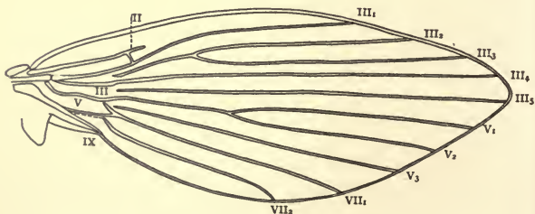
FIG. 500.—Wing of a moth-like fly.
