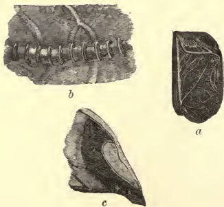
FIG. 133.—Tegmina of male Gryllus .
