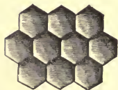
FIG. 72.—Part of compound eye, greatly enlarged.
