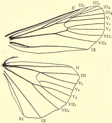
FIG. 350.—Wings of Agrotis ypsilon .
