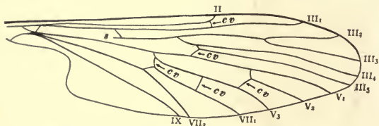
FIG. 504.—Wing of Protoplasma fitchii . (After Osten Sacken.)
