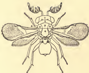
FIG. 738.—A Chalcis-fly: 1, pronotum; 2, 3, 2, mesoscutum; 5, tegula.
