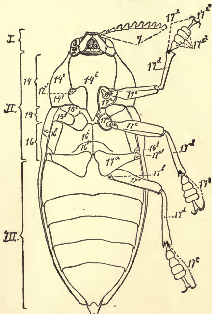
FIG. 611.—Ventral aspect of a beetle, Enchroma gigantea : I, head; 2 c , gena of the epicranium; 3, eye; 7, antenna; II, thorax; 14, prothorax; 14 o , proepisternum or episternum of the prothorax; 14 f , proepimeron or epimeron of the prothorax; 14 i , prosternum; 15, mesothorax; 15 o , mesoepisternum; 15 f , mesoepimeron; 15 i , mesosternum; 16, metathorax; 16 o , metaepisternum; 16 f , metaepimeron; 16 i , metasternum; 16 h , antcoxal piece of the metasternum; 17 o , coxa; 17 h , trochantin; 17 b , trochanter; 17 e , femur; 17 d , tibia; 17 o , tarsus; 17 o1 , tarsal claws; 17 o2 , pulvilli; 18, elytron.
