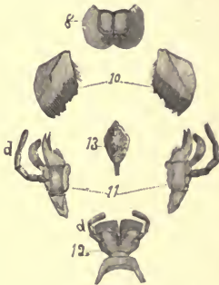
FIG. 75.—Mouth-parts of the Red-legged Locust.
