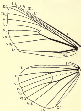
FIG. 379.—Wings of Copidryas gloveri .
