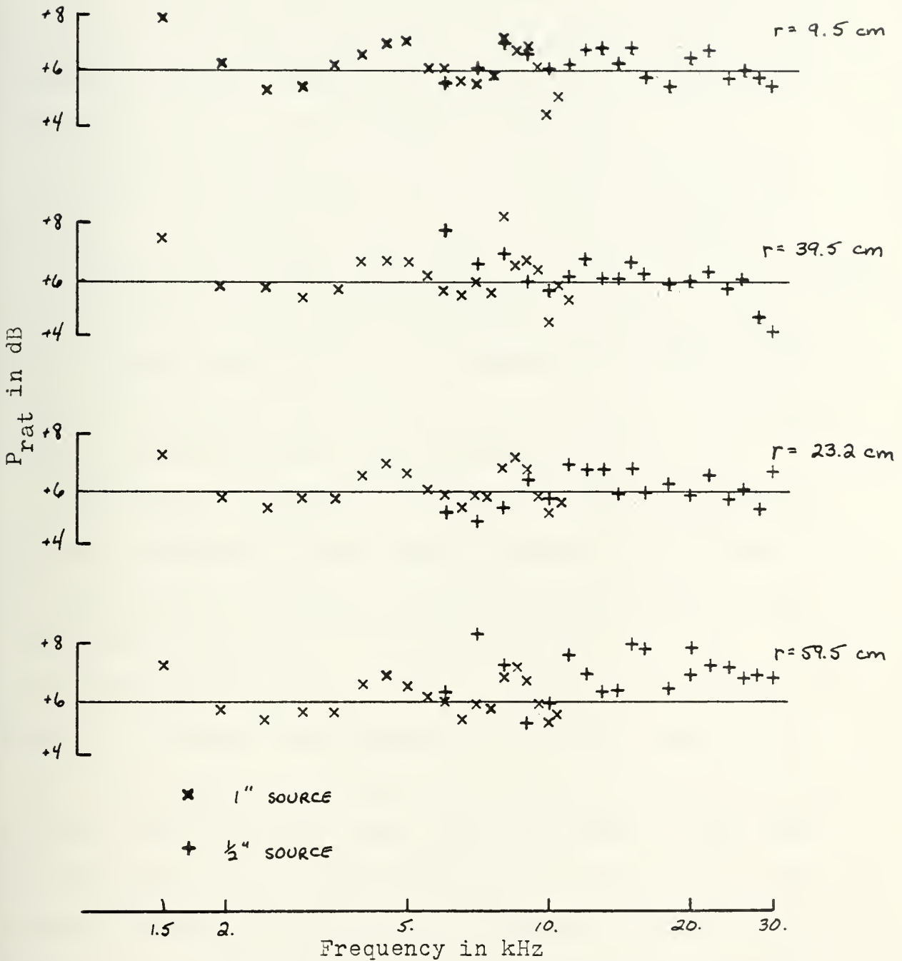
Figure 28. Comparison of P_{rad} as a Function of Frequency at Various Distances ( r ) for the 10 cm Strip (Geometry of Fig. 27).
