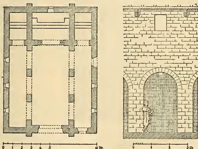
Fig. 225.—Plan and System of S. Adrian in Tufion.
