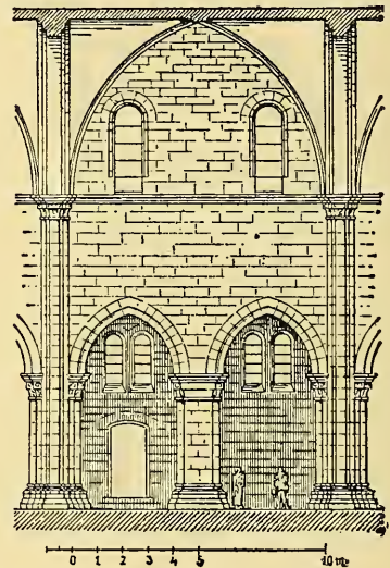
Fig. 336.—System of the Cathedral of Naumburg.
