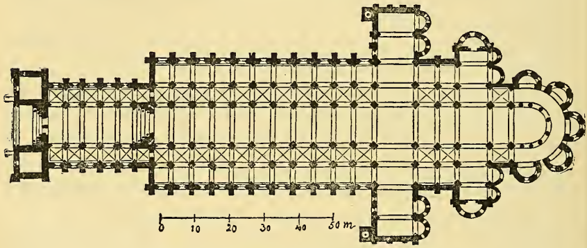
Fig. 212.—Plan of the Abbey Church of Cluny.
