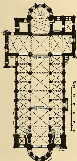
Fig. 333.—Plan of the Cathedral of Bamberg.
