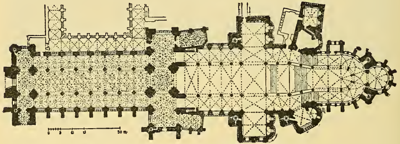
Fig. 324.—Plan of the Cathedral of Canterbury.
