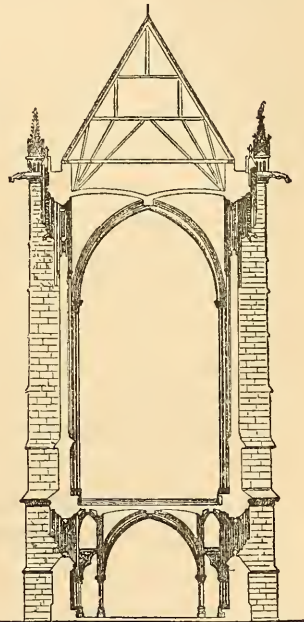
Fig. 305. —Section of the Sainte Chapelle, Paris.
