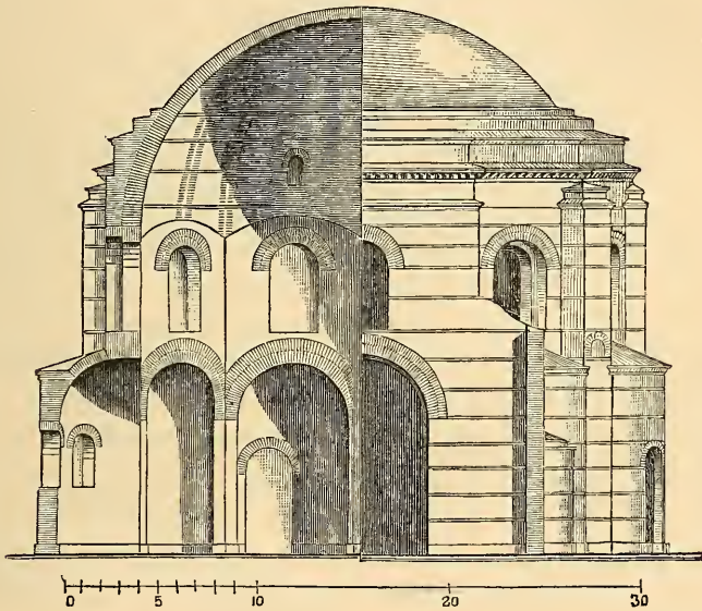
Fig. 21.—So-called Temple of Minerva Medica.
