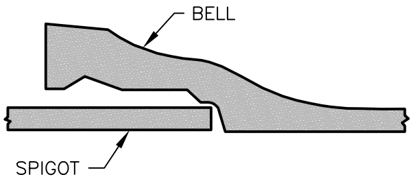
UNFINISHED JOINT
