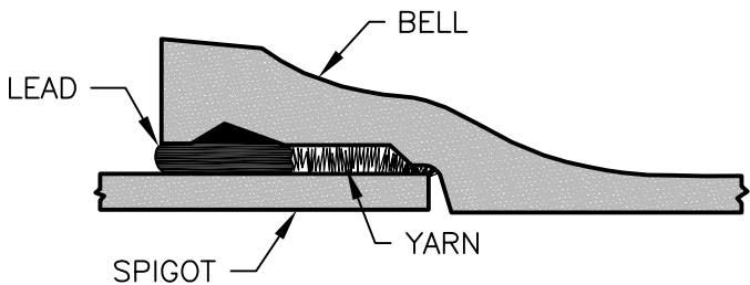
COMPLETED JOINT
