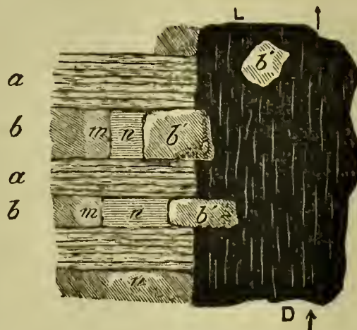
FIG. 8.—Projection of blocks from the permeable Strata b into the ascending lava (one side only is represented).
