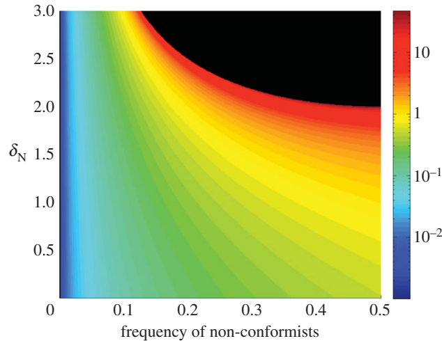
Figure 3. Convergence positions for a minority of non-conformists. Initial positions were zero for conformists and 1 for non-conformists. The colour map is on a log scale and indicates the limiting equilibrium position. That is, the colour indicates the point towards which the conformists and non-conformists converge. The black area indicates values for which the system diverges.
