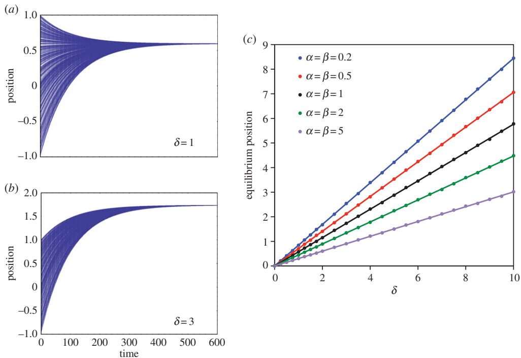
Figure 1. The system converges on a single value when all individuals share the same preferred distinctiveness. We first illustrate example trajectories for (a) \delta = 1 and (b) \delta = 3 . (c) Equilibrium positions at convergence limit as a function of \delta for several distributions of initial positions. For these and all other runs, N = 500, k = 0.01 .
