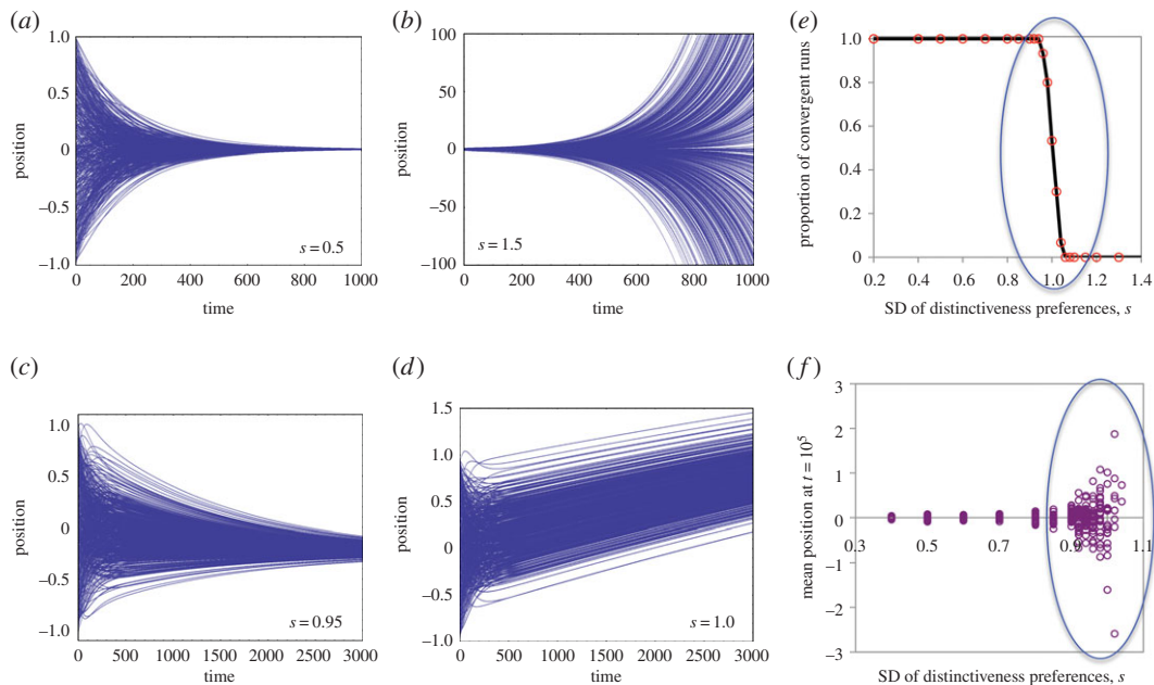
Figure 2. Individual preferences drawn from a normal distribution. (a–d) Example trajectories of runs, with s as indicated. (e) The proportion of simulation runs (of 30) for which the population converged as a function of s . (f) Mean population position for convergent runs as a function of s . This figure omits one outlier at (0.96, -5.46 ).
