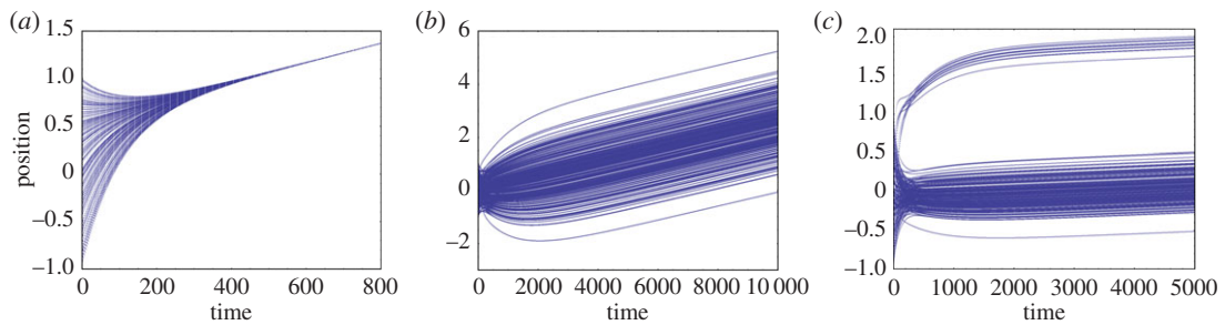
Figure 5. Example trajectory plots for Model 2, patterned after otherwise identical runs for Model 1. (a) Uniform distinctiveness preferences, \delta = 1 . (b) Normally distributed preferences drawn from N(0, 0.9) . (c) Bimodally distributed preferences. 92% conformists' preferences drawn from N(-0.2, 0.3) . 8% non-conformists' preferences drawn from N(3, 0.1) . For all runs, \epsilon = 0.1 .
