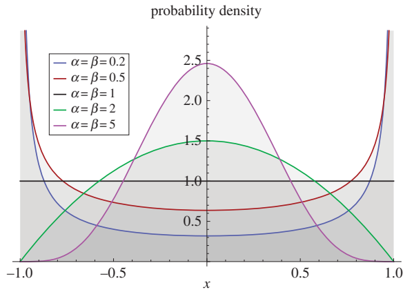
Figure 6. Probability densities of initial distributions of agent positions featured in the main text, figure 1c. Distributions are beta distributions, transformed so that the support is [-1, 1] .
