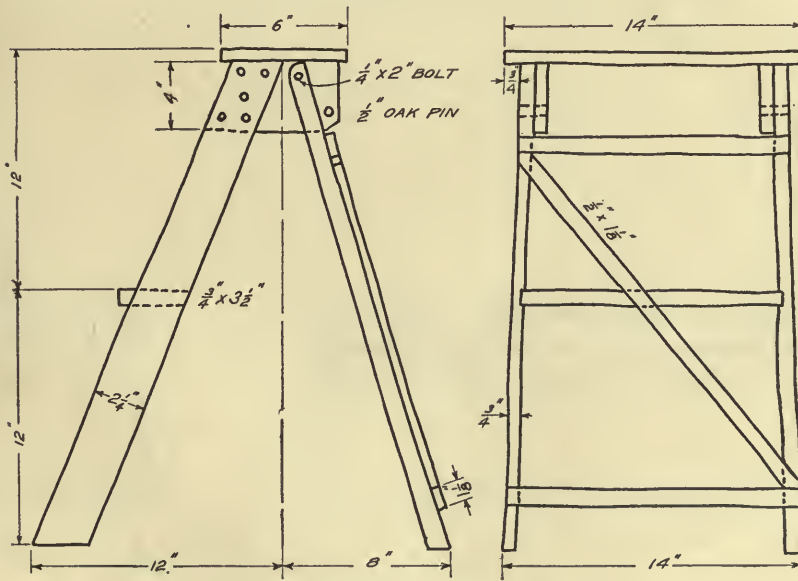
FIG. 178.—Kitchen step-ladder.
