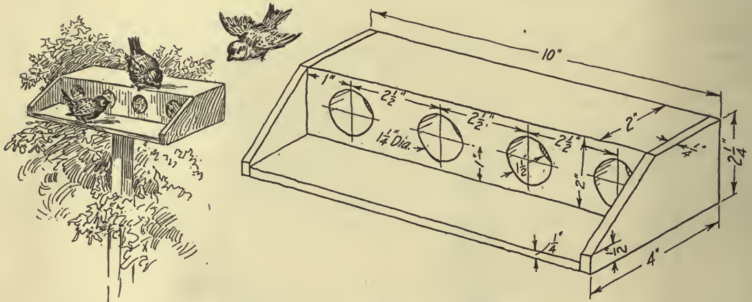
FIG. 34.—Feeding stick for birds.
