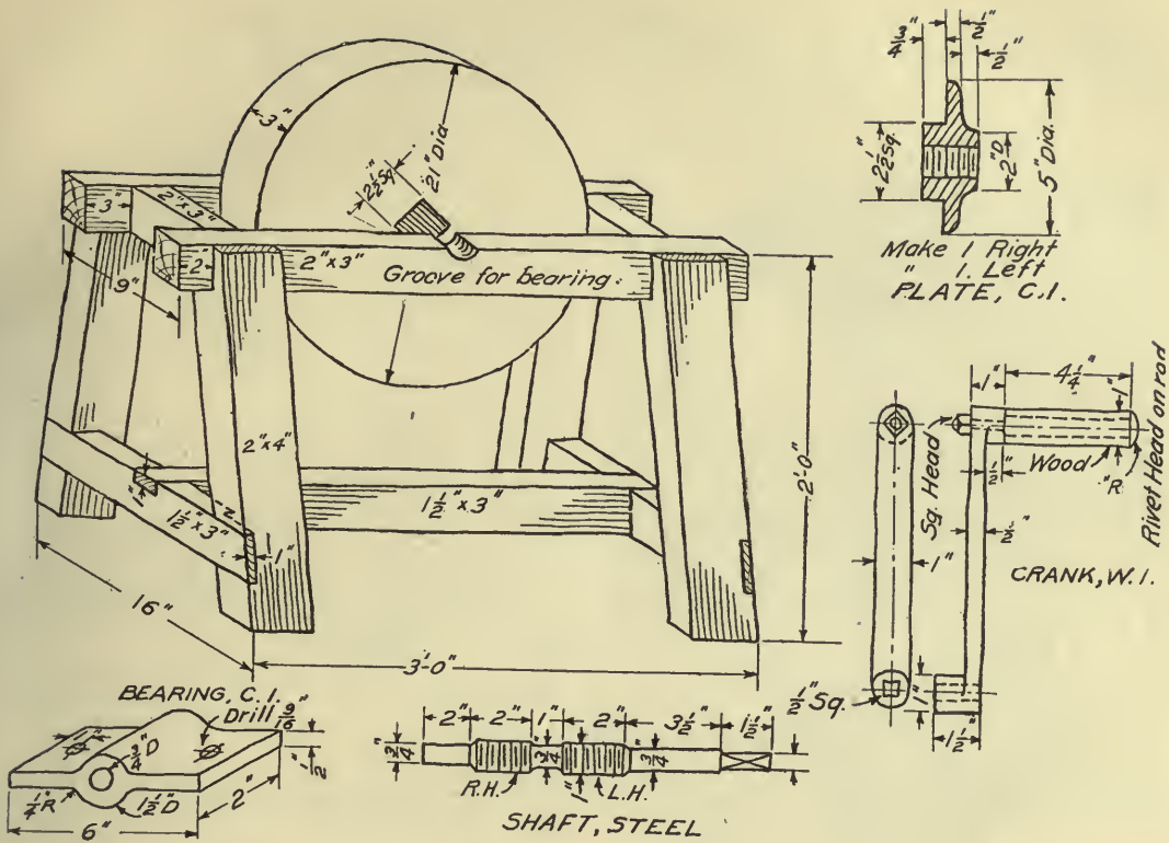
FIG. 89.—Grindstone frame details.
