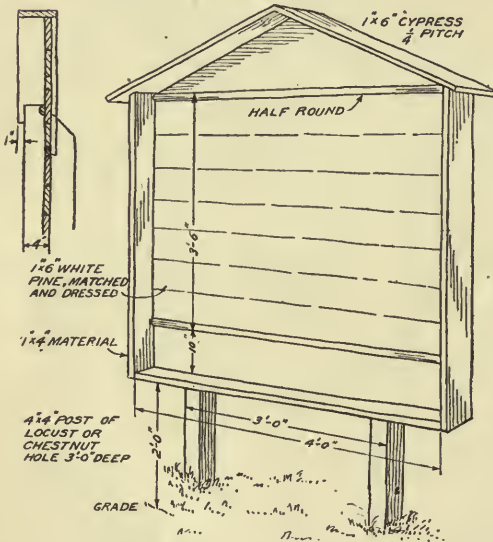
FIG. 86.—Bulletin board.
