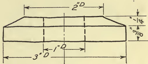
FIG. 163.—Washer.
