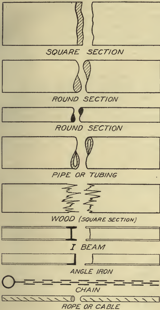
FIG. 56.—Conventional breaks and symbols.
