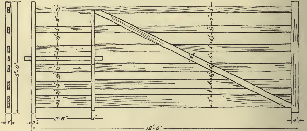
FIG. 88.—Farm gate.
