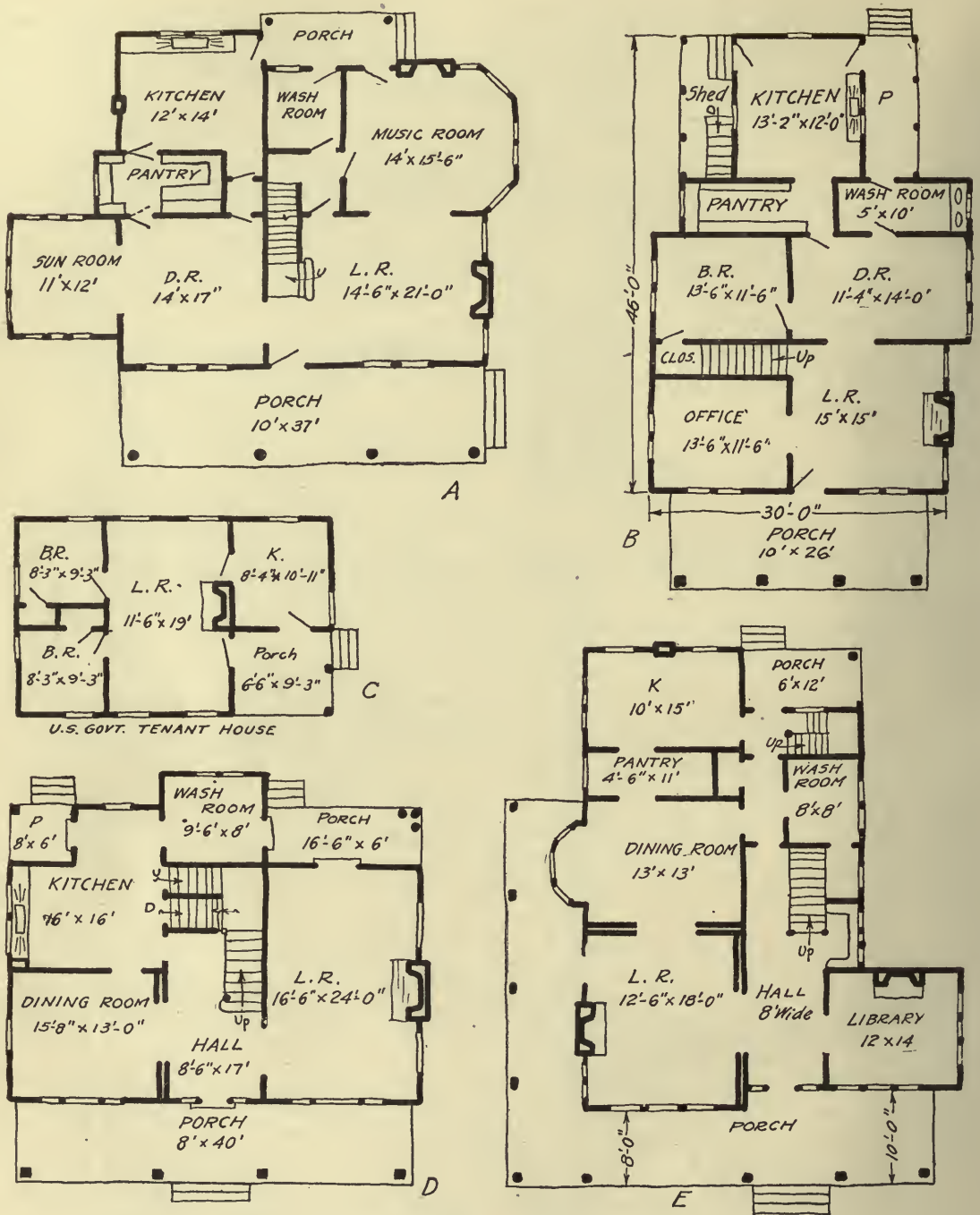
FIG. 137.—Sketch plans of farm houses.
