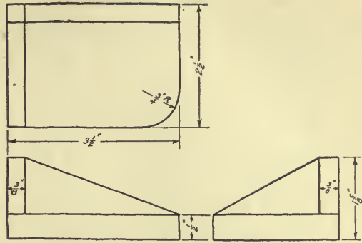
FIG. 162.—Corner plate.
