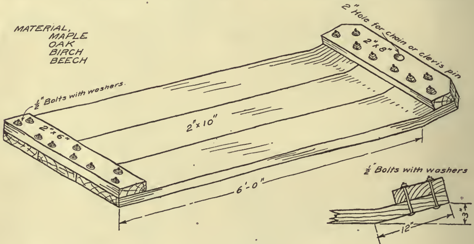
Fig. 81.—Stone boat.
