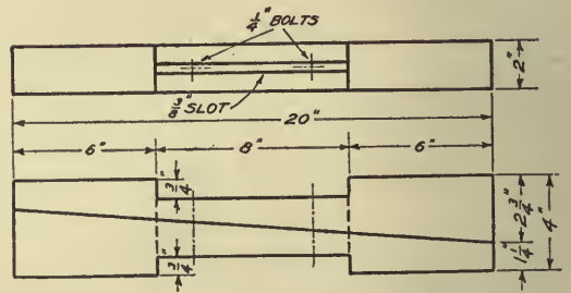
Fig. 169.—Adjustable spacing block.
