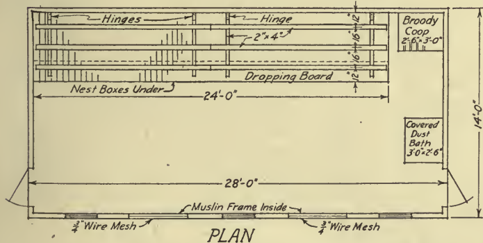
FIG. 123.—Poultry house designed for 100 hens.
