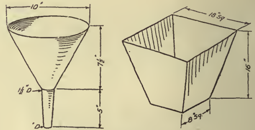
FIG. 95.—Funnel and hopper.
