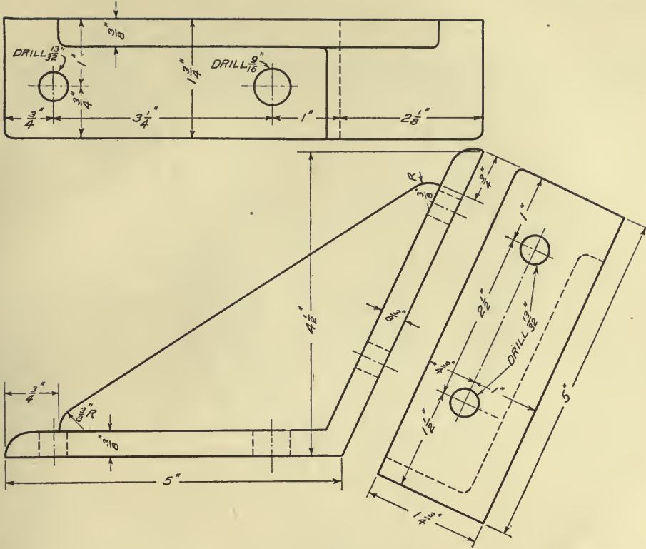
FIG. 177.—Angle brace.
