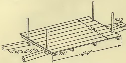
Fig. 80.—Silo rack.
