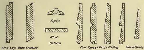
FIG. 103.—Forms of siding.
