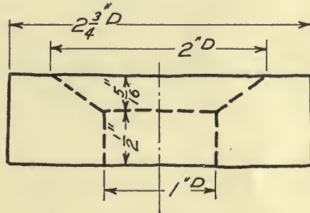
FIG. 164.—Countersunk washer.
