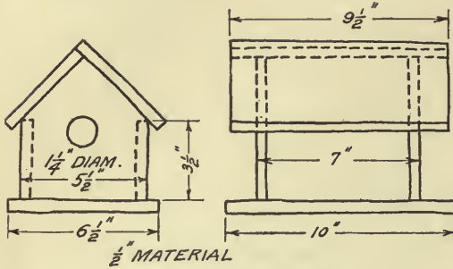
FIG. 174.—Bird house.
