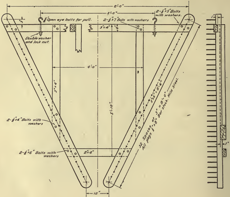
FIG. 179.—Stone rake.
