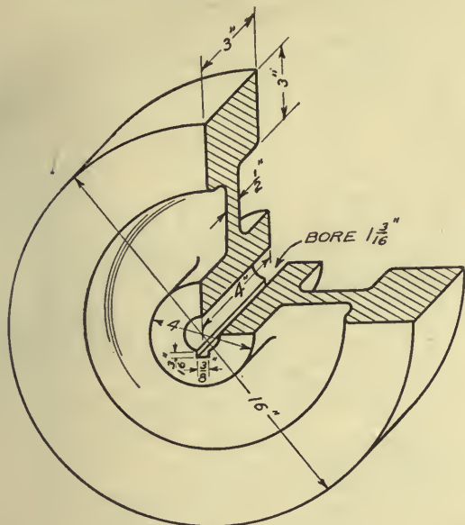
FIG. 83.—Flywheel.
