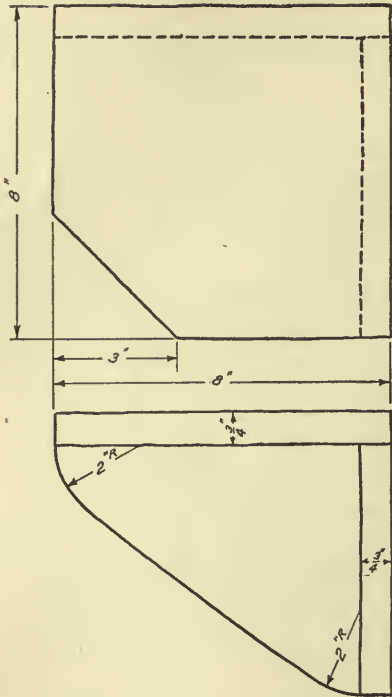
Fig. 166.—Corner bracket.
