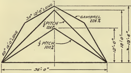
FIG. 100.—Comparative diagram of roof shapes.
