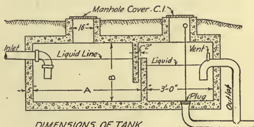
DIMENSIONS OF TANK
