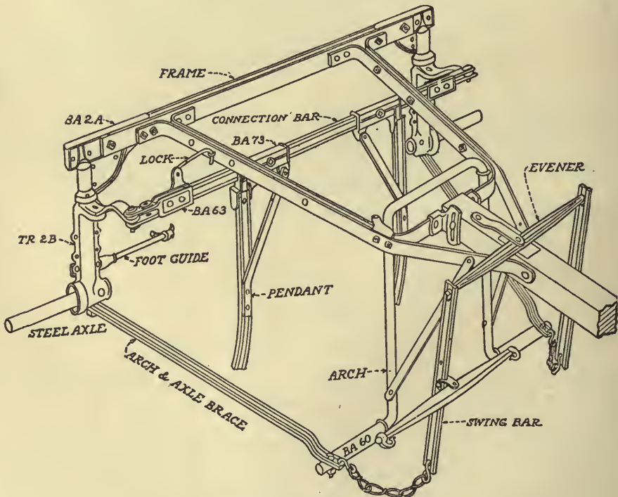
FIG. 3.—An isometric illustration.
