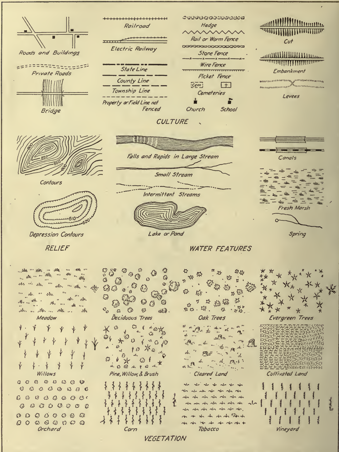
Fig. 142.—Topographic symbols.
