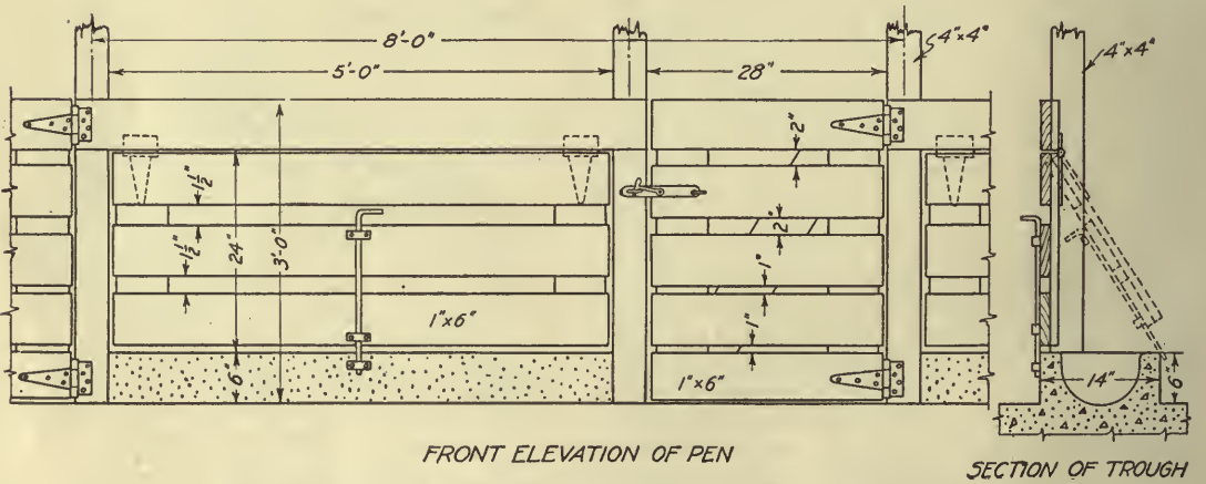
FIG. 121.—Swine house, colony type with half-monitor roof.
