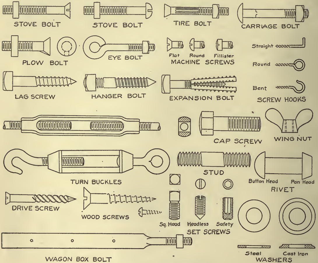
Fig. 62.—Various bolts and screws.
