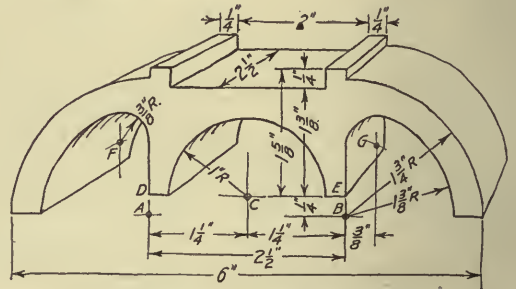
FIG. 39.—Windmill brake shoe.
