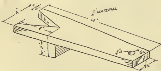
Fig. 82.—Boot jack.
