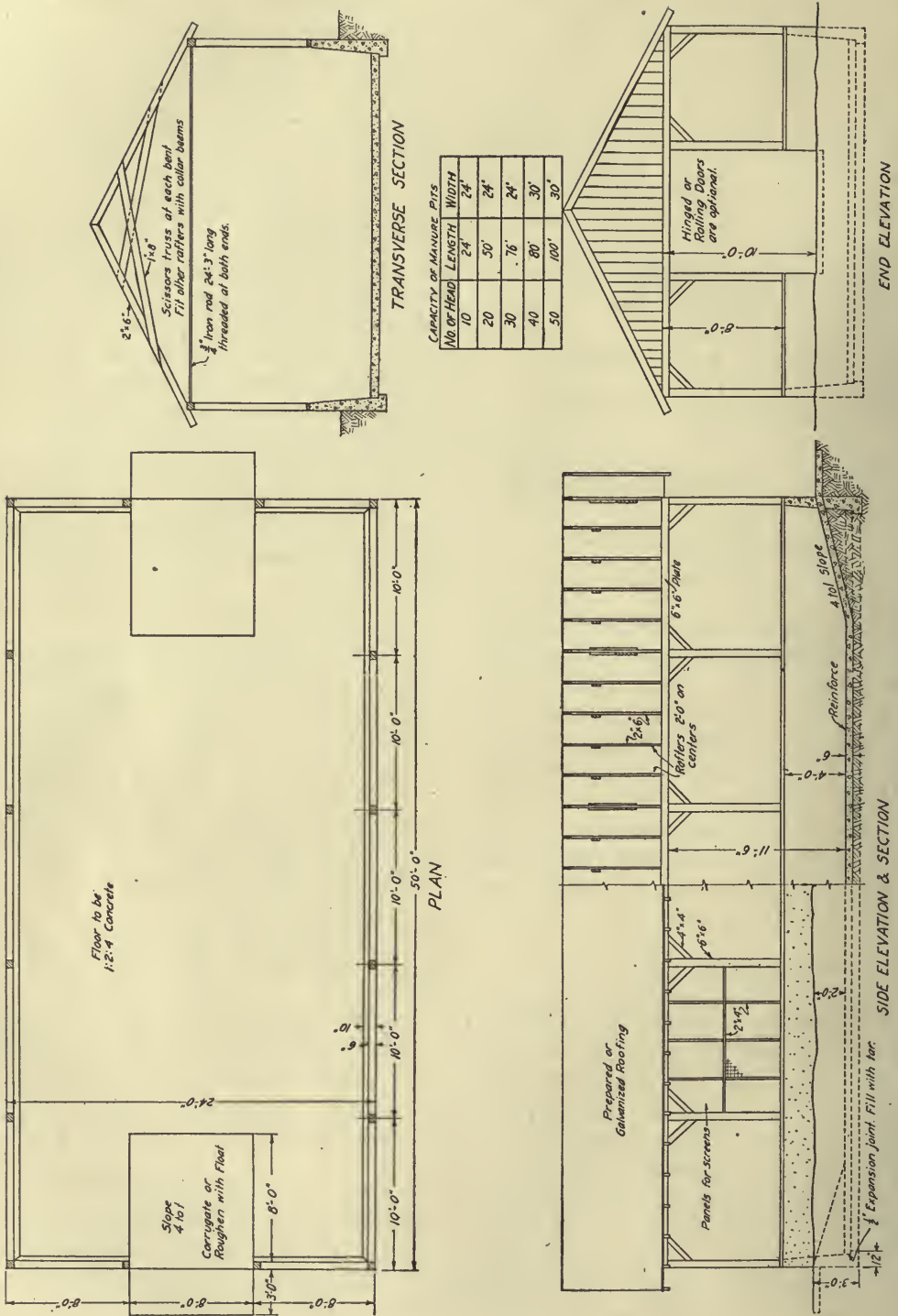
Fig. 132.—Covered manure pit.
