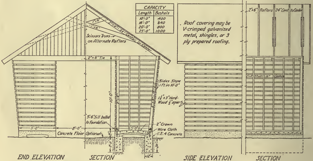
FIG. 126.—Double corn crib, flaring sides, concrete floor.
