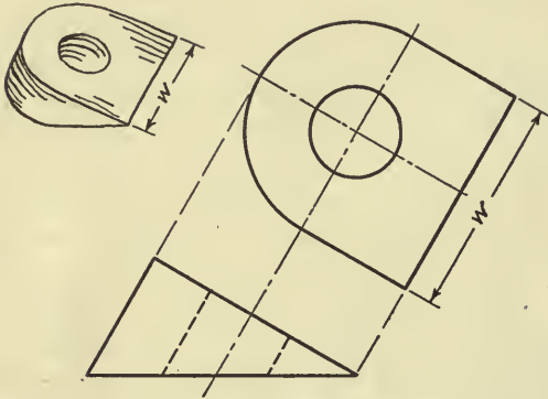
FIG. 51.—An auxiliary view.
