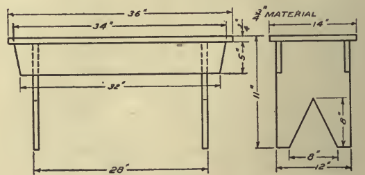
Fig. 170.—Bench.
