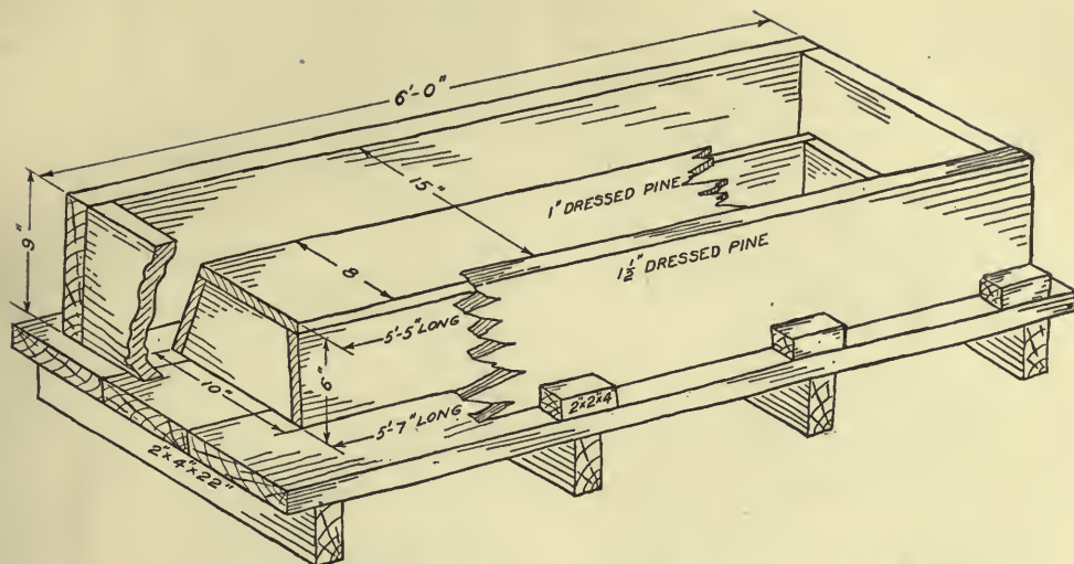
FIG. 78.—Form for concrete trough.
