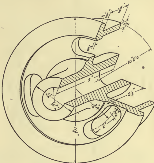
FIG. 84.—Flanged roller.
