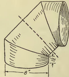
FIG. 93.—Three-piece elbow.
