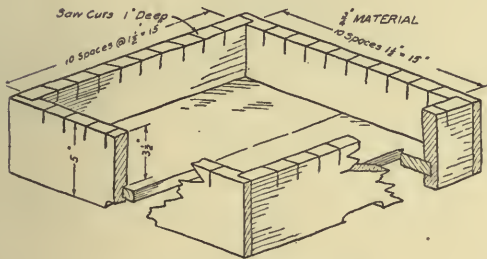
FIG. 71.—Corn tester.
