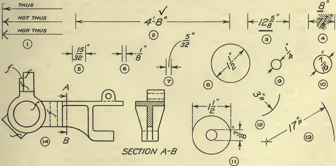
FIG. 54.—Dimensioning.
