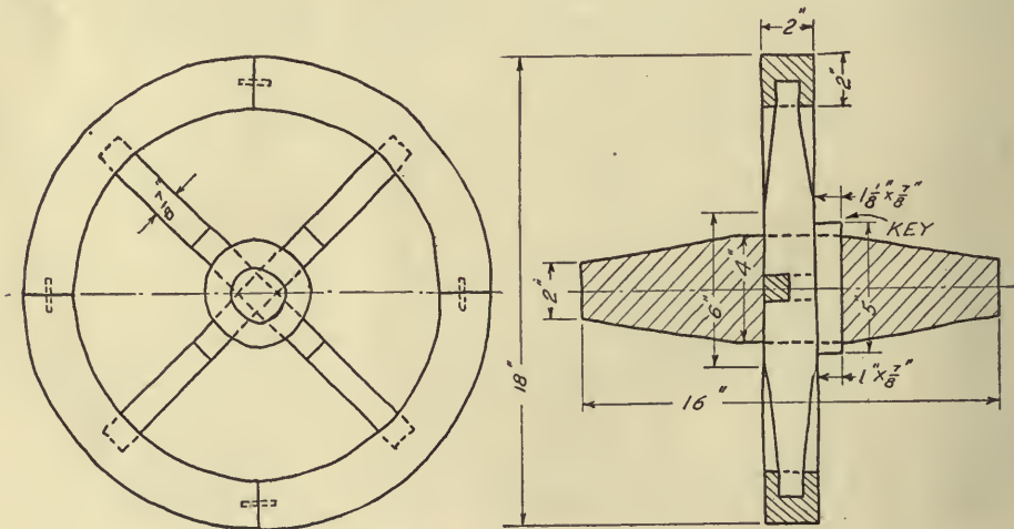
FIG. 176.—Wooden wheelbarrow wheel.
