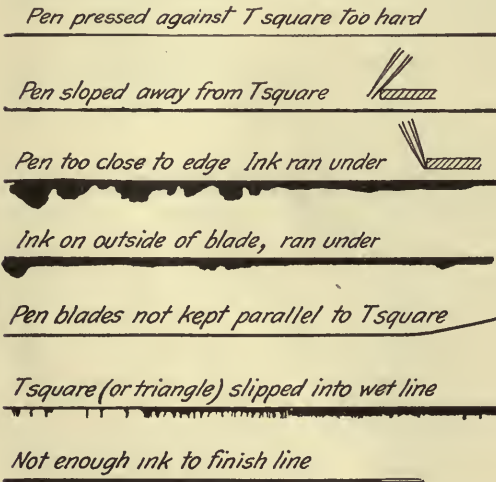
FIG. 38.—Faulty lines.
