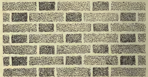
FIG. 106.—Flemish bond.
