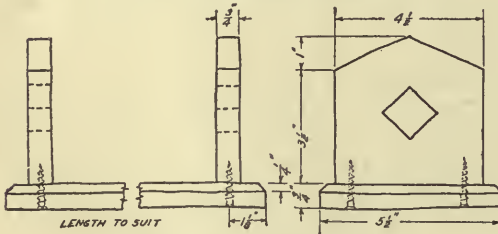
FIG. 175.—Book rack.
