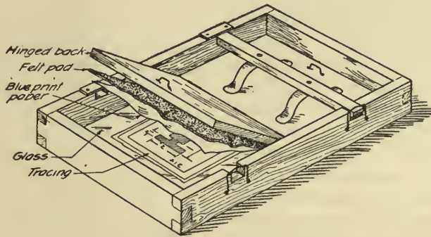
FIG. 182.—Blue-print frame.
