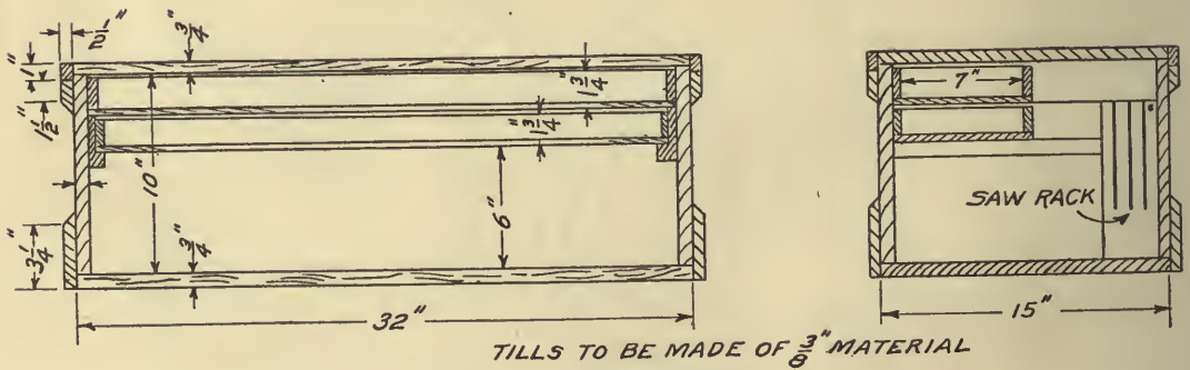
FIG. 180.—Tool chest.
