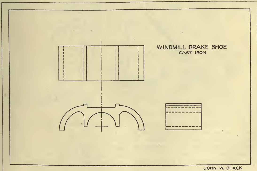
FIG. 41.—Inked drawing.
