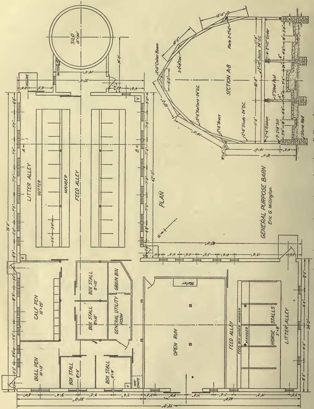
Fig. 117.—General purpose barn, plan and section. Balloon frame.
