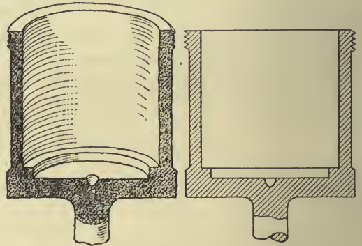
FIG. 48.—Illustration of a section.
