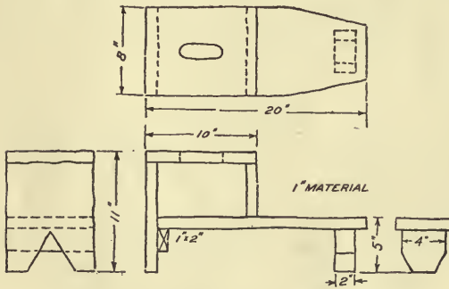
FIG. 75.—Milk stool.
