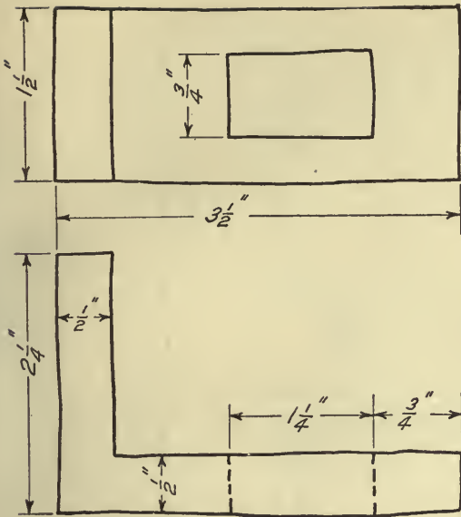
FIG. 159.—Angle stop.
