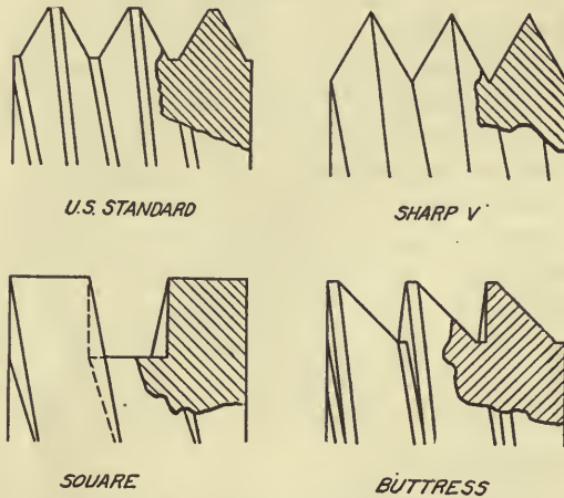
FIG. 57.—Some forms of threads.
