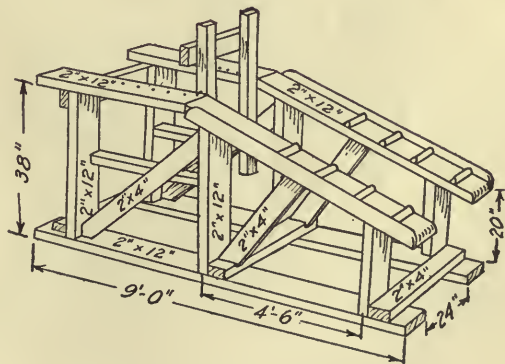
FIG. 91.—Cattle breeding crate.
