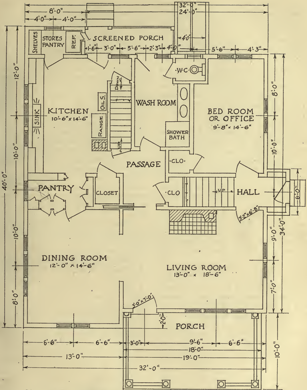
▲ FIRST FLOOR PLAN ▲ • SCALE: 1/8" = 1 FT. •
