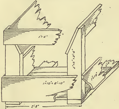
FIG. 74.—Sheep rack.
