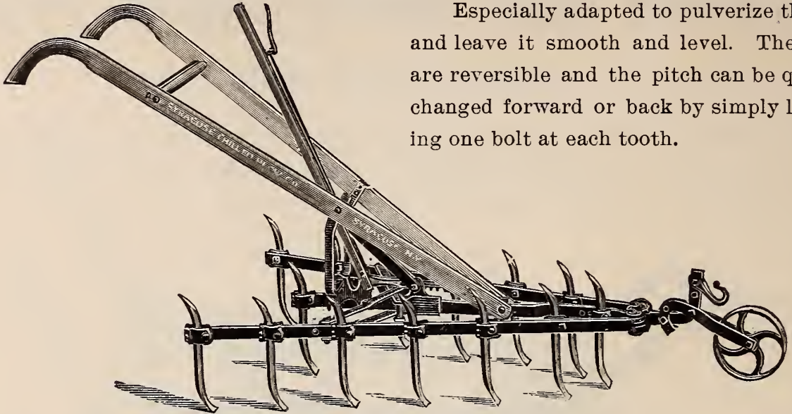
Expanding Lever, fourteen Spike Teeth and Wheel.
