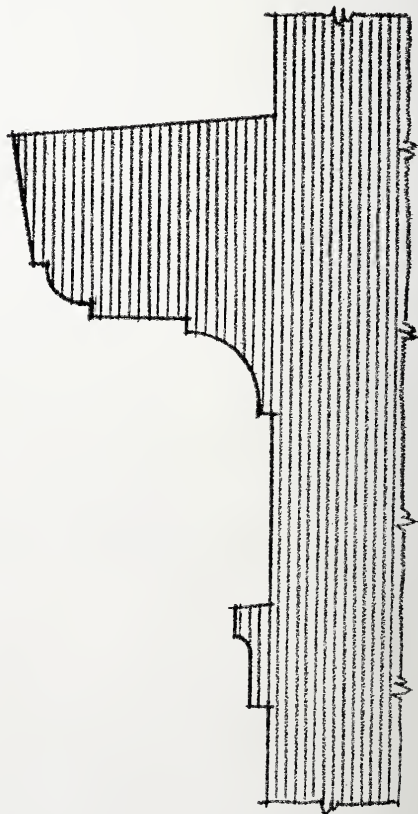
FIG. 8. SUGGESTION FOR CORNICE DETAIL IN CONCRETE.
