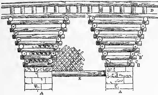
TRACE OF ORIGINAL STRUCTURE IN WOOD, UXMAL.
