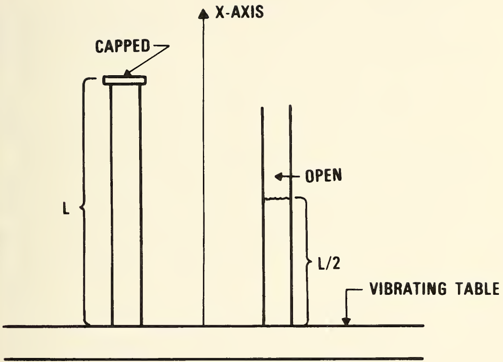
Figure 1a, b: Vibrating cylinders
