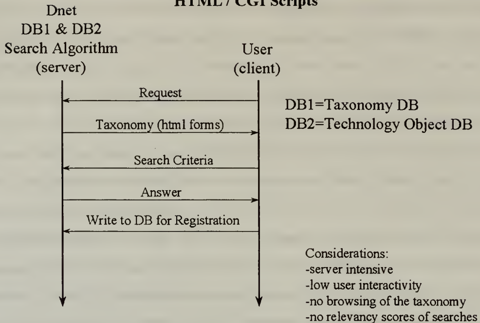
Figure 3. Time Sequence Diagram - Option A
