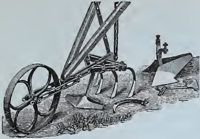
Gem Single Wheel Hoe and Cultivator.
